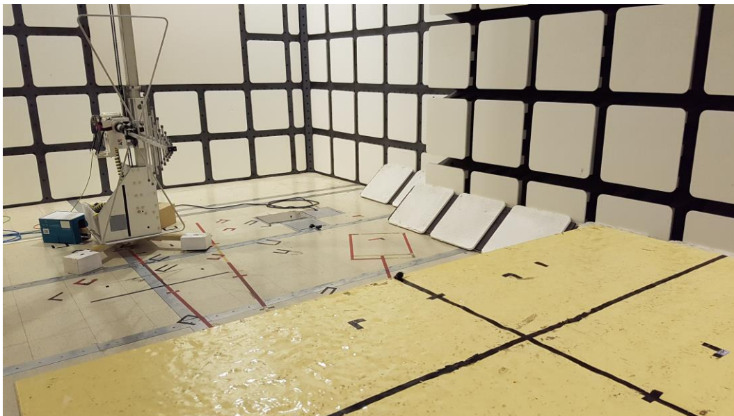
Below 1 GHz _ Rear View
