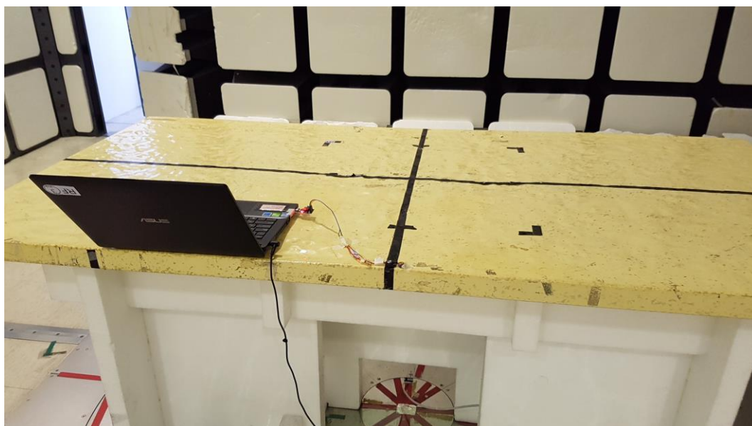
Above 1 GHz _ Rear View
