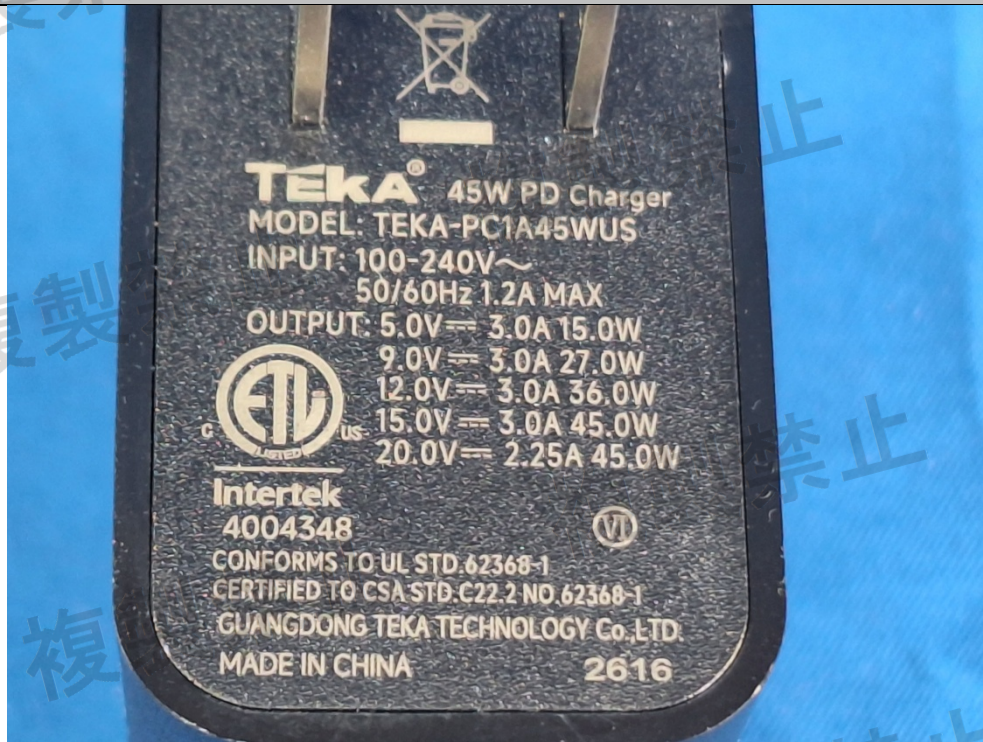
Adapter2 Photo
