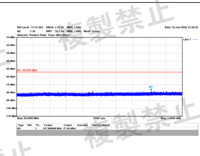
GFSK/4M/2478MHz/Ch38/Ant. 1/1-2 (Nom)
