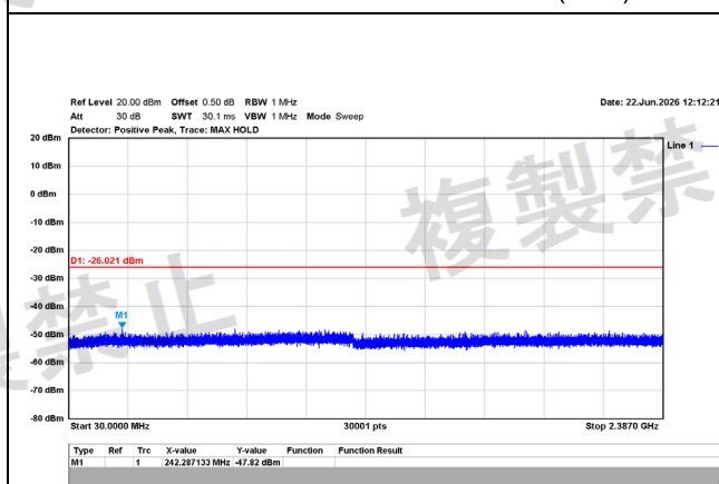
GFSK/4M/2440MHz/Ch19/Ant.1/1-4 (Nom)
