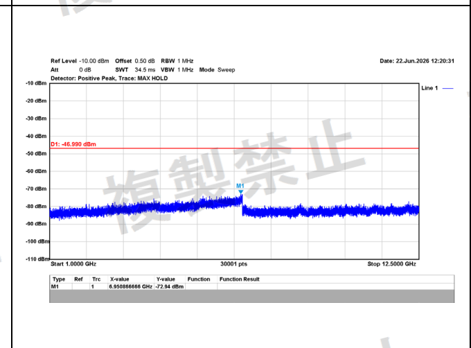
GFSK/4M/2478MHz/Ch38/Ant. 1/2-2 (Nom)
