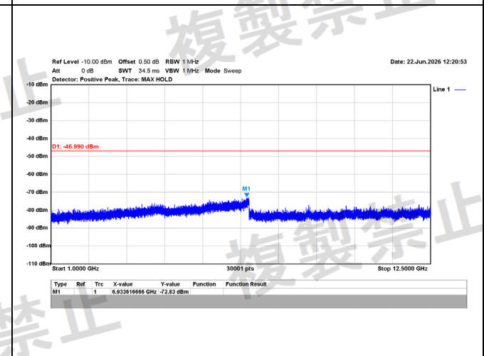
GFSK/4M/2478MHz/Ch38/Ant. 1/2-2 (Nom)
