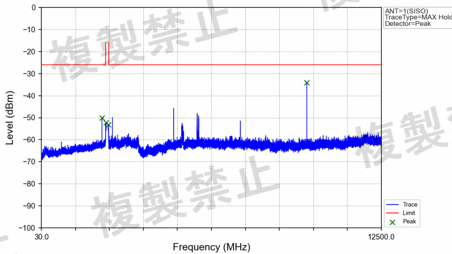
GFSK_DH5_2441MHz_Ant1_NTHV
