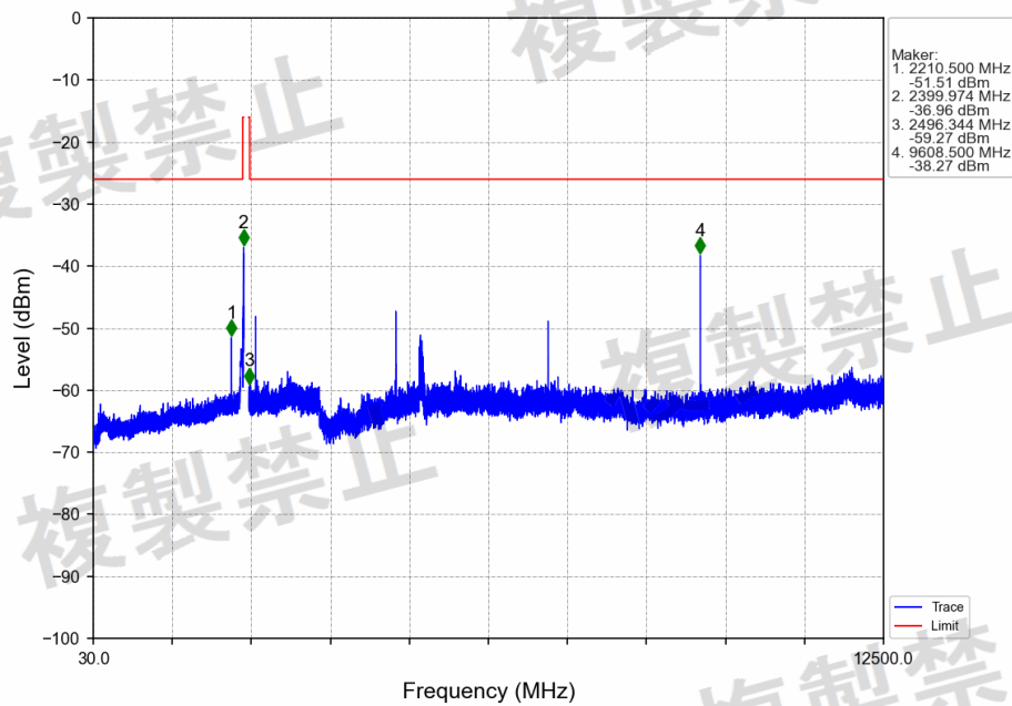
GFSK_DH5_2402MHz_Ant1_NTLV
