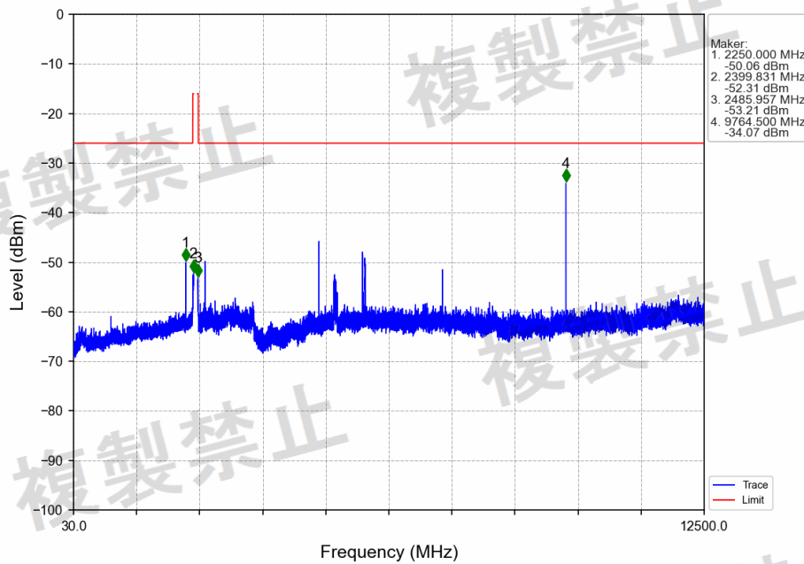
GFSK_DH5_2441MHz_Ant1_NTHV
