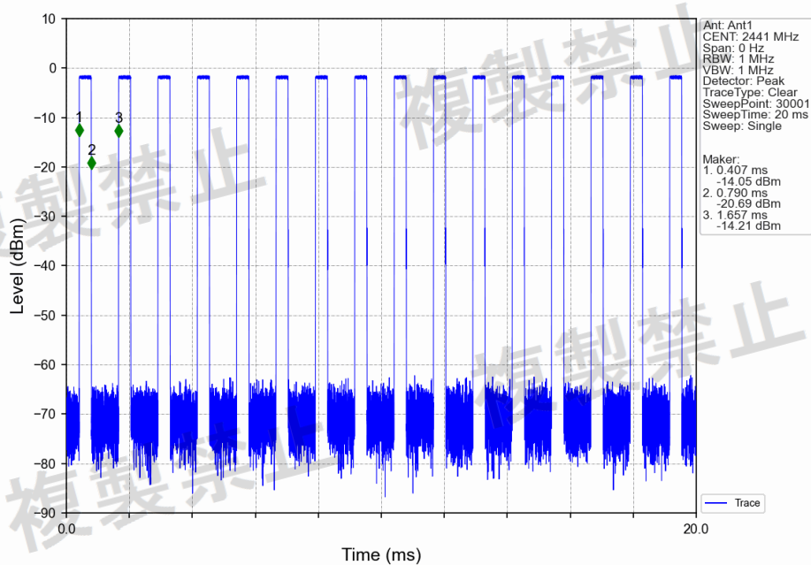
GFSK DH3_2441MHz_Ant1_NTNV
