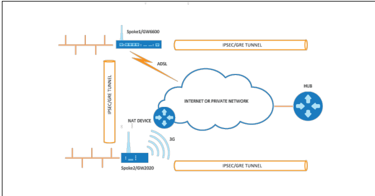
Figure 171: Network diagram for DMVPN spoke behind NAT
