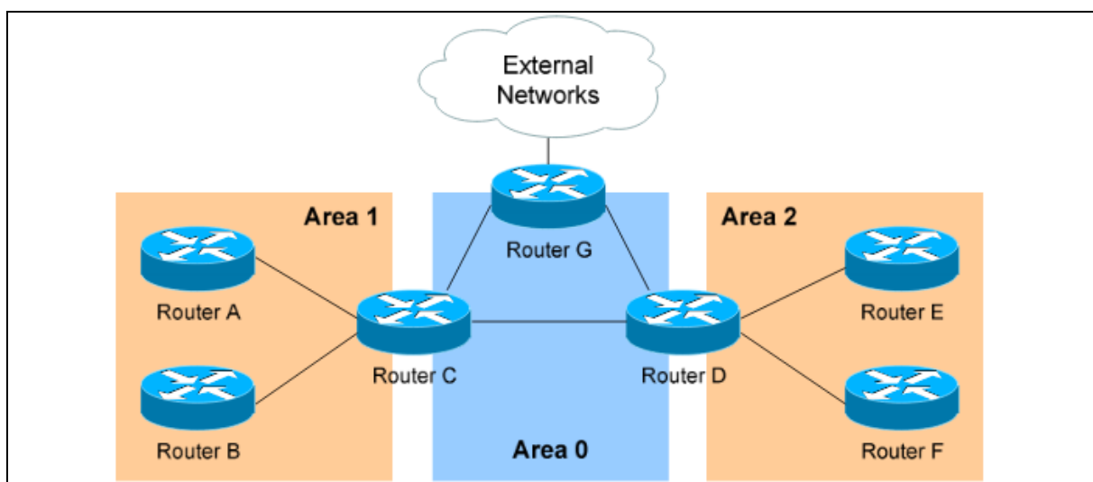
Figure 98: OSPF hierarchy
