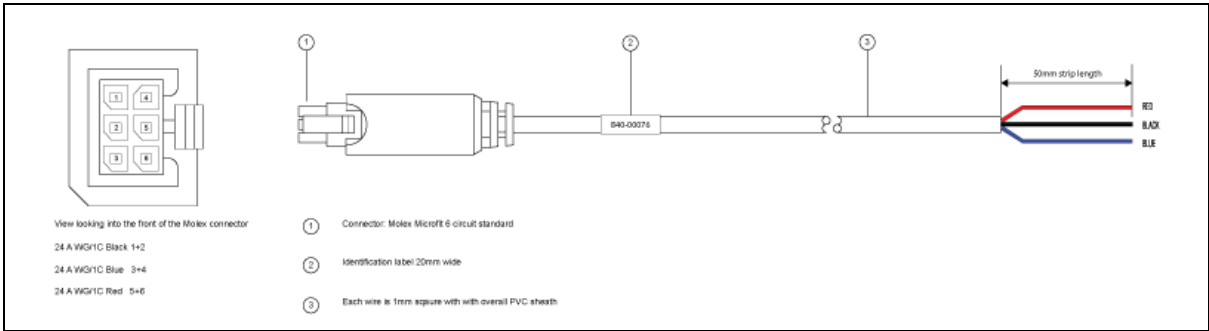
Figure 7: 840-00076 3 core power cable
