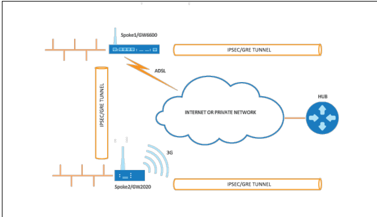
Figure 170: Network diagram for DMVPN spoke to spoke
