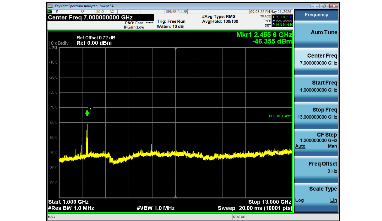
Rx. Spurious NVNT BLE 1M 2440MHz Ant1 @ 1000MHz-13000MHz
