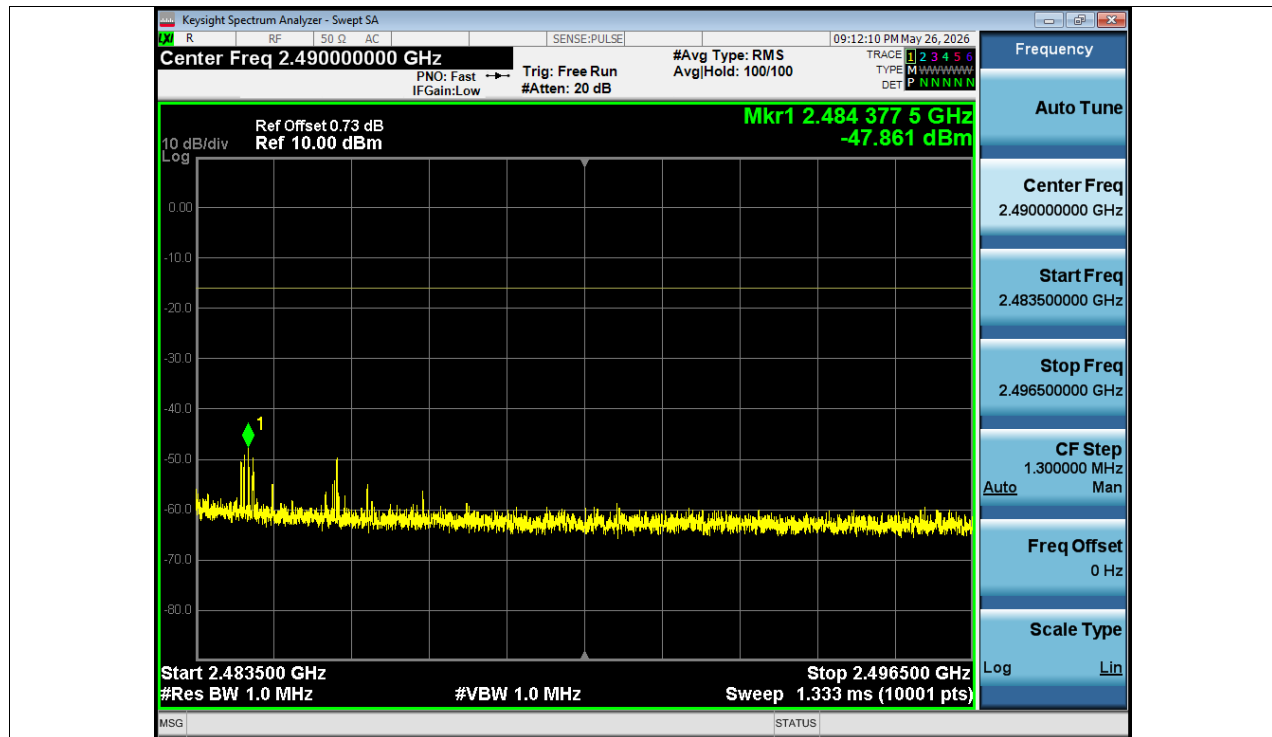
Tx. Spurious NVNT BLE 1M 2480MHz Ant1 @ 2483.5MHz-2496.5MHz
