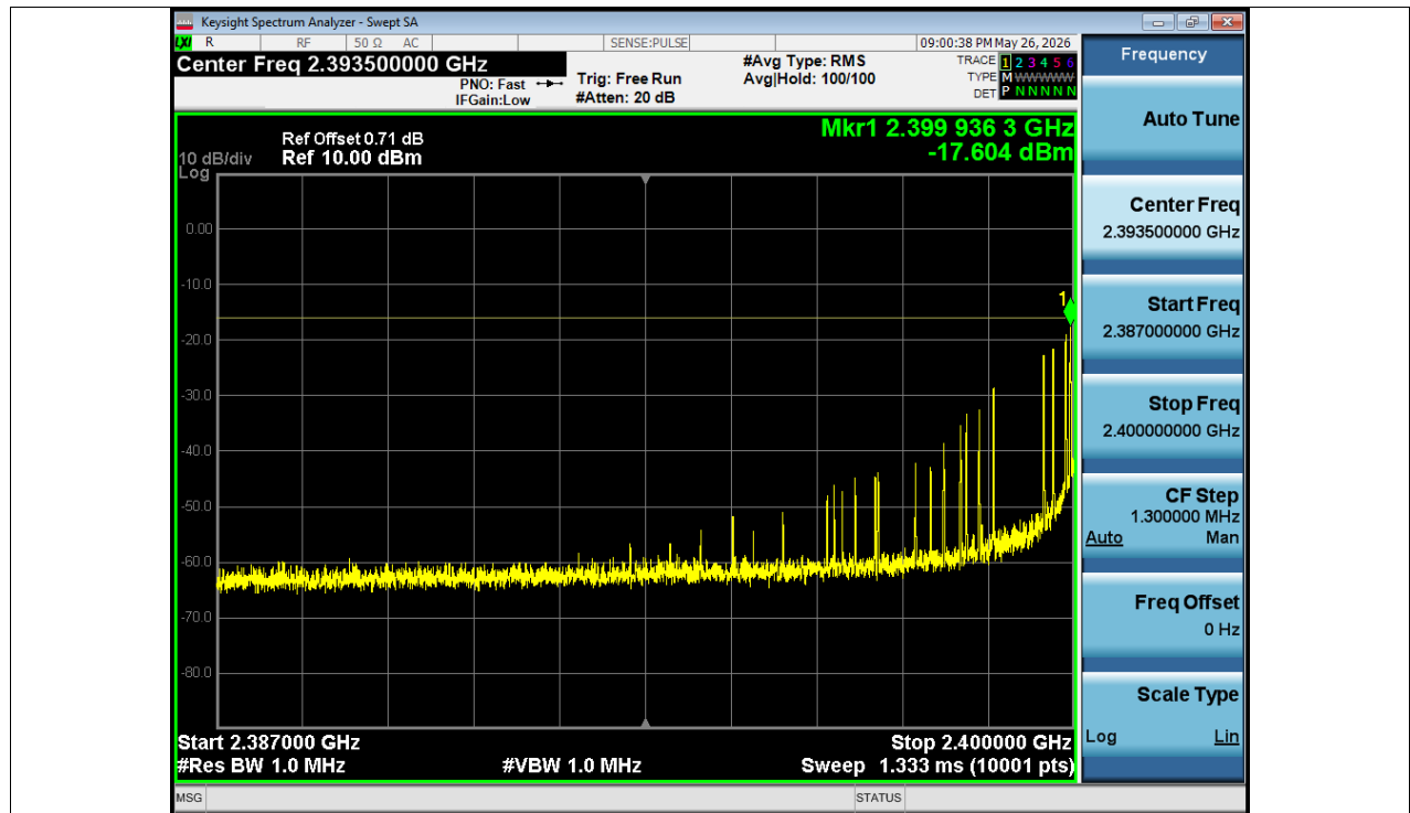
Tx. Spurious NVNT BLE 1M 2402MHz Ant1 @ 2387MHz-2400MHz
