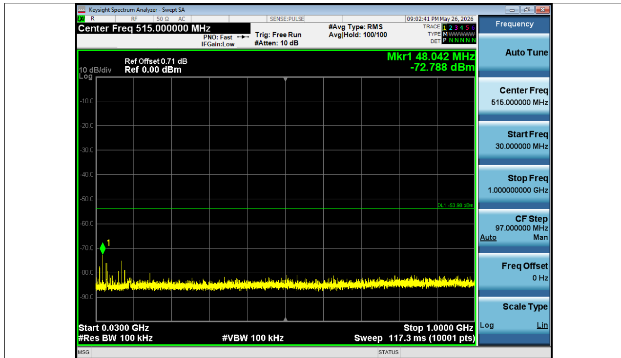
Rx. Spurious NVNT BLE 1M 2402MHz Ant1 @ 30MHz-1000MHz
