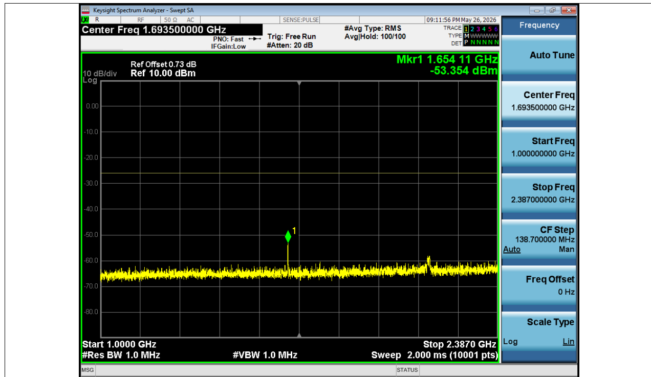
Tx. Spurious NVNT BLE 1M 2480MHz Ant1 @ 1000MHz-2387MHz
