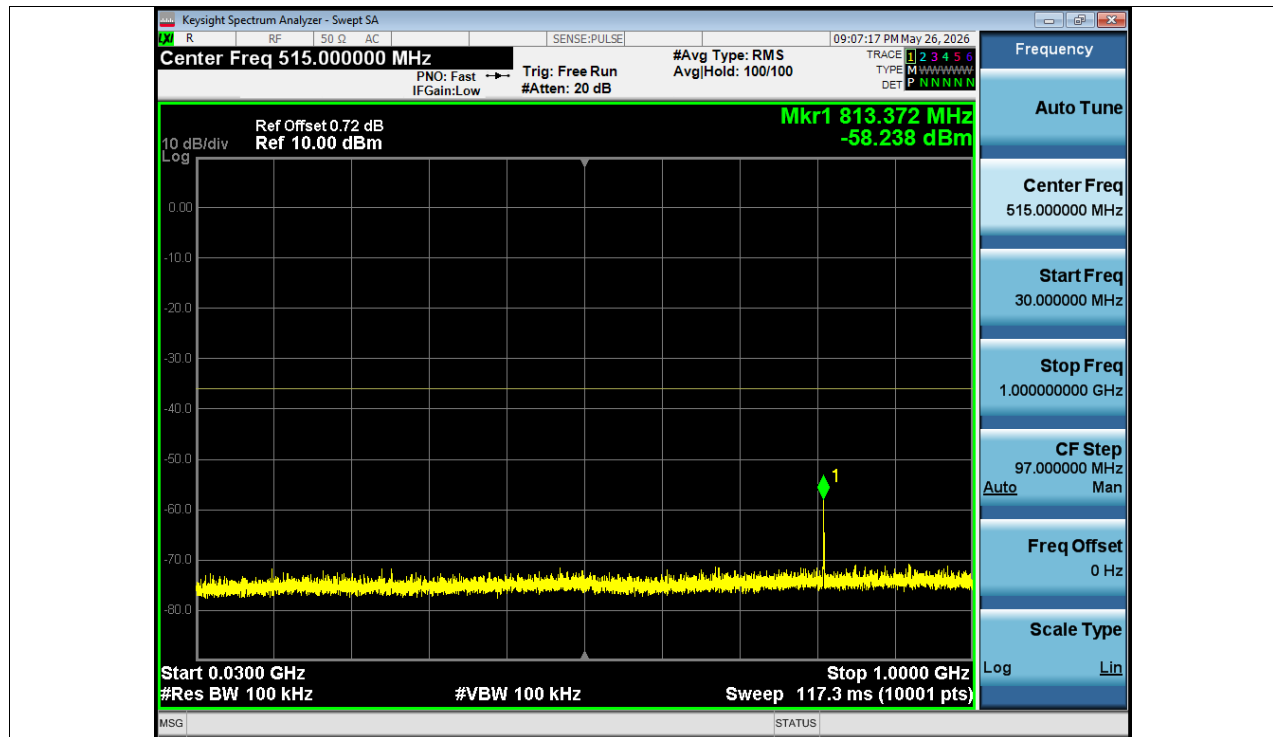
Tx. Spurious NVNT BLE 1M 2440MHz Ant1 @ 30MHz-1000MHz
