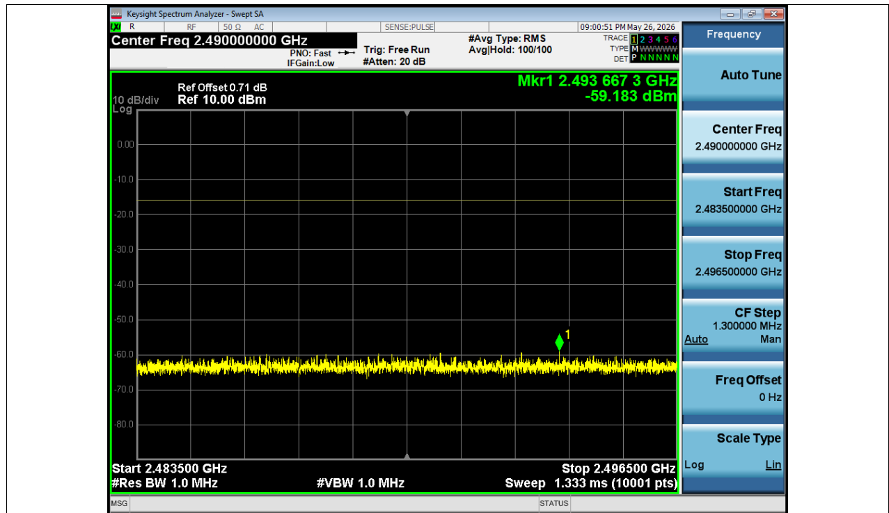
Tx. Spurious NVNT BLE 1M 2402MHz Ant1 @ 2483.5MHz-2496.5MHz
