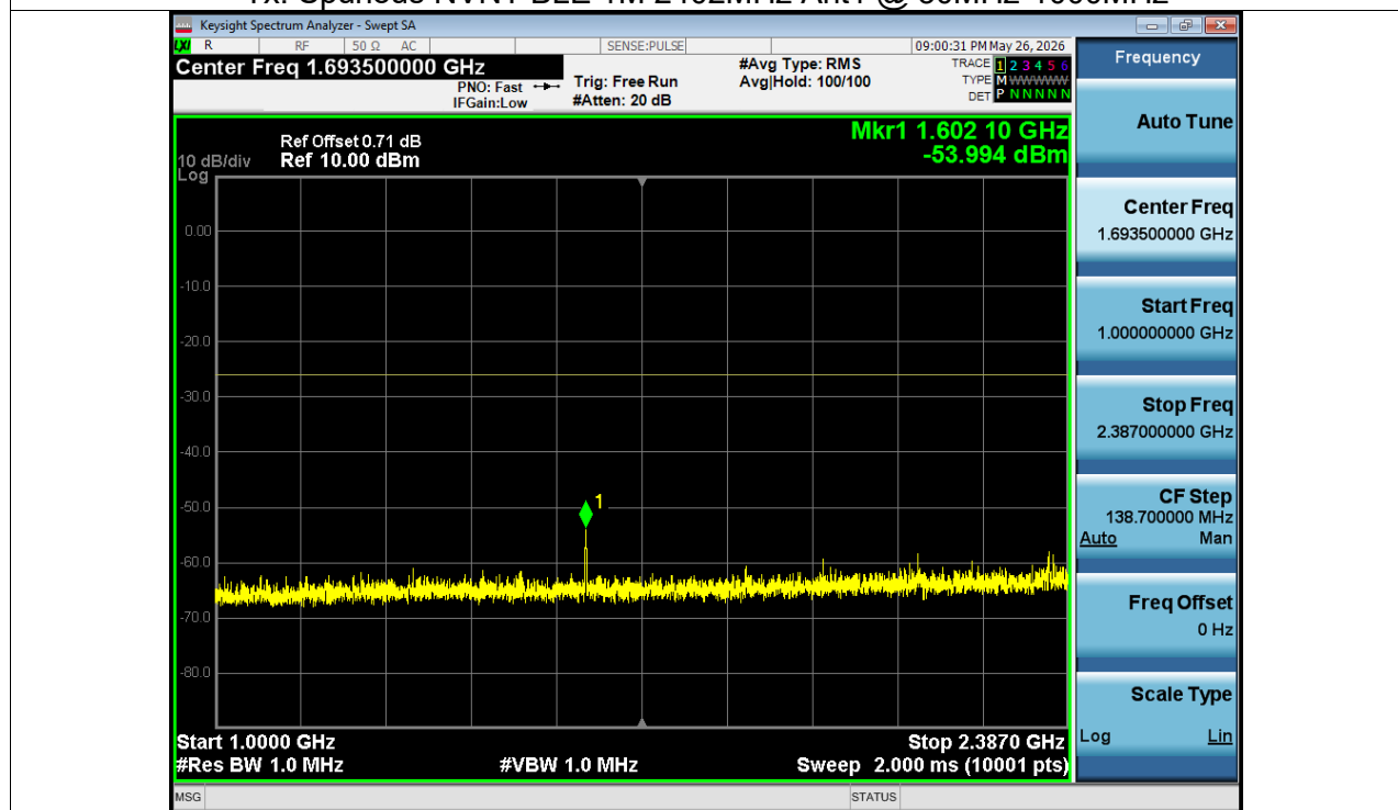
Tx. Spurious NVNT BLE 1M 2402MHz Ant1 @ 1000MHz-2387MHz
