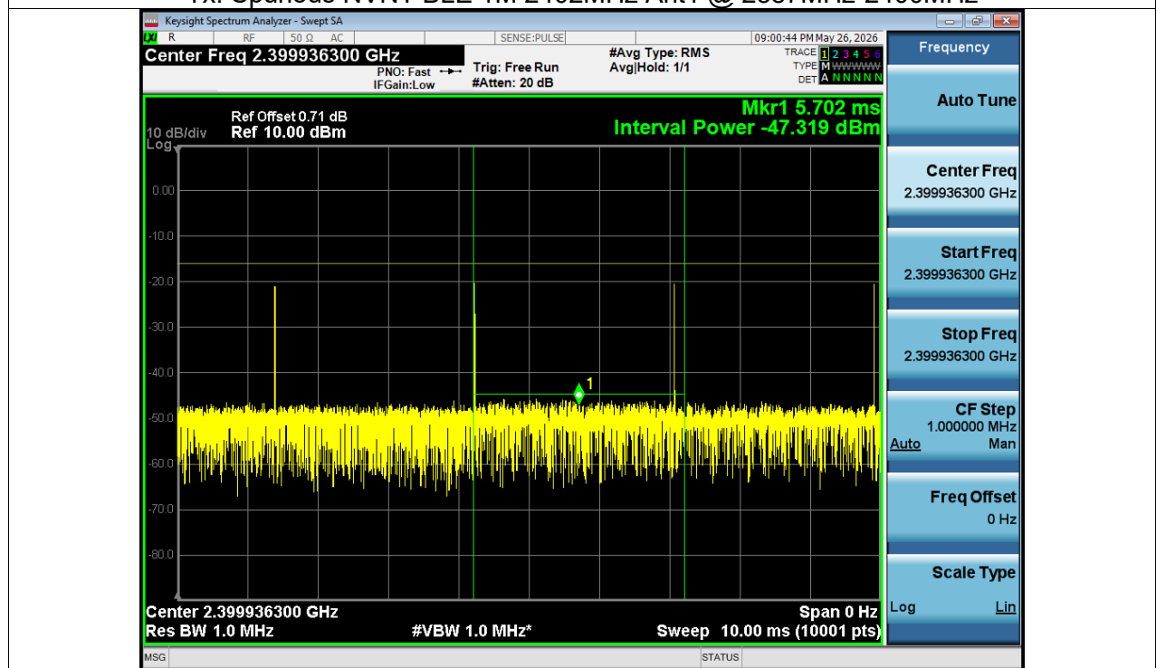
Tx. Spurious NVNT BLE 1M 2402MHz Ant1 @ 2387MHz-2400MHz Final
