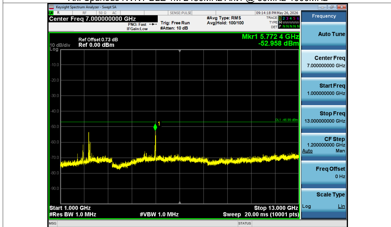
Rx. Spurious NVNT BLE 1M 2480MHz Ant1 @ 1000MHz-13000MHz
