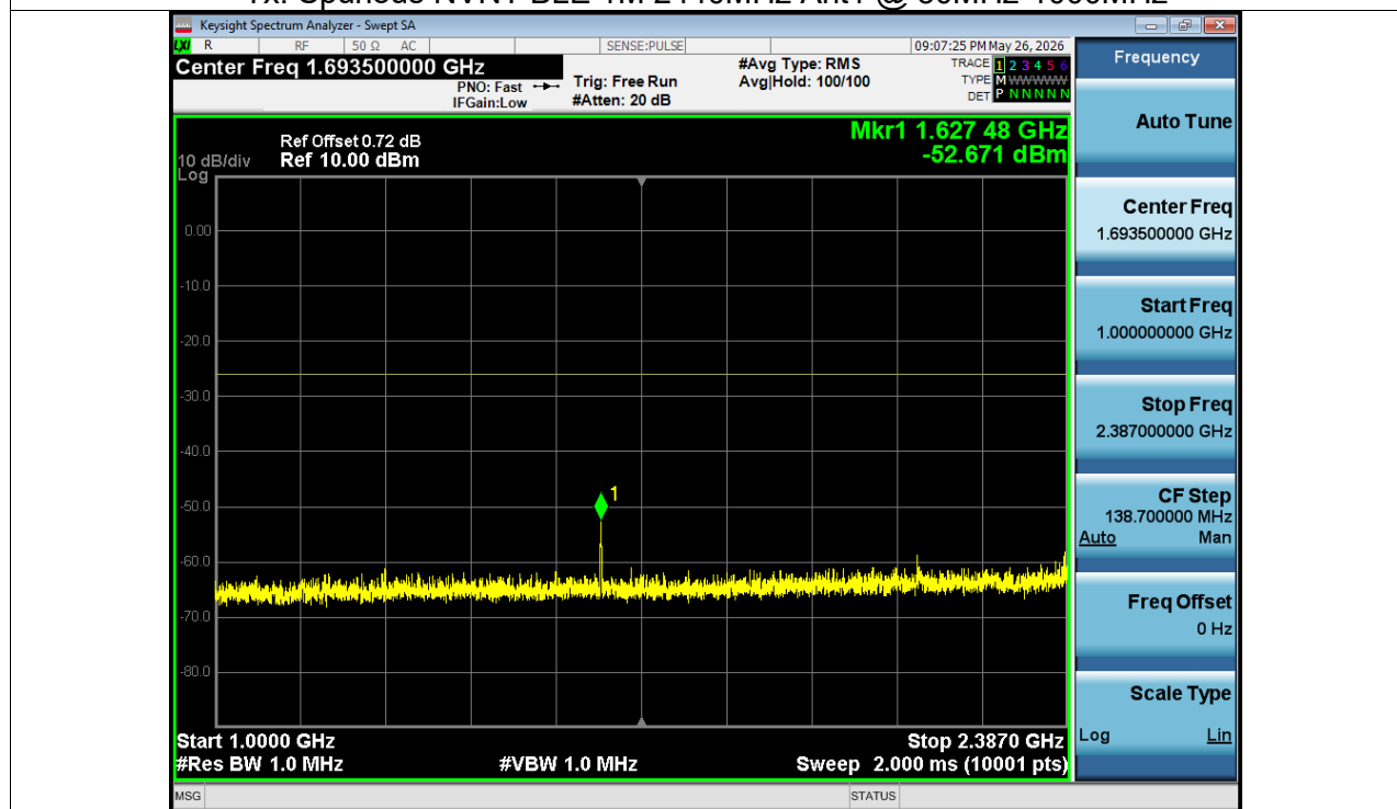
Tx. Spurious NVNT BLE 1M 2440MHz Ant1 @ 1000MHz-2387MHz
