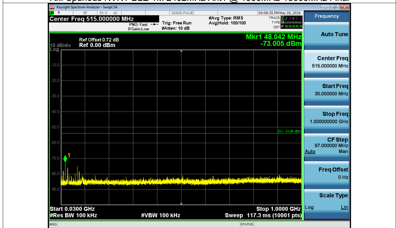
Rx. Spurious NVNT BLE 1M 2440MHz Ant1 @ 30MHz-1000MHz
