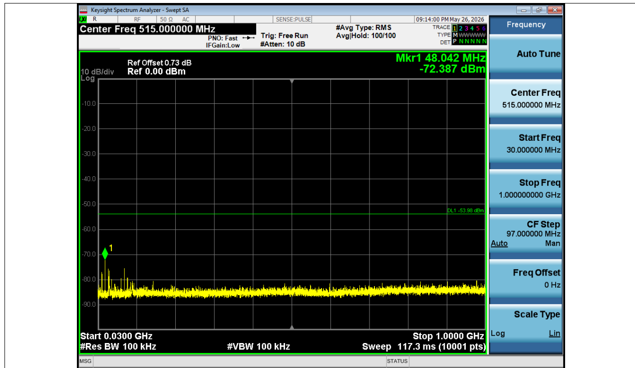
Rx. Spurious NVNT BLE 1M 2480MHz Ant1 @ 30MHz-1000MHz
