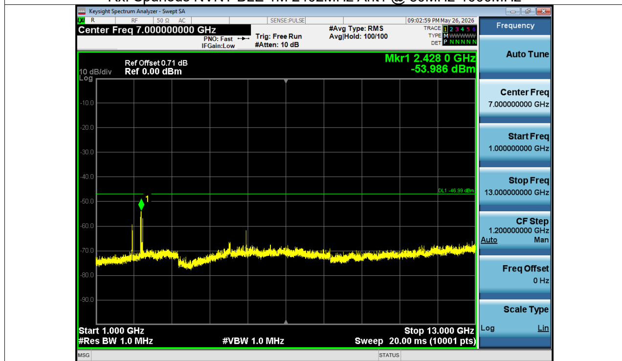
Rx. Spurious NVNT BLE 1M 2402MHz Ant1 @ 1000MHz-13000MHz
