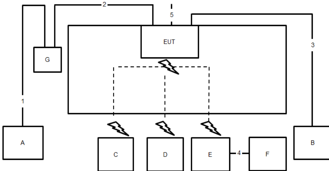
Test Setup Diagram - Radiated Unintentional Below 1GHz and Above 1GHz
