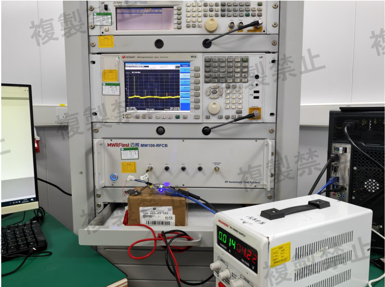
RF Conducted Test View-BT
