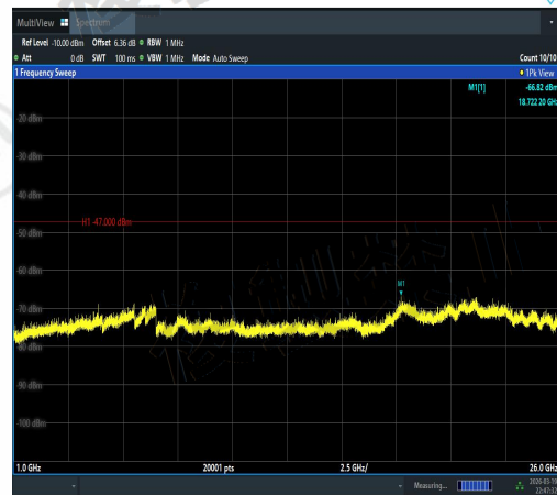
NTNV-11N20SISO-Ant1-5240-1000~26000-PAS
