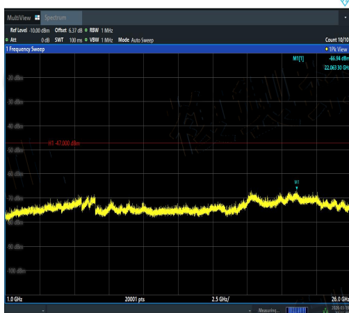
NTNV-11N20SISO-Ant2-5220-1000~26000-PASS
