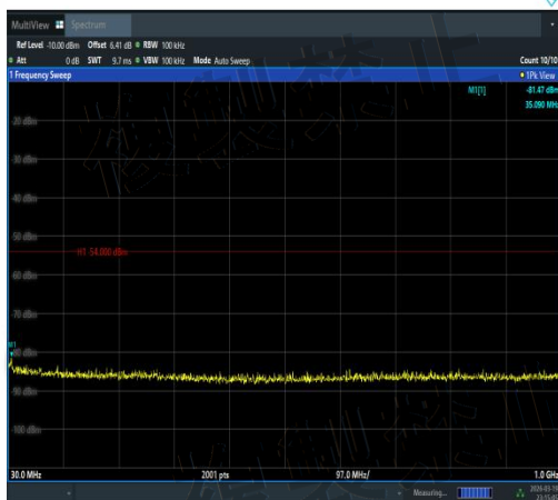
NTNV-11N40MIMO-Ant3-5230-30~1000-PASS
