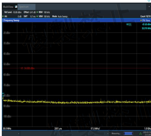
NTNV-11N20MIMO-Ant3-5240-30~1000-PASS
