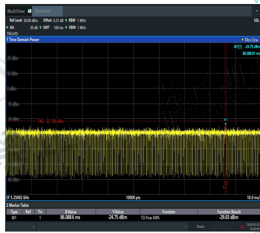
NTNV-11AX40SISO-Ant1-5230-5250~5251-PAS S
