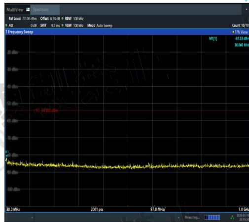
NTNV-11AC40MIMO-Ant2-5190-30~1000-PASS
