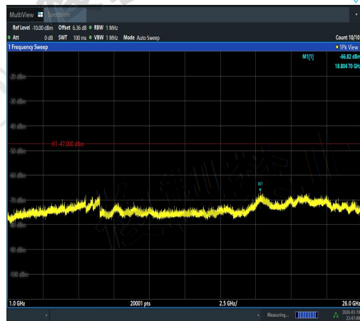
NTNV-11N20SISO-Ant1-5220-1000~26000-PASS
