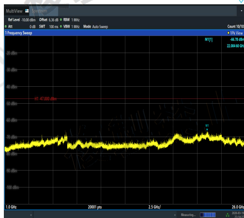
NTNV-11N40MIMO-Ant1-5230-1000~26000-PASS
