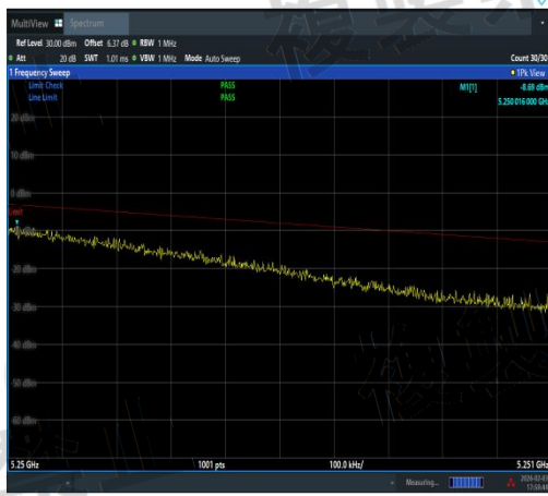
NTNV-11AX40SISO-Ant1-5230-5250~5251-PAS S
