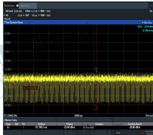
NTNV-11AC20MIMO-Ant1-5240-5250~5251-PAS
