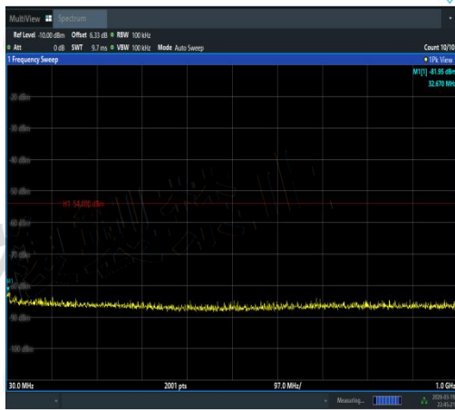
NTVN-11A-Ant1-5180-30~1000-PASS
