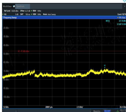
NTNV-11N20SISO-Ant2-5240-1000~26000-PAS
