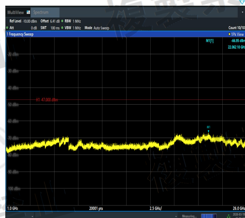
NTNV-11AC20SISO-Ant3-5220-1000~26000-PA SS
