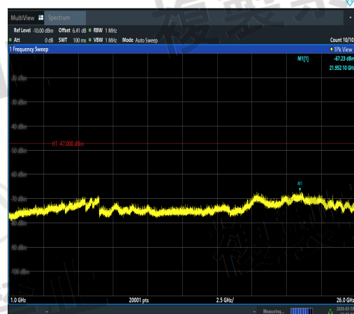
NTNV-11N40SISO-Ant3-5230-1000~26000-PAS
