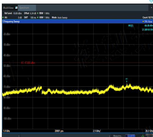
NTNV-11N40MIMO-Ant2-5190-1000~26000-PAS
