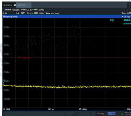
NTNV-11N20MIMO-Ant2-5220-30~1000-PASS
