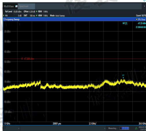
NTVN-11A-Ant3-5180-1000~26000-PASS
