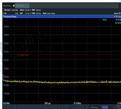
NTNV-11N40SISO-Ant2-5190-30~1000-PASS
