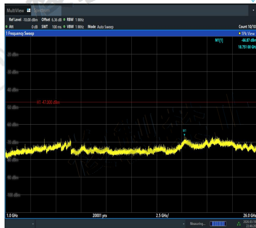
NTVN-11A-Ant1-5240-1000~26000-PASS
