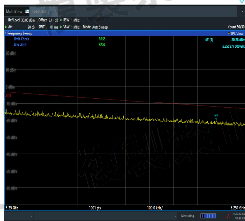
NTNV-11AC40MIMO-Ant1-5230-5250~5251-PAS
