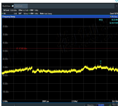
NTVN-11AC20MIMO-Ant2-5240-1000~26000-PA SS
