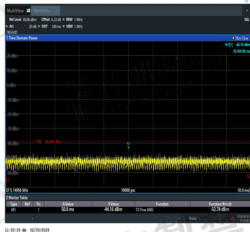
NTNV-11AC40SISO-Ant1-5190-5141.6~5150-PA
