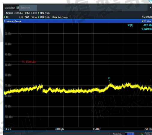
NTVN-11AC20SISO-Ant3-5180-1000~26000-PA SS
