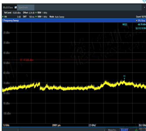
NTNV-11AC40MIMO-Ant2-5190-1000~26000-PA SS
