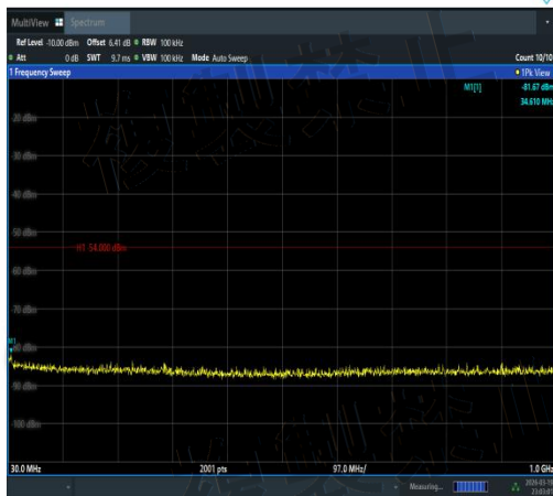
NTNV-11N20SISO-Ant3-5220-30~1000-PASS
