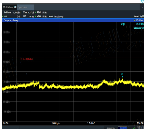
NTVN-11AC40SISO-Ant2-5230-1000~26000-PA SS
