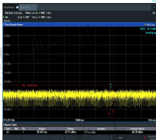
NTNV-11AC40SISO-Ant3-5230-5250~5251-PAS
