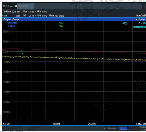
NTVN-11AX20MIMO-Ant2-5240-5250~5250.2-P ASS
