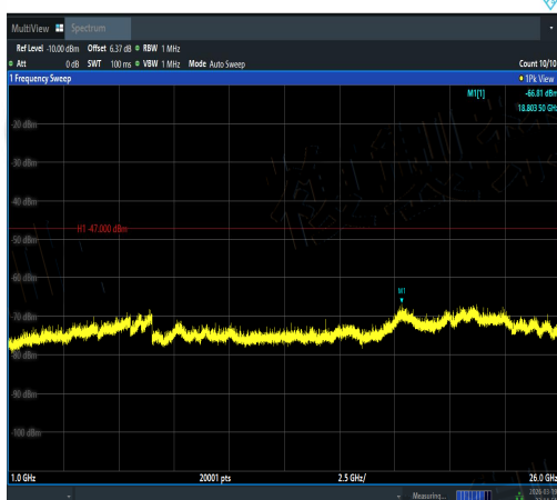
NTNV-11N40MIMO-Ant2-5230-1000~26000-PASS
