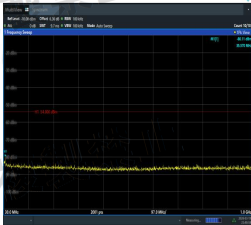
NTNV-11AC20SISO-Ant1-5220-30~1000-PASS
