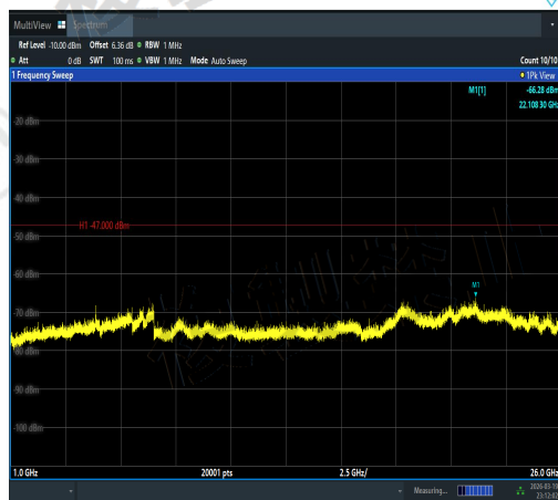
NTNV-11N20MIMO-Ant1-5240-1000~26000-PASS
