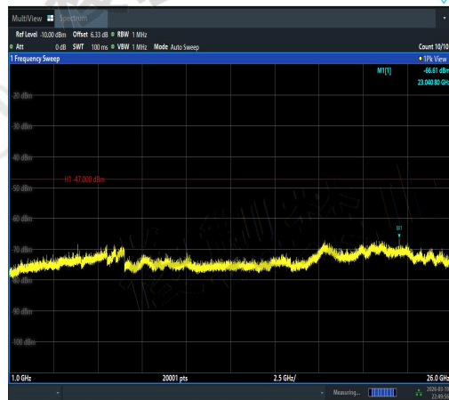
NTVN-11AC40SISO-Ant1-5190-1000~26000-PA SS
