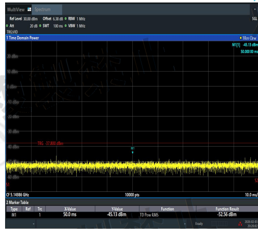
NTNV-11AX40SISO-Ant3-5190-5141.6~5150-PA SS
