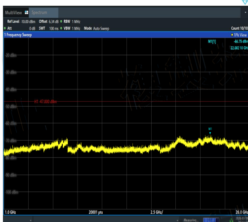
NTVN-11AC40SISO-Ant2-5190-1000~26000-PA SS
