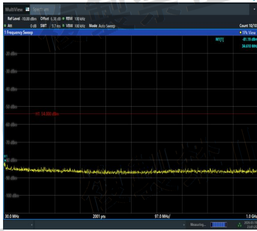
NTVN-11A-Ant3-5180-30~1000-PASS
