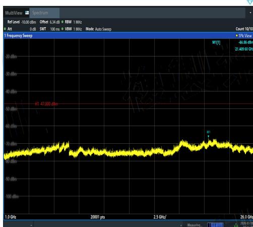
NTVN-11AC20SISO-Ant2-5180-1000~26000-PA SS
