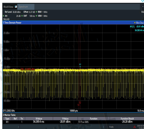
NTNV-11AX20SISO-Ant2-5240-5250~5250.2-PA
