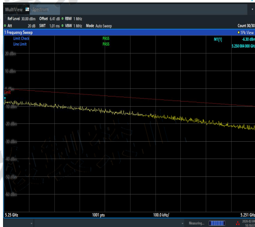
NTNV-11AC20MIMO-Ant3-5240-5250~5251-PAS
