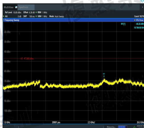
NTVN-11AC40SISO-Ant3-5190-1000~26000-PA SS
