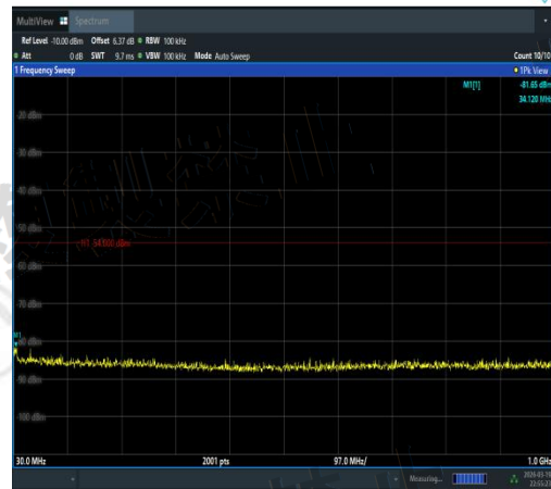
NTNV-11N20SISO-Ant2-5240-30~1000-PASS
