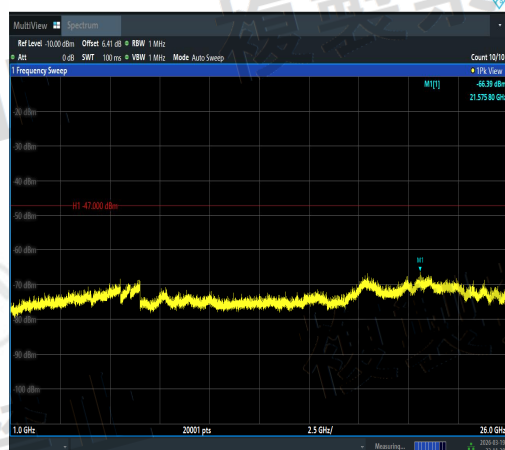
NTNV-11N20MIMO-Ant3-5220-1000~26000-PAS
