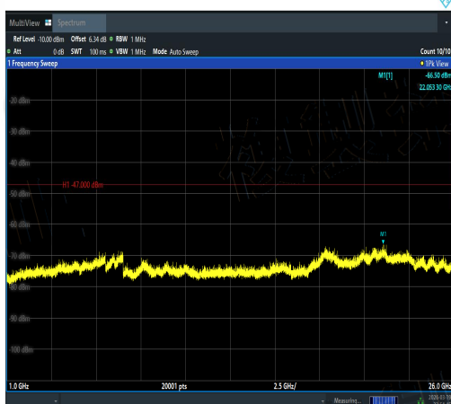
NTNV-11N20SISO-Ant2-5180-1000~26000-PAS
