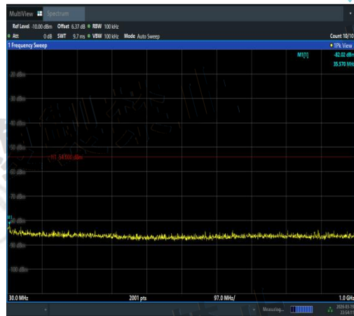
NTVN-11A-Ant2-5240-30~1000-PASS
