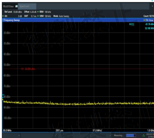
NTNV-11AC40MIMO-Ant3-5190-30~1000-PASS
