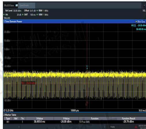
NTNV-11AC20MIMO-Ant3-5240-5250~5251-PAS
