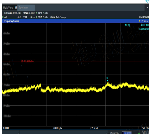
NTNV-11AC20MIMO-Ant2-5180-1000~26000-PA SS
