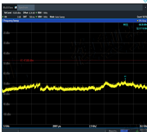
NTNV-11N20MIMO-Ant2-5180-1000~26000-PAS
