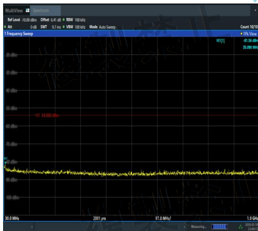
NTNV-11N40SISO-Ant1-5230-30~1000-PASS
