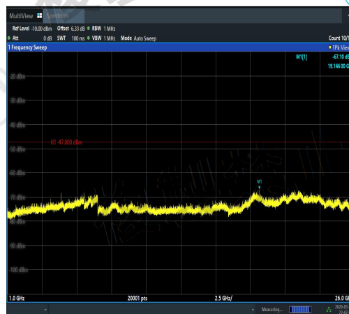
NTNV-11N40SISO-Ant1-5190-1000~26000-PASS
