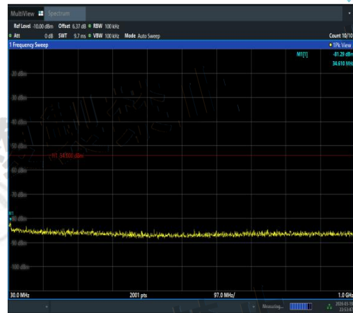
NTVN-11A-Ant2-5220-30~1000-PASS
