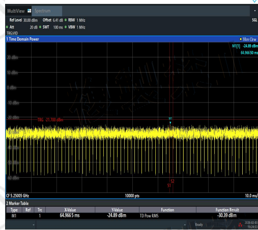
NTNV-11AC20SISO-Ant3-5240-5250~5251-PAS
