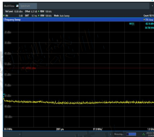
NTNV-11N20SISO-Ant2-5220-30~1000-PASS
