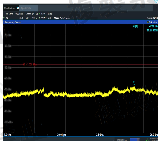
NTVN-11AC40MIMO-Ant3-5230-1000~26000-PA SS
