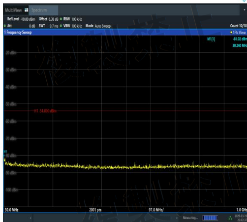
NTNV-11N20SISO-Ant3-5180-30~1000-PASS
