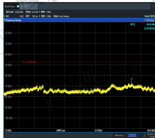
NTVN-11AC40SISO-Ant1-5230-1000~26000-PA SS
