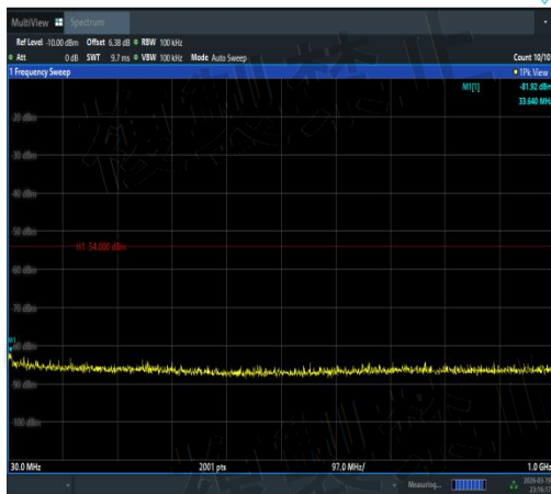
NTNV-11AC20MIMO-Ant3-5180-30~1000-PASS
