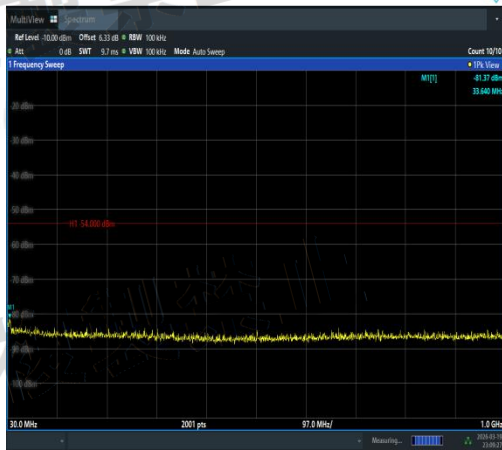
NTNV-11N20MIMO-Ant1-5180-30~1000-PASS
