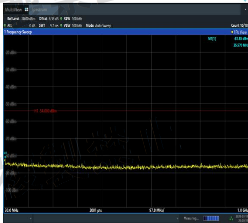
NTVN-11AC40MIMO-Ant1-5230-30~1000-PASS
