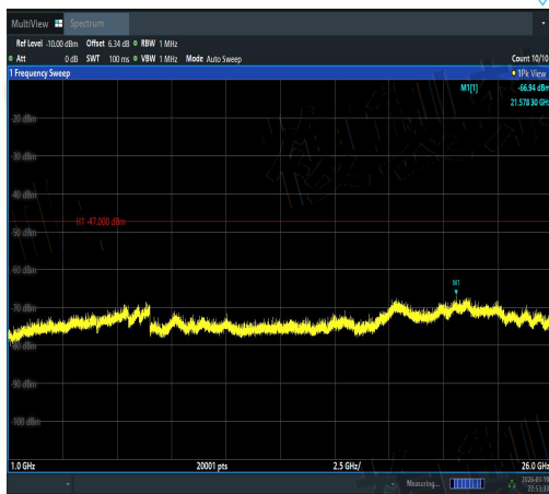
NTVN-11A-Ant2-5180-1000~26000-PASS
