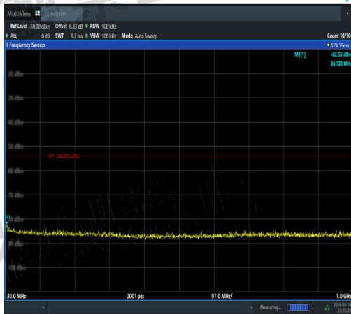
NTNV-11AC20MIMO-Ant1-5180-30~1000-PASS
