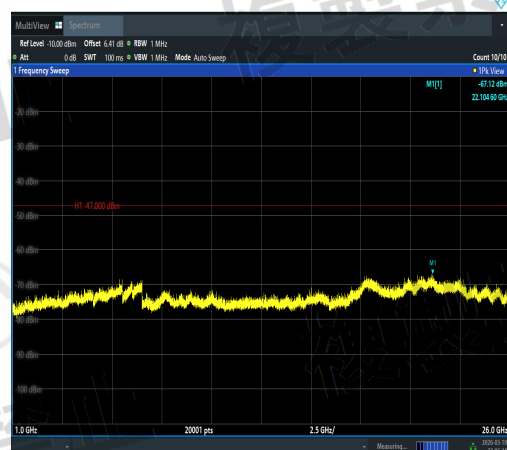
NTVN-11AC40SISO-Ant3-5230-1000~26000-PA SS
