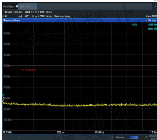
NTVN-11A-Ant3-5240-30~1000-PASS
