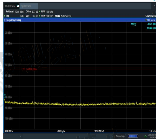
NTVN-11AC20MIMO-Ant2-5240-30~1000-PASS
