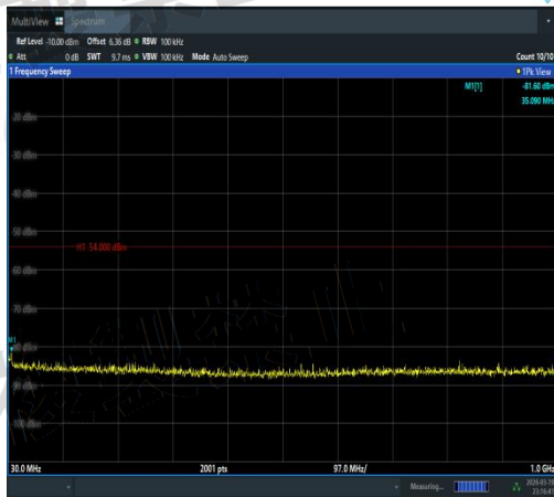
NTNV-11AC20MIMO-Ant1-5220-30~1000-PASS
