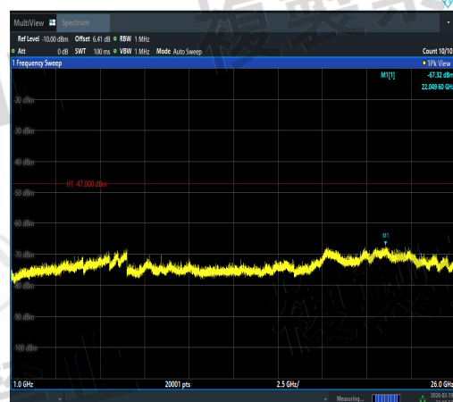
NTVN-11AC20MIMO-Ant3-5240-1000~26000-PA SS
