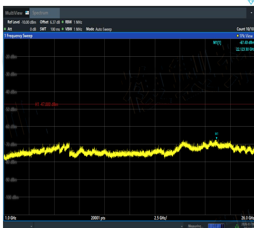
NTNV-11AC20SISO-Ant2-5220-1000~26000-PA SS
