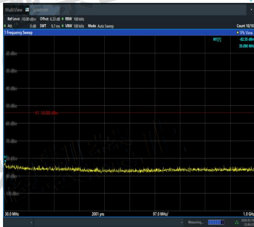
NTNV-11N20SISO-Ant1-5180-30~1000-PASS
