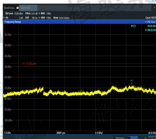
NTNV-11N20SISO-Ant3-5220-1000~26000-PASS
