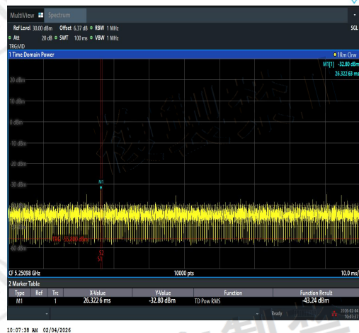
NTNV-11AC20MIMO-Ant2-5240-5250~5251-PAS
