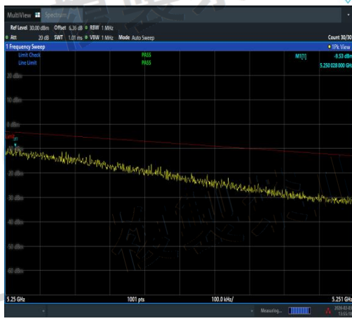
NTNV-11AX40SISO-Ant1-5230-5250~5251-PAS S
