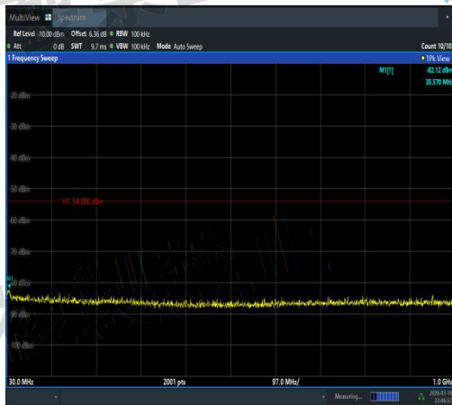
NTNV-11N20SISO-Ant1-5220-30~1000-PASS
