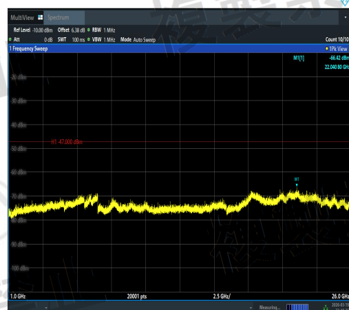
NTNV-11N20MIMO-Ant3-5180-1000~26000-PAS
