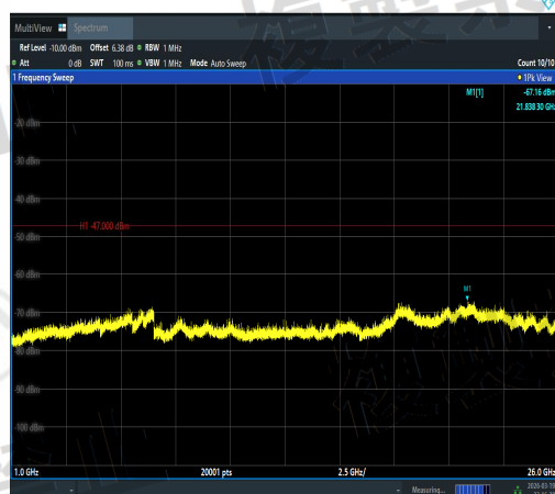
NTNV-11AC20MIMO-Ant3-5180-1000~26000-PA SS
