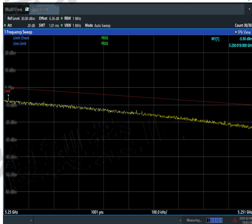
NTNV-11AC20MIMO-Ant1-5240-5250~5251-PAS
