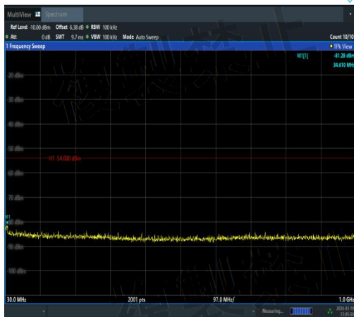
NTVN-11AC40SISO-Ant3-5190-30~1000-PASS
