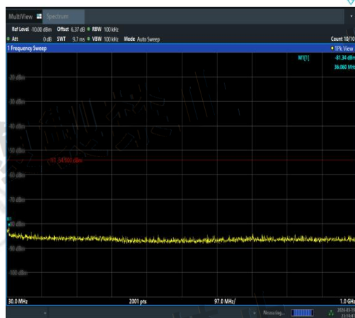
NTNV-11N40MIMO-Ant2-5230-30~1000-PASS
