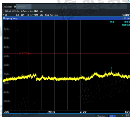
NTNV-11N40SISO-Ant3-5190-1000~26000-PASS
