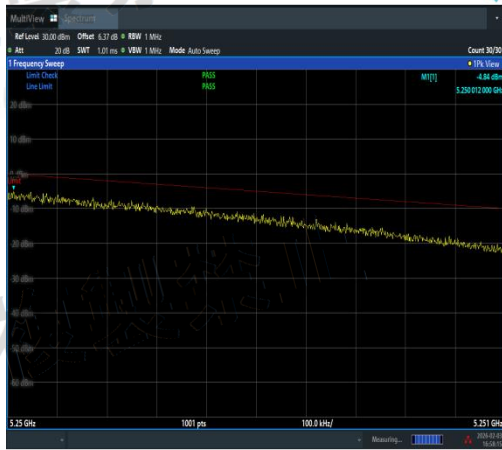
NTNV-11AC20SISO-Ant2-5240-5250~5251-PAS
