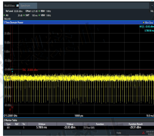
NTNV-11AC20SISO-Ant2-5240-5250~5251-PAS
