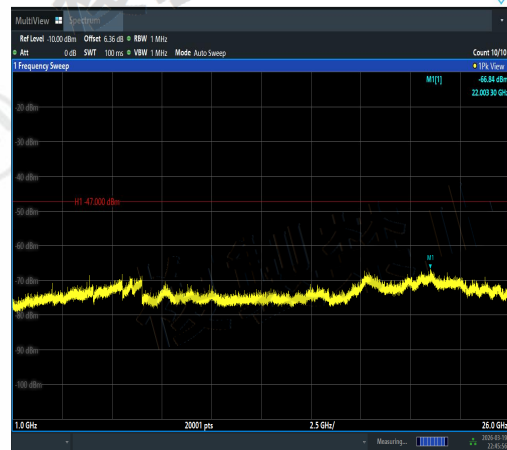
NTVN-11A-Ant1-5220-1000~26000-PASS
