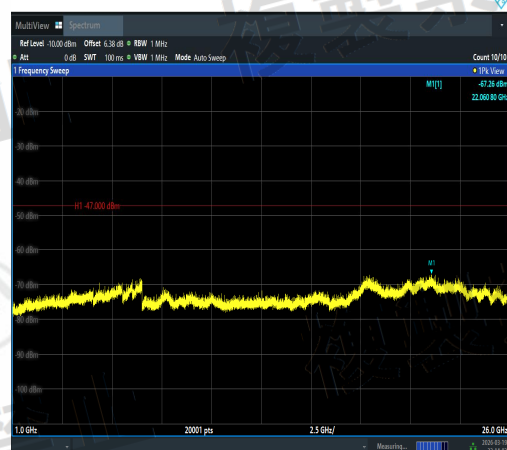
NTNV-11N40MIMO-Ant3-5190-1000~26000-PAS
