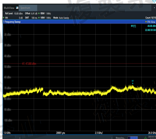
NTNV-11N40MIMO-Ant3-5230-1000~26000-PASS
