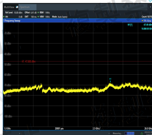
NTVN-11A-Ant3-5240-1000~26000-PASS
