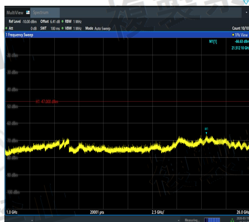
NTNV-11AC20MIMO-Ant3-5220-1000~26000-PA SS
