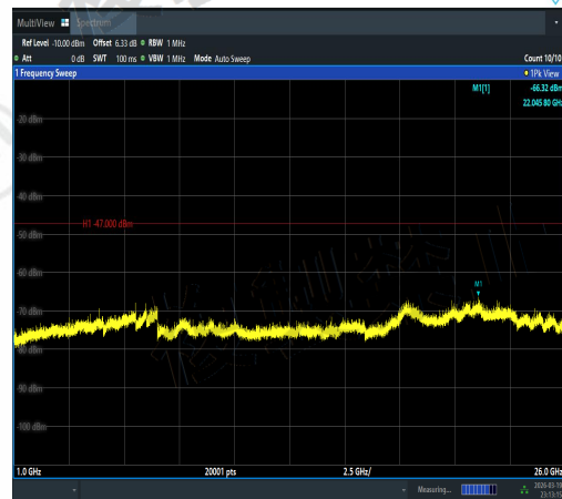
NTNV-11N40MIMO-Ant1-5190-1000~26000-PAS
