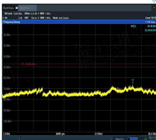
NTVN-11AC40MIMO-Ant2-5230-1000~26000-PA SS
