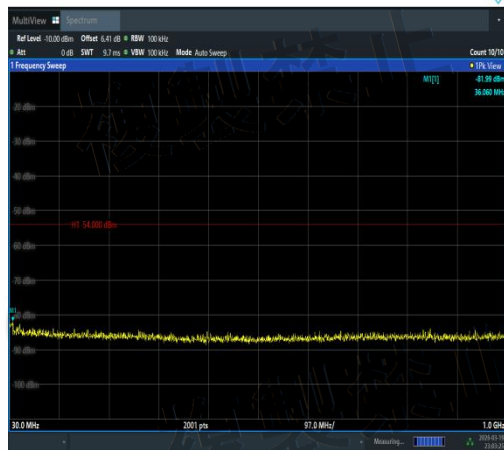
NTNV-11N20SISO-Ant3-5240-30~1000-PASS
