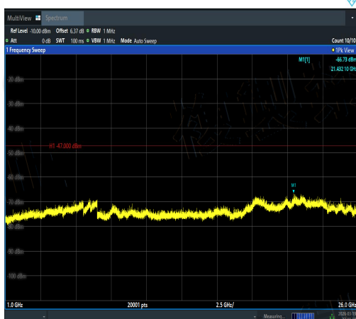
NTNV-11N20MIMO-Ant2-5220-1000~26000-PAS
