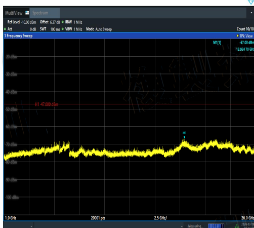
NTNV-11AC20MIMO-Ant2-5220-1000~26000-PA SS
