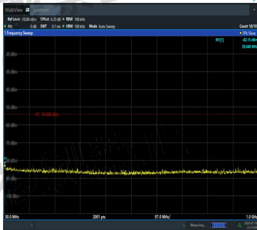
NTNV-11N40MIMO-Ant1-5190-30~1000-PASS
