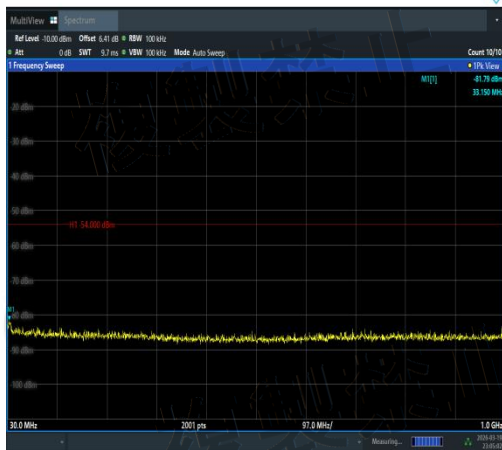
NTNV-11AC20SISO-Ant3-5220-30~1000-PASS
