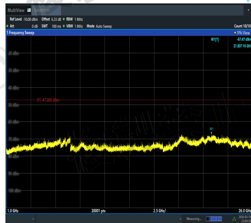
NTNV-11N20MIMO-Ant1-5180-1000~26000-PAS
