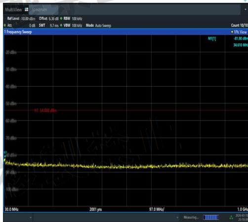
NTNV-11N20MIMO-Ant1-5220-30~1000-PASS
