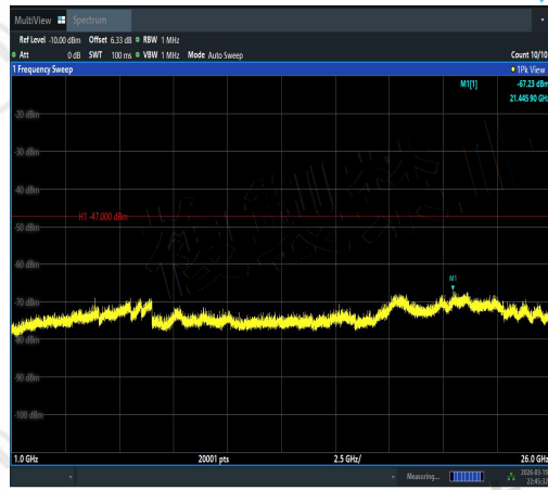
NTVN-11A-Ant1-5180-1000~26000-PASS
