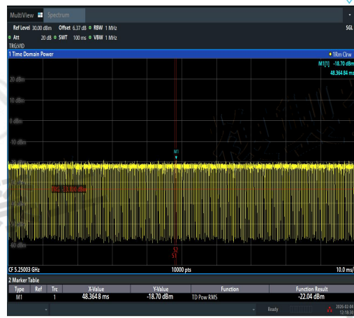
NTVN-11AX20MIMO-Ant2-5240-5250~5250.2-P ASS
