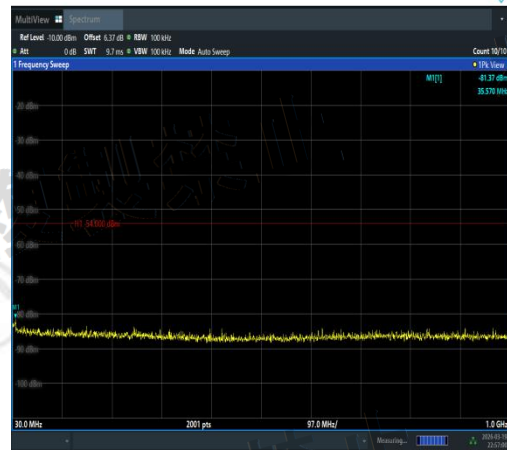
NTNV-11AC20SISO-Ant2-5220-30~1000-PASS
