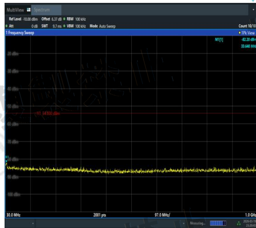
NTVN-11AC40MIMO-Ant2-5230-30~1000-PASS
