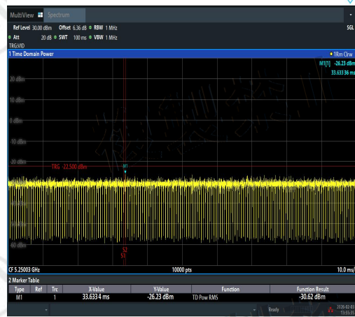
NTNV-11AX40SISO-Ant1-5230-5250~5251-PAS S
