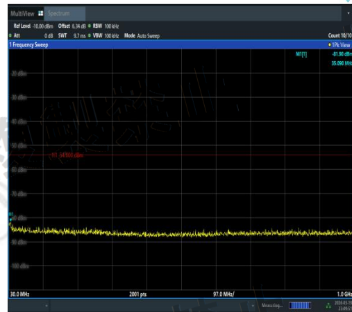
NTNV-11N20MIMO-Ant2-5180-30~1000-PASS
