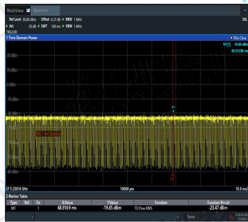
NTVN-11AX20MIMO-Ant2-5240-5250~5250.2-P ASS
