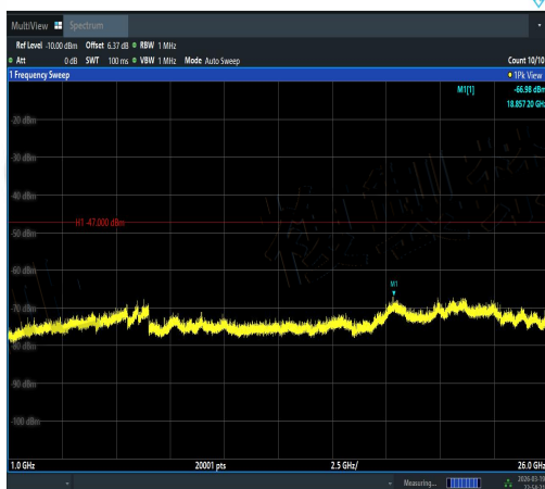
NTVN-11A-Ant2-5240-1000~26000-PASS
