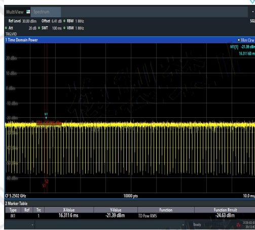
NTNV-11AX20SISO-Ant3-5240-5250~5250.2-PA
