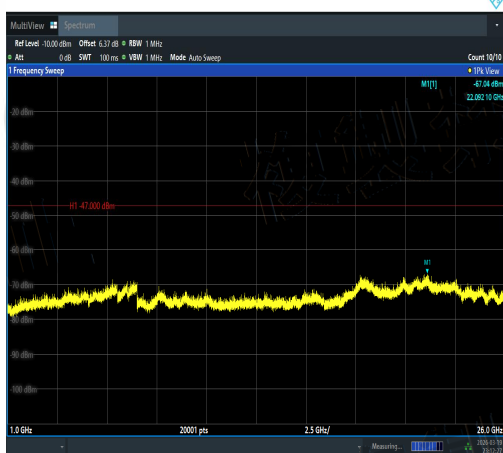
NTNV-11N20MIMO-Ant2-5240-1000~26000-PASS
