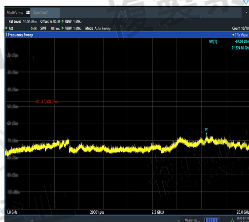
NTNV-11AC40MIMO-Ant3-5190-1000~26000-PA SS
