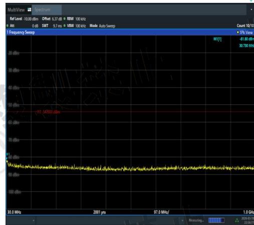
NTNV-11N40SISO-Ant2-5230-30~1000-PASS
