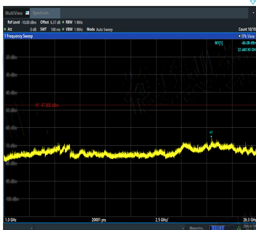
NTNV-11N40SISO-Ant2-5230-1000~26000-PAS
