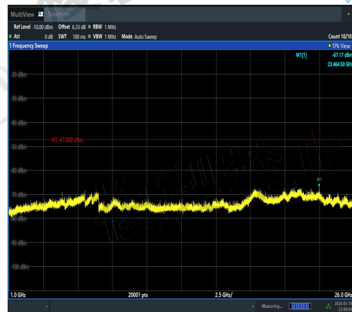
NTVN-11AC20SISO-Ant1-5180-1000~26000-PA SS
