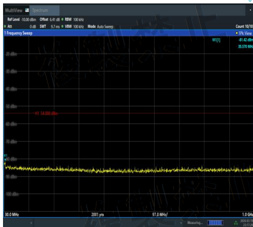
NTNV-11AC20MIMO-Ant3-5220-30~1000-PASS
