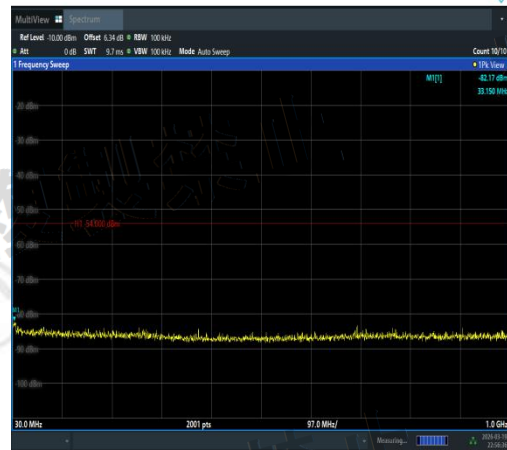
NTVN-11AC20SISO-Ant2-5180-30~1000-PASS
