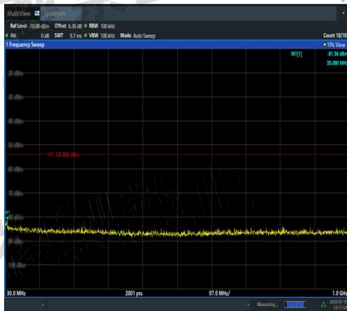
NTVN-11AC20MIMO-Ant1-5240-30~1000-PASS
