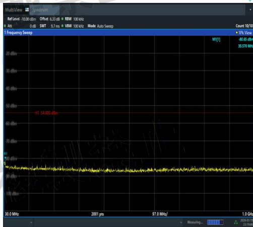
NTNV-11AC40MIMO-Ant1-5190-30~1000-PASS
