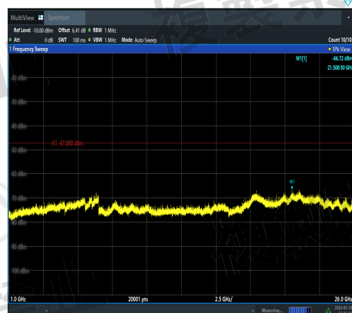
NTNV-11N20SISO-Ant3-5240-1000~26000-PAS
