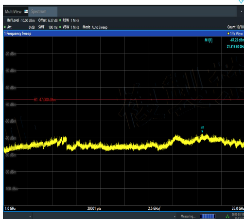
NTVN-11A-Ant2-5220-1000~26000-PASS
