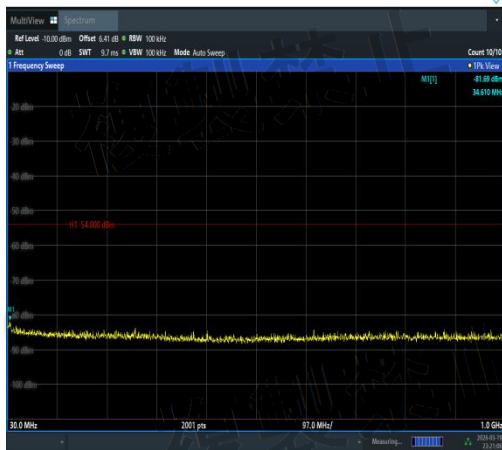
NTVN-11AC40MIMO-Ant3-5230-30~1000-PASS
