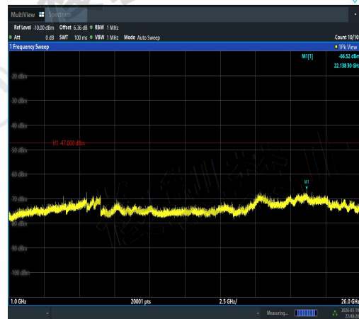
NTNV-11N40SISO-Ant1-5230-1000~26000-PAS
