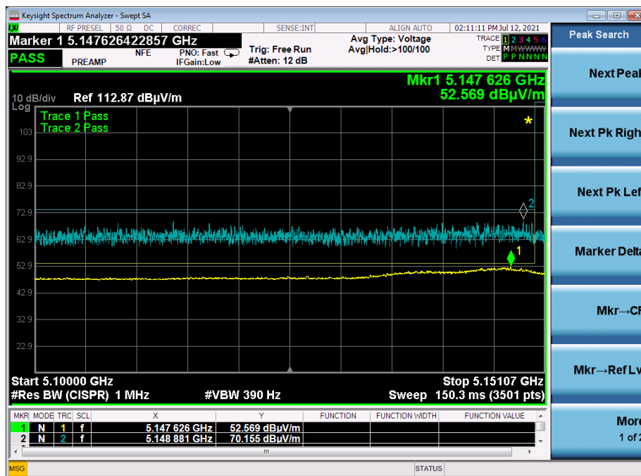
Graph 2: Band Edge ax20 Mode Middle 5210 MHz
