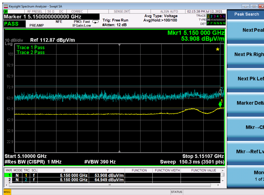
Graph 4: Band Edge ax40 Mode Low 5180 MHz
