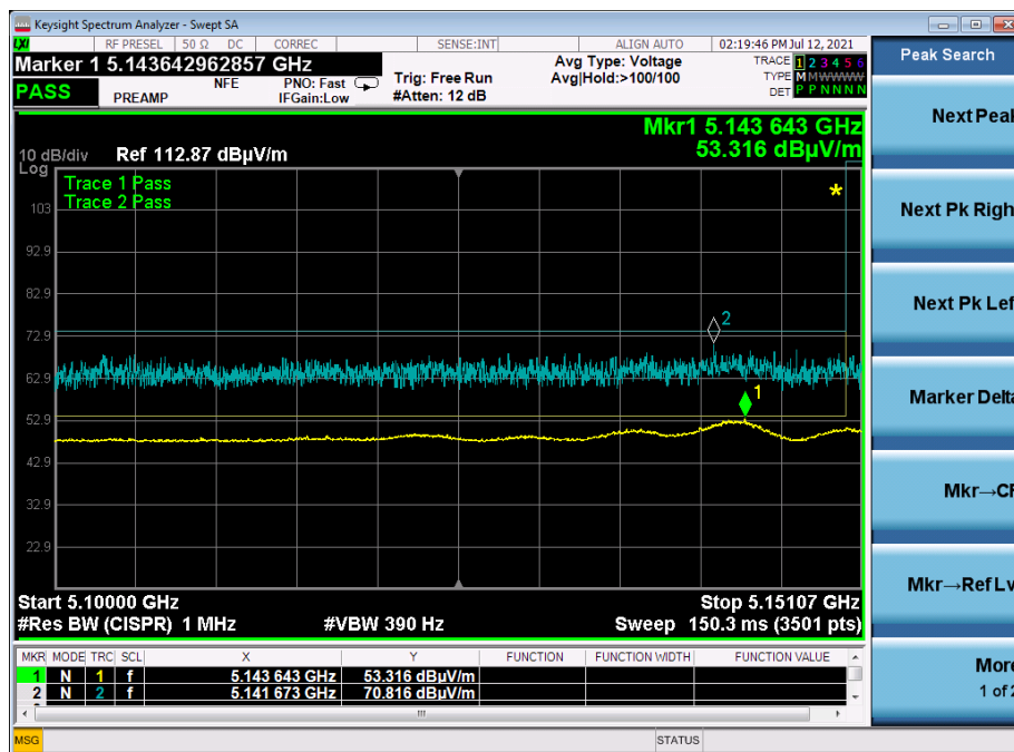
Graph 6: Band Edge ax80 Mode 5210 MHz
