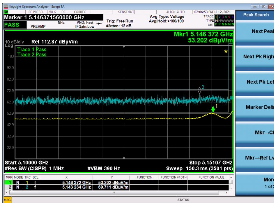
Graph 1: Band Edge ax20 Mode Low 5180 MHz
