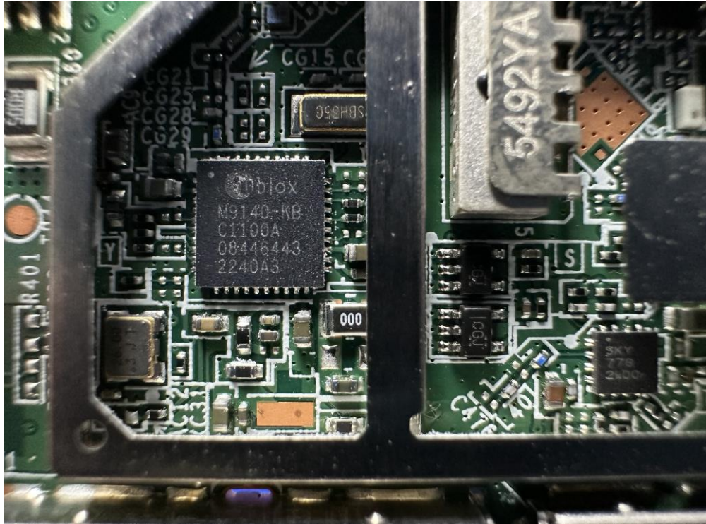
(25) EUT Photo
