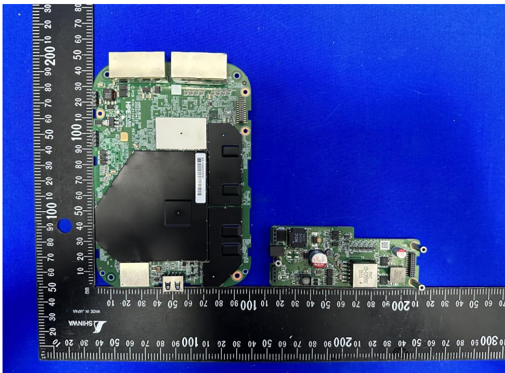
(7) EUT Photo
