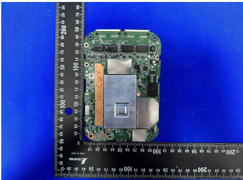
(11) EUT Photo
