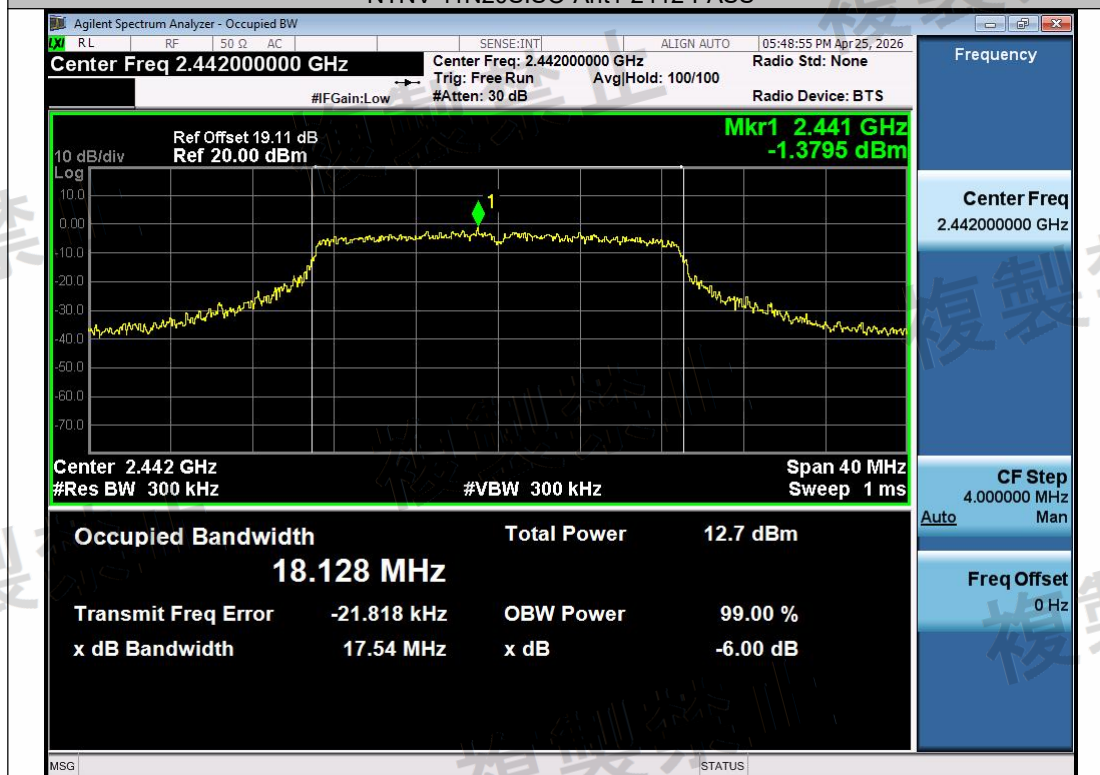
NTNV-11N20SISO-Ant1-2442-PASS
