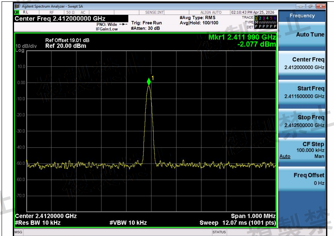
NTNV-11B-Ant1-2412-PASS
