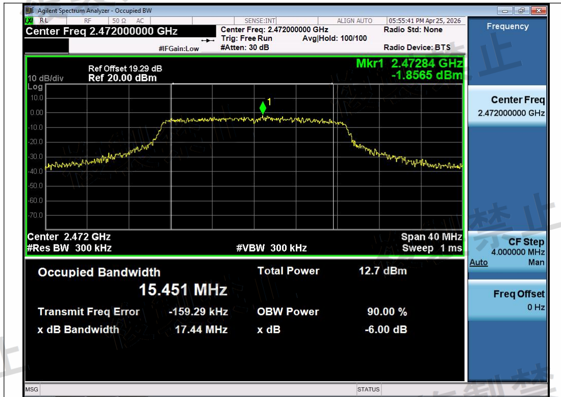
NTNV-11N20SISO-Ant1-2472-PASS
