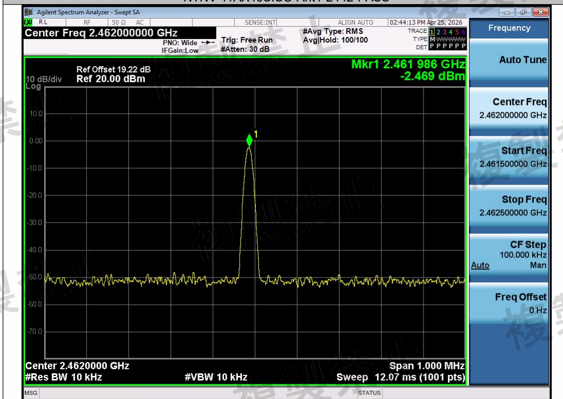
NTNV-11AX40SISO-Ant1-2462-PASS
