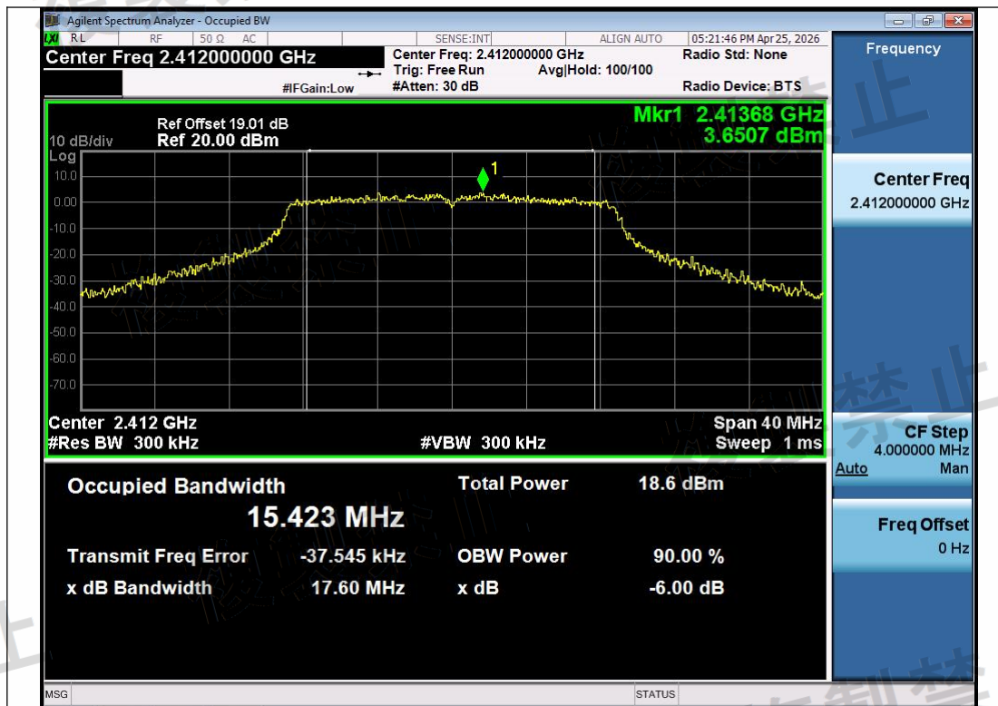
NTNV-11N20SISO-Ant1-2412-PASS
