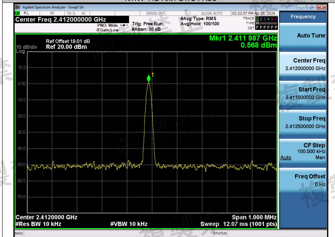
NTNV-11G-Ant1-2412-PASS
