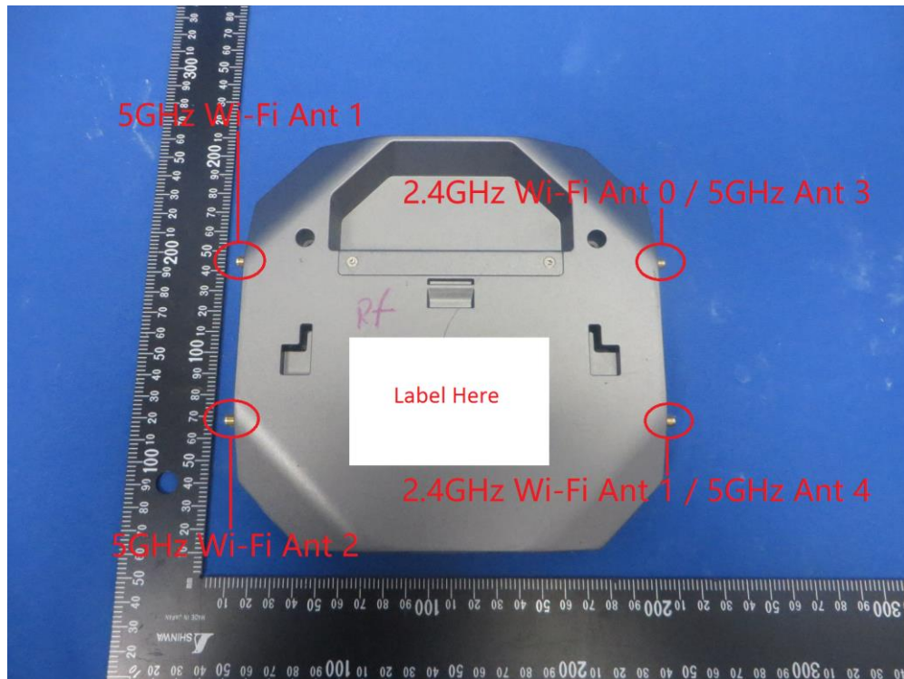
(5) EUT Photo_OAW-AP1322
