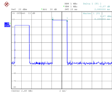
CH78-DH5
