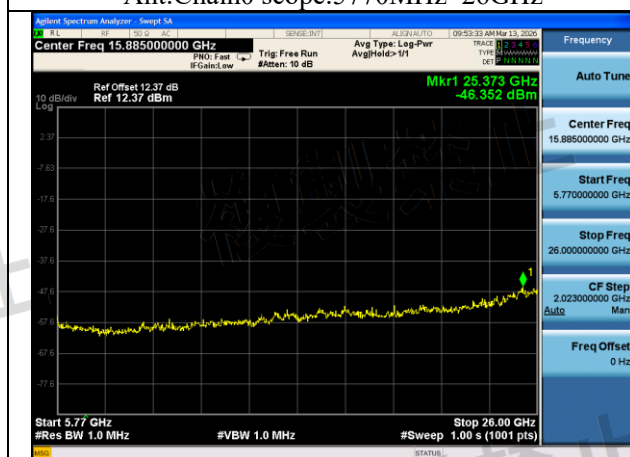
Mode:802.11ac VHT40 Frequency:5710MHz Ant:Chain0 scope:5770MHz~26GHz
