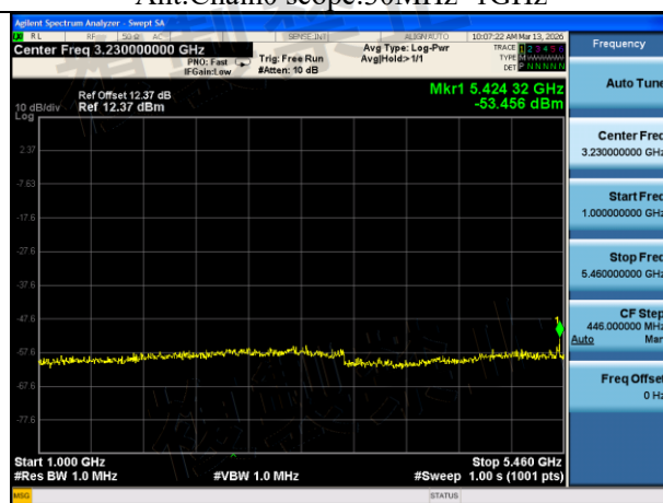
Mode:802.11ac VHT80 Frequency:5530MHz Ant:Chain0 scope:1GHz~5460MHz
