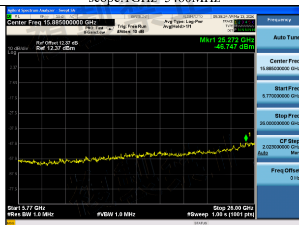
Mode:802.11n HT40 Frequency:5510MHz Ant:Chain1 scope:5770MHz~26GHz
