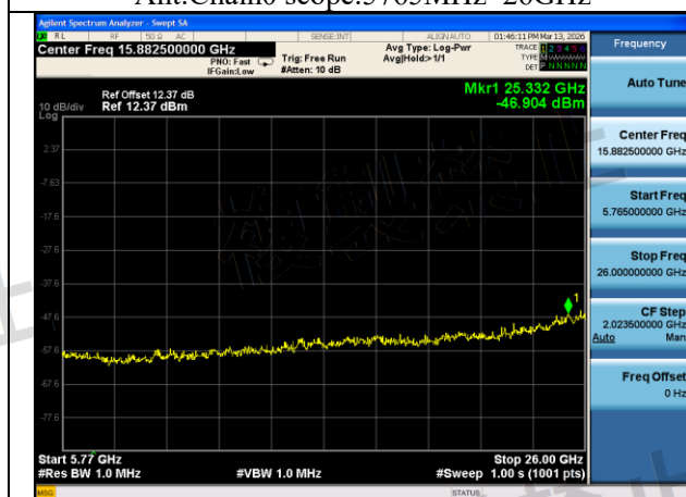
Mode:802.11ac VHT20 Frequency:5720MHz Ant:Chain0 scope:5765MHz~26GHz
