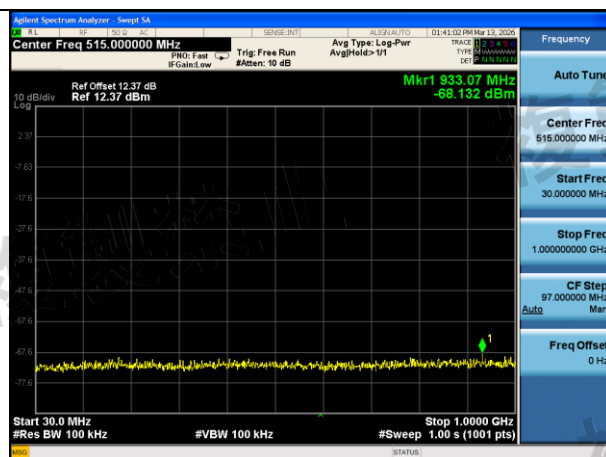
Mode:802.11ax HE20 Frequency:5620MHz Ant:Chain0 scope:30MHz~1GHz
