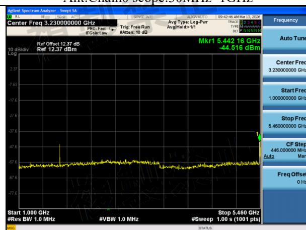
Mode:802.11ac VHT40 Frequency:5510MHz Ant:Chain0 scope:1GHz~5460MHz
