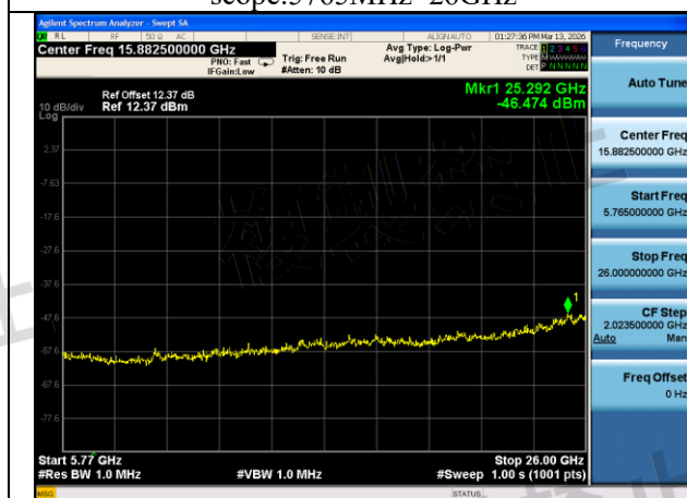
Mode:802.11a Frequency:5720MHz Ant:Chain0 scope:5765MHz~26GHz
