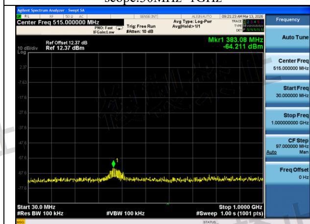
Mode:802.11n HT40 Frequency:5710MHz Ant:Chain0 scope:30MHz~1GHz
