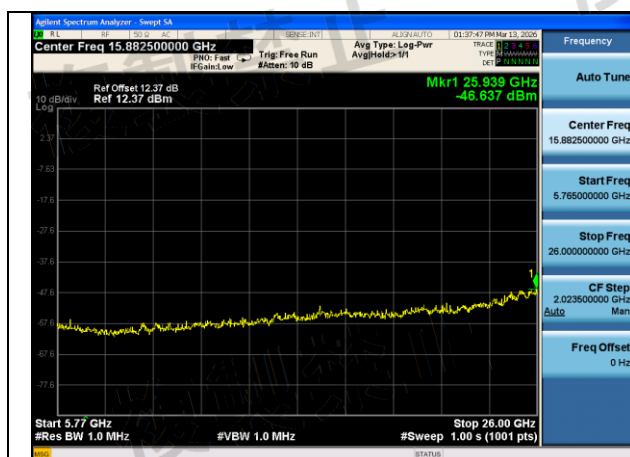
Mode:802.11ac VHT20 Frequency:5500MHz Ant:Chain0 scope:5765MHz~26GHz
