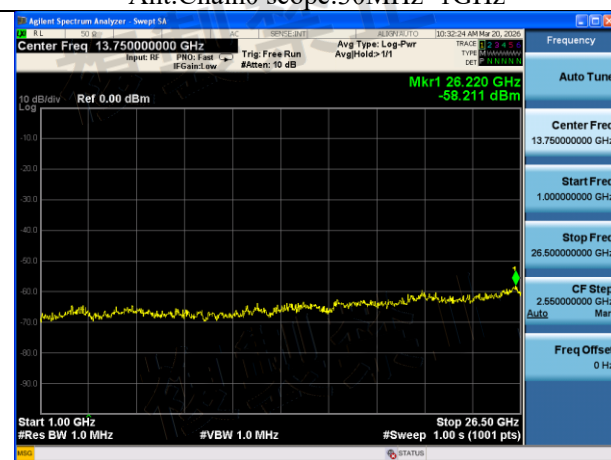
Mode:802.11ac VHT40 Frequency:5510MHz Ant:Chain0 scope:1GHz~26.5GHz
