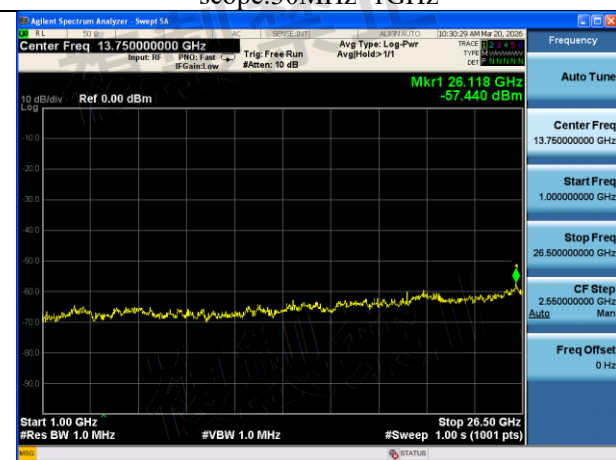
Mode:802.11n HT20 Frequency:5500MHz Ant:Chain0 scope:1GHz~26.5GHz
