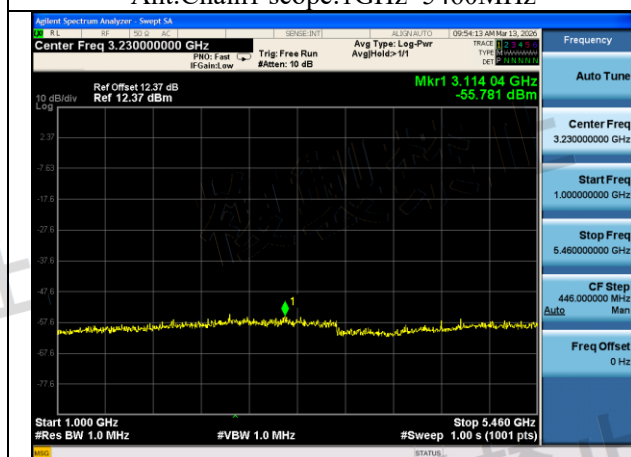
Mode:802.11ac VHT40 Frequency:5710MHz Ant:Chain1 scope:1GHz~5460MHz
