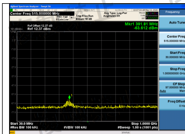
Mode:802.11ac VHT80 Frequency:5530MHz Ant:Chain0 scope:30MHz~1GHz
