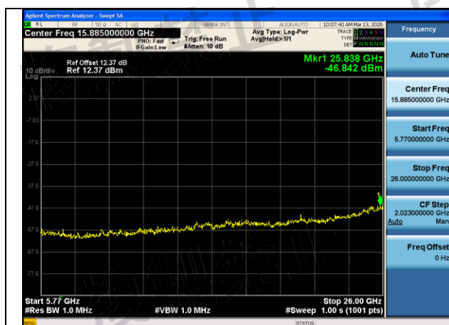
Mode:802.11ac VHT80 Frequency:5530MHz Ant:Chain0 scope:5770MHz~26GHz
