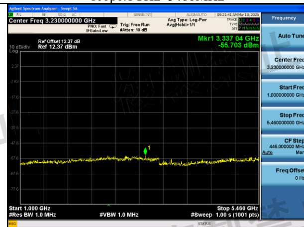
Mode:802.11n HT40 Frequency:5710MHz Ant:Chain0 scope:1GHz~5460MHz
