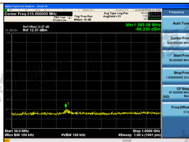
Mode:802.11ax HE40 Frequency:5630MHz Ant:Chain0 scope:30MHz~1GHz
