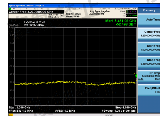
Mode:802.11ax HE40 Frequency:5510MHz Ant:Chain1 scope:1GHz~5460MHz
