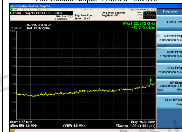
Mode:802.11ac VHT80 Frequency:5690MHz Ant:Chain0 scope:5770MHz~26GHz
