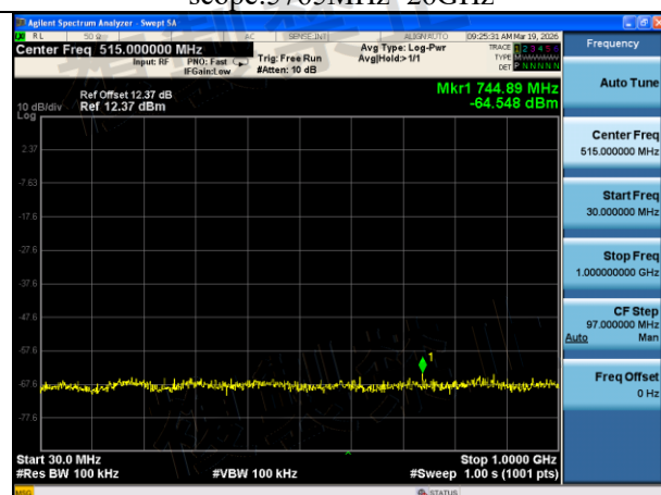
Mode:802.11n HT20 Frequency:5500MHz Ant:Chain1 scope:30MHz~1GHz
