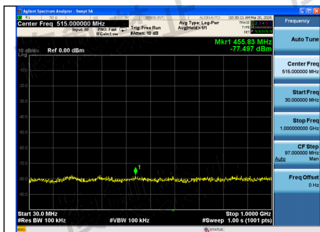
Mode:802.11n HT20 Frequency:5500MHz Ant:Chain0 scope:30MHz~1GHz
