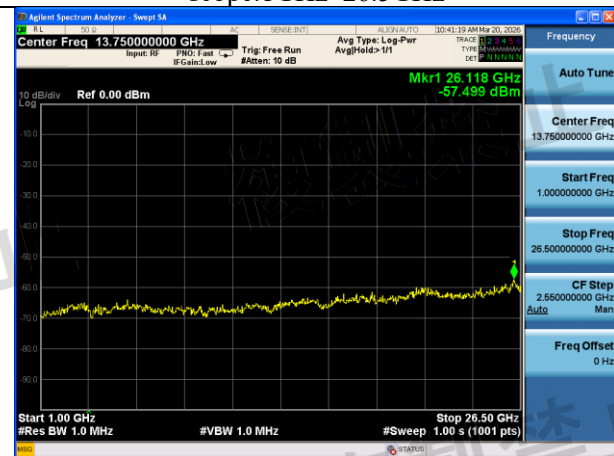
Mode:802.11n HT40 Frequency:5710MHz Ant:Chain0 scope:1GHz~26.5GHz
