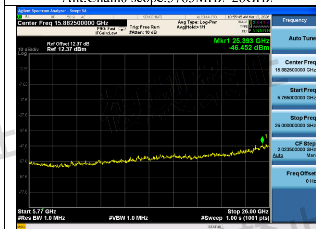
Mode:802.11ax HE20 Frequency:5720MHz Ant:Chain0 scope:5765MHz~26GHz
