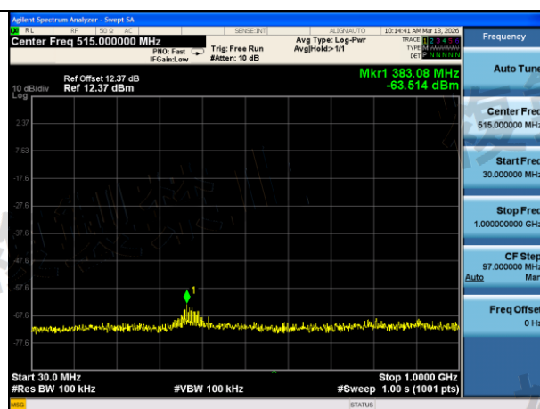
Mode:802.11ac VHT80 Frequency:5610MHz Ant:Chain0 scope:30MHz~1GHz
