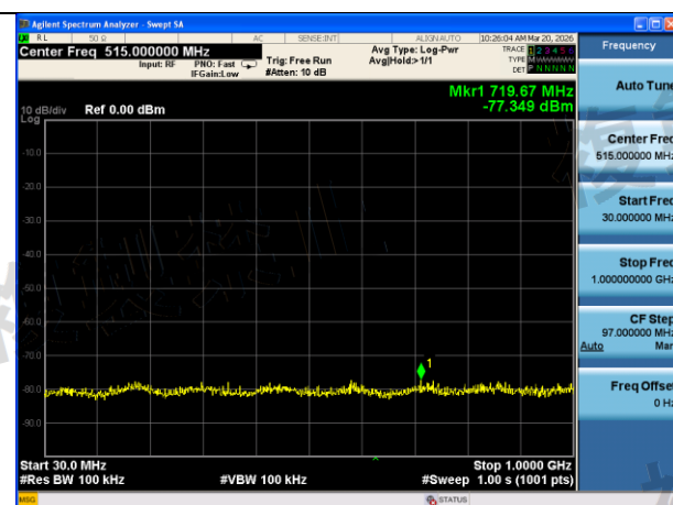
Mode:802.11ac VHT80 Frequency:5610MHz Ant:Chain1 scope:30MHz~1GHz
