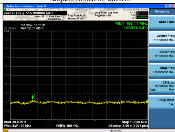
Mode:802.11a Frequency:5500MHz Ant:Chain1 scope:30MHz~1GHz
