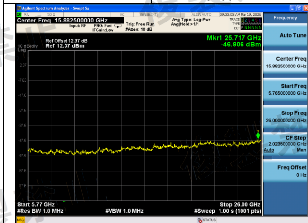
Mode:802.11ac VHT20 Frequency:5620MHz Ant:Chain1 scope:5765MHz~26GHz
