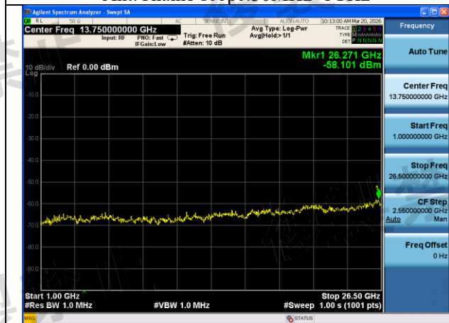
Mode:802.11ac VHT40 Frequency:5630MHz Ant:Chain1 scope:1GHz~26.5GHz
