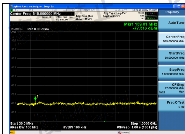
Mode:802.11ac VHT80 Frequency:5530MHz Ant:Chain1 scope:30MHz~1GHz
