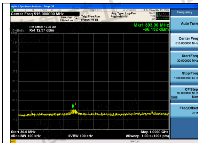
Mode:802.11ax HE40 Frequency:5510MHz Ant:Chain0 scope:30MHz~1GHz
