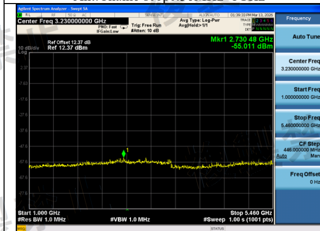
Mode:802.11ac VHT20 Frequency:5620MHz Ant:Chain0 scope:1GHz~5460MHz
