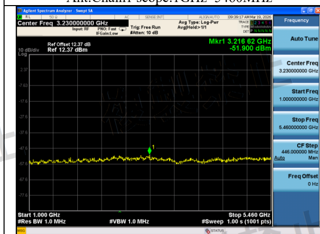
Mode:802.11ac VHT80 Frequency:5690MHz Ant:Chain1 scope:1GHz~5460MHz
