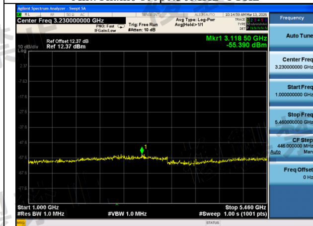
Mode:802.11ac VHT80 Frequency:5610MHz Ant:Chain0 scope:1GHz~5460MHz
