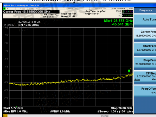
Mode:802.11ac VHT40 Frequency:5510MHz Ant:Chain1 scope:5770MHz~26GHz
