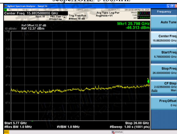
Mode:802.11a Frequency:5500MHz Ant:Chain1 scope:5765MHz~26GHz
