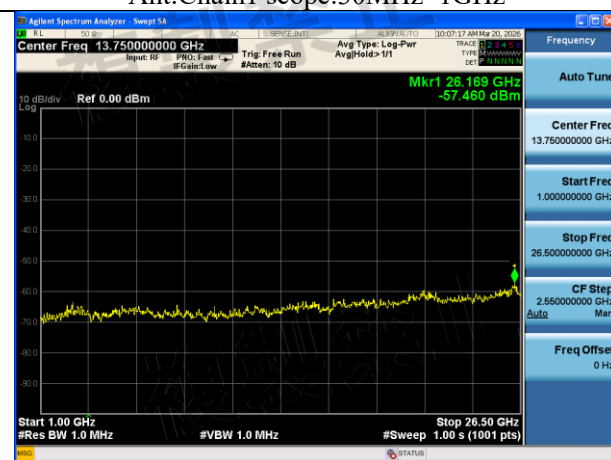
Mode:802.11ac VHT40 Frequency:5510MHz Ant:Chain1 scope:1GHz~26.5GHz
