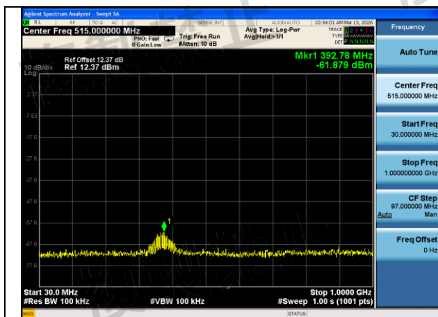
Mode:802.11ax HE20 Frequency:5500MHz Ant:Chain0 scope:30MHz~1GHz
