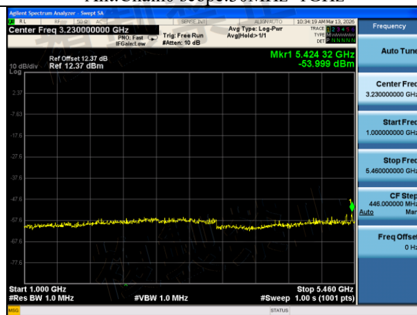
Mode:802.11ax HE20 Frequency:5500MHz Ant:Chain0 scope:1GHz~5460MHz
