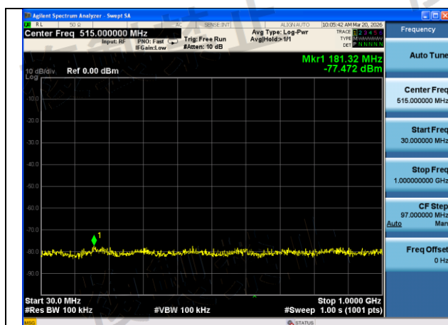
Mode:802.11n HT40 Frequency:5510MHz Ant:Chain1 scope:30MHz~1GHz
