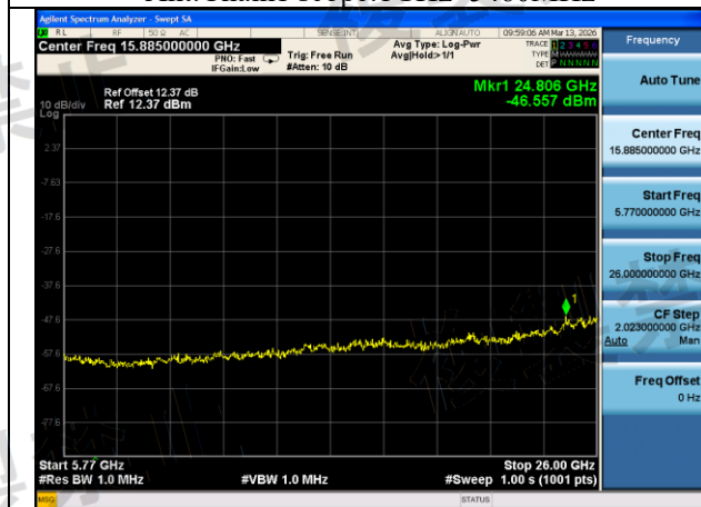
Mode:802.11ac VHT40 Frequency:5630MHz Ant:Chain1 scope:5770MHz~26GHz
