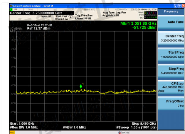
Mode:802.11ax HE20 Frequency:5500MHz Ant:Chain1 scope:1GHz~5460MHz
