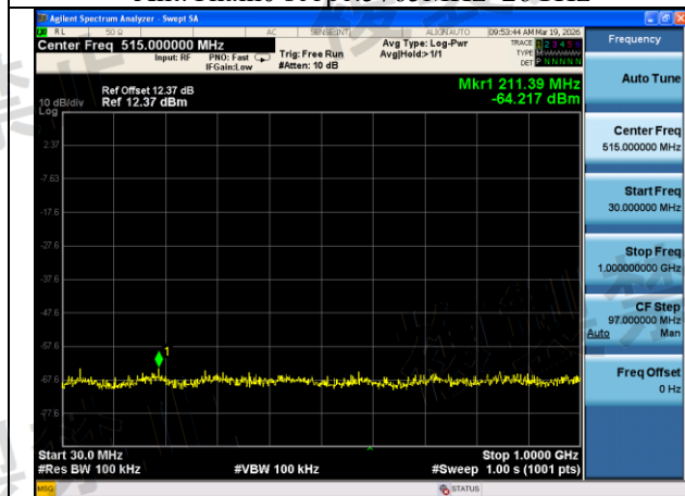
Mode:802.11ax HE20 Frequency:5620MHz Ant:Chain1 scope:30MHz~1GHz
