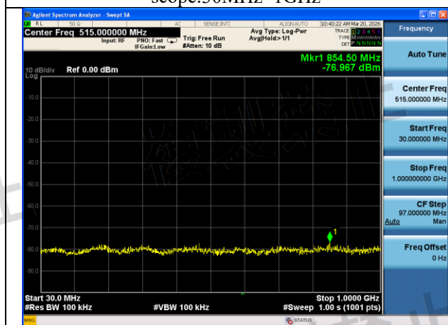
Mode:802.11n HT20 Frequency:5720MHz Ant:Chain0 scope:30MHz~1GHz
