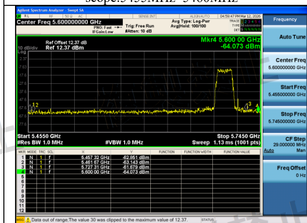
Mode:802.11n HT20 Frequency:5720MHz Ant:Chain0 scope:5455MHz~5460MHz
