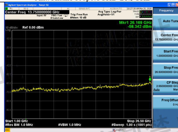
Mode:802.11ac VHT80 Frequency:5690MHz Ant:Chain1 scope:1GHz~26.5GHz
