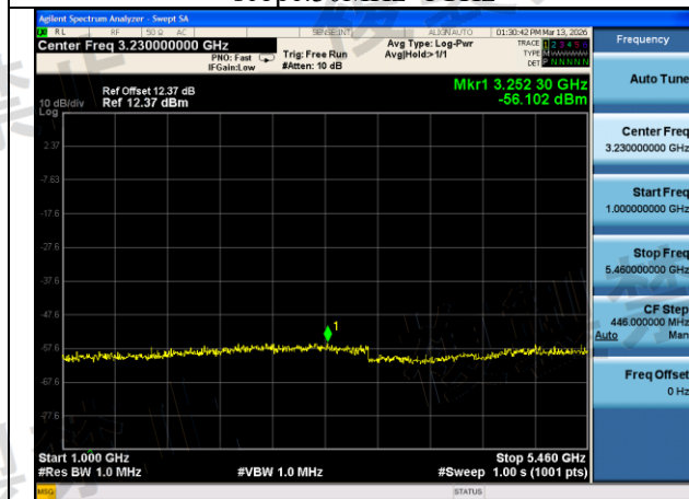
Mode:802.11n HT20 Frequency:5620MHz Ant:Chain0 scope:1GHz~5460MHz
