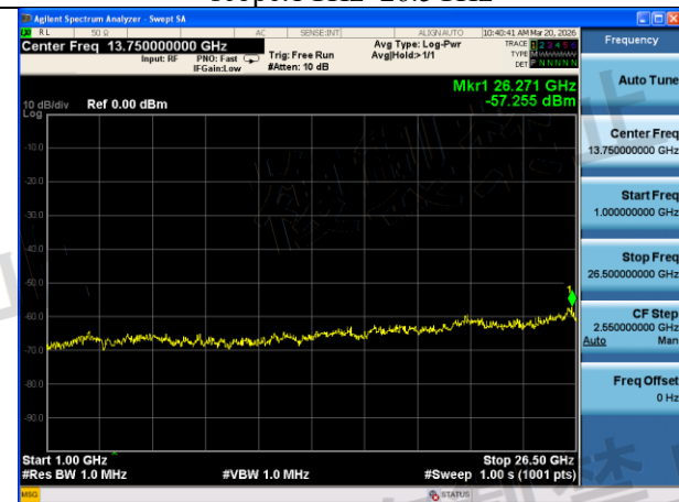
Mode:802.11n HT20 Frequency:5720MHz Ant:Chain0 scope:1GHz~26.5GHz
