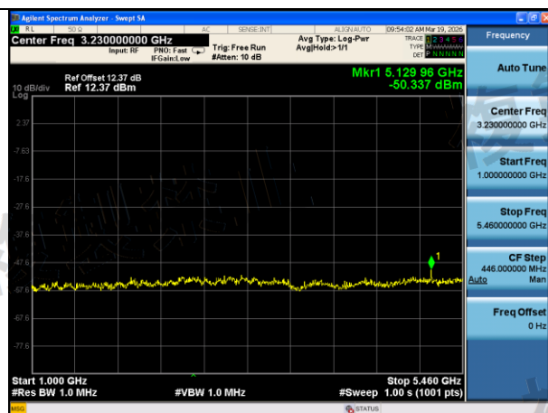
Mode:802.11ax HE20 Frequency:5620MHz Ant:Chain1 scope:1GHz~5460MHz
