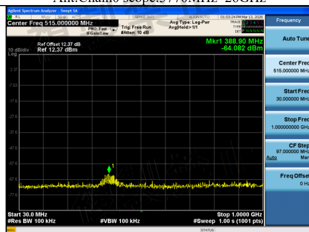
Mode:802.11ax HE40 Frequency:5510MHz Ant:Chain1 scope:30MHz~1GHz
