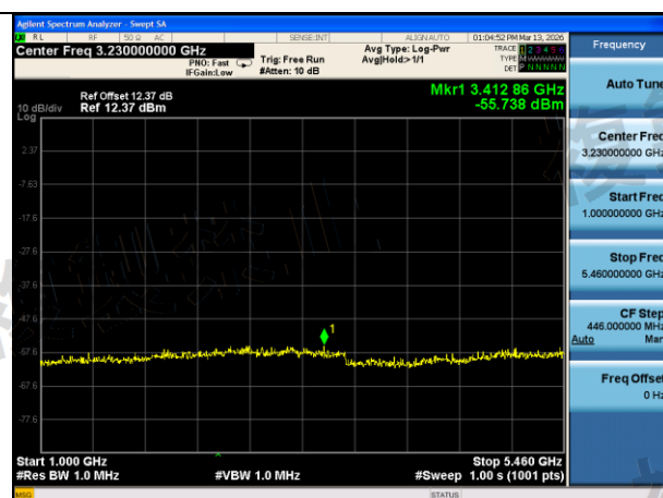
Mode:802.11ax HE40 Frequency:5630MHz Ant:Chain1 scope:1GHz~5460MHz
