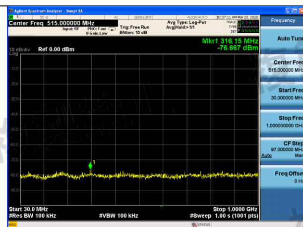
Mode:802.11ac VHT40 Frequency:5630MHz Ant:Chain0 scope:30MHz~1GHz
