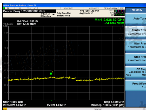
Mode:802.11ac VHT40 Frequency:5630MHz Ant:Chain1 scope:1GHz~5460MHz
