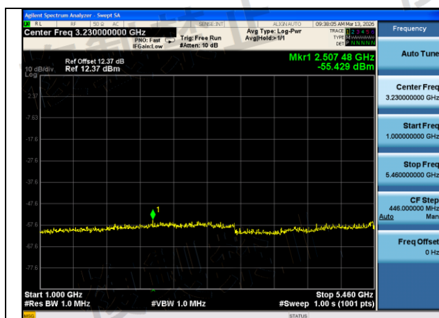
Mode:802.11n HT40 Frequency:5510MHz Ant:Chain1 scope:1GHz~5460MHz
