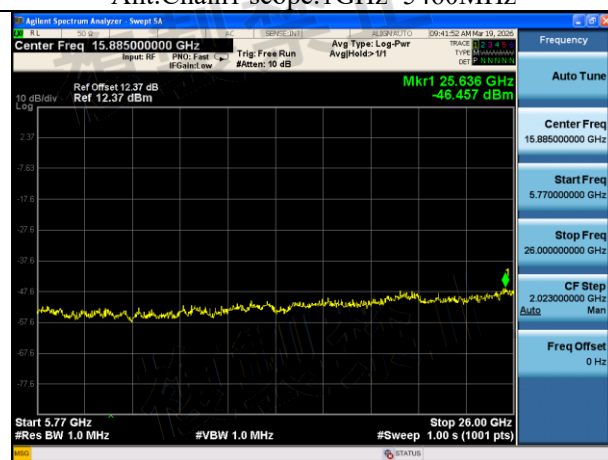
Mode:802.11ax HE80 Frequency:5530MHz Ant:Chain1 scope:5770MHz~26GHz
