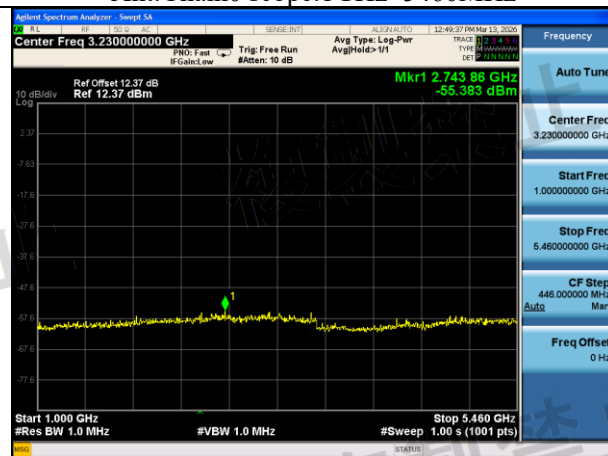
Mode:802.11ax HE40 Frequency:5710MHz Ant:Chain0 scope:1GHz~5460MHz
