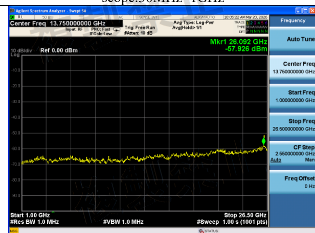
Mode:802.11n HT20 Frequency:5500MHz Ant:Chain1 scope:1GHz~26.5GHz
