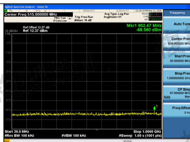
Mode:802.11ac VHT20 Frequency:5620MHz Ant:Chain0 scope:30MHz~1GHz
