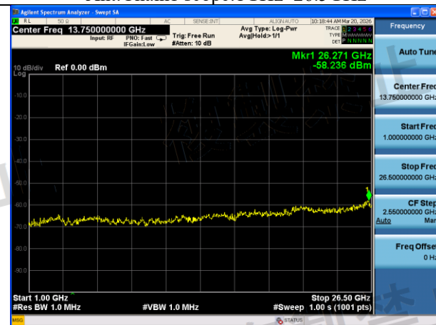
Mode:802.11ac VHT40 Frequency:5710MHz Ant:Chain1 scope:1GHz~26.5GHz
