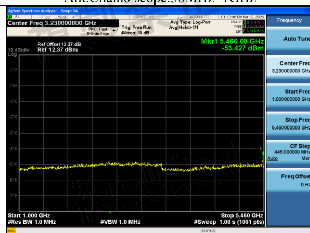
Mode:802.11ax HE80 Frequency:5530MHz Ant:Chain0 scope:1GHz~5460MHz
