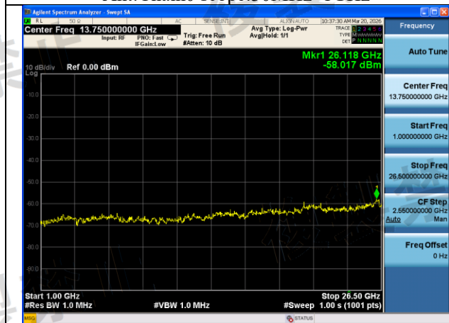
Mode:802.11ac VHT40 Frequency:5630MHz Ant:Chain0 scope:1GHz~26.5GHz
