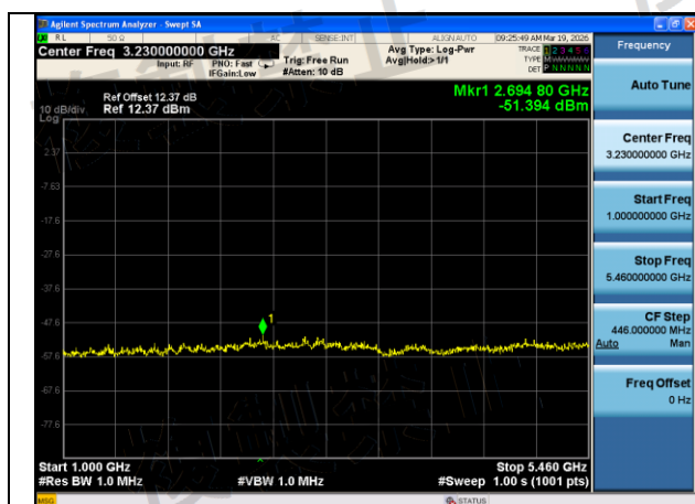
Mode:802.11n HT20 Frequency:5500MHz Ant:Chain1 scope:1GHz~5460MHz
