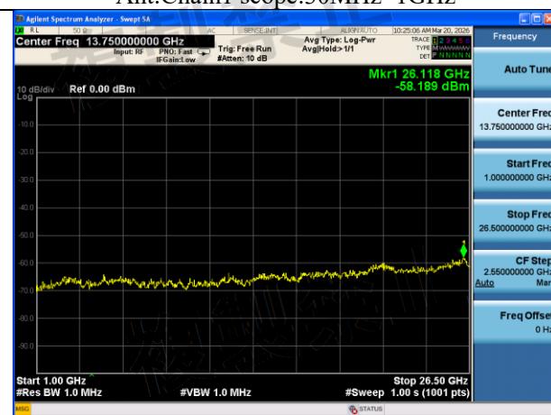
Mode:802.11ac VHT80 Frequency:5530MHz Ant:Chain1 scope:1GHz~26.5GHz
