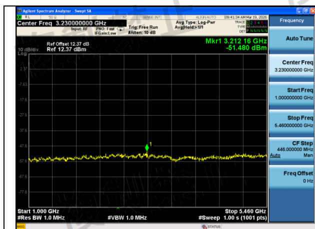
Mode:802.11ax HE80 Frequency:5530MHz Ant:Chain1 scope:1GHz~5460MHz
