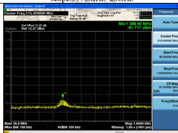
Mode:802.11n HT40 Frequency:5510MHz Ant:Chain1 scope:30MHz~1GHz
