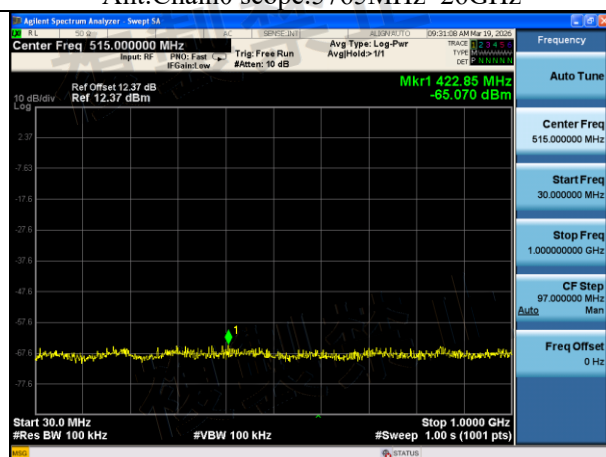
Mode:802.11ac VHT20 Frequency:5500MHz Ant:Chain1 scope:30MHz~1GHz
