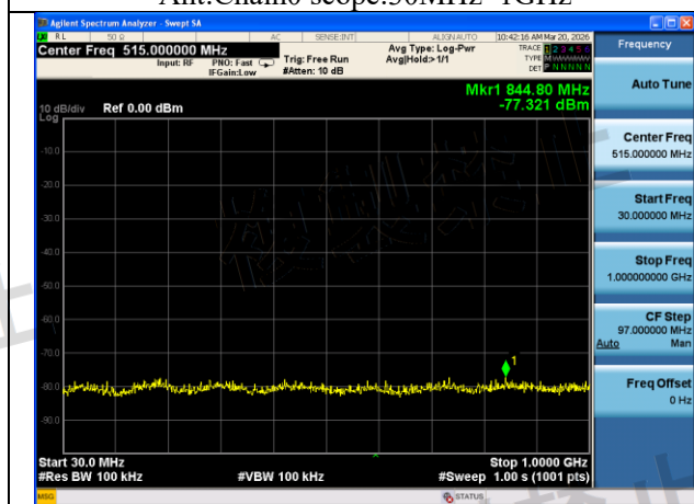
Mode:802.11ac VHT40 Frequency:5710MHz Ant:Chain0 scope:30MHz~1GHz
