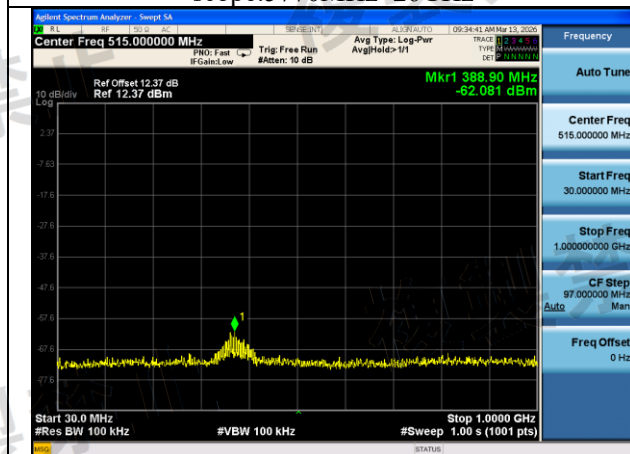
Mode:802.11n HT40 Frequency:5630MHz Ant:Chain1 scope:30MHz~1GHz
