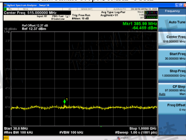
Mode:802.11ac VHT80 Frequency:5690MHz Ant:Chain1 scope:30MHz~1GHz
