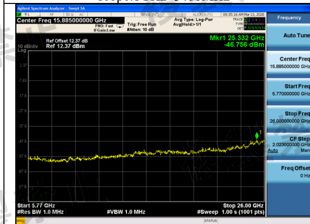
Mode:802.11n HT40 Frequency:5630MHz Ant:Chain1 scope:5770MHz~26GHz
