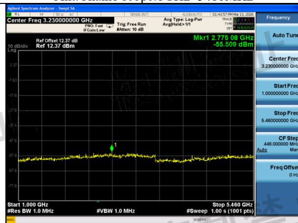
Mode:802.11ax HE80 Frequency:5690MHz Ant:Chain0 scope:1GHz~5460MHz
