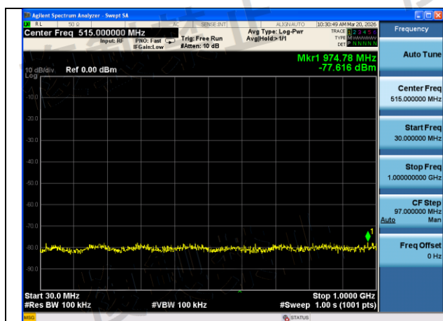
Mode:802.11n HT40 Frequency:5510MHz Ant:Chain0 scope:30MHz~1GHz
