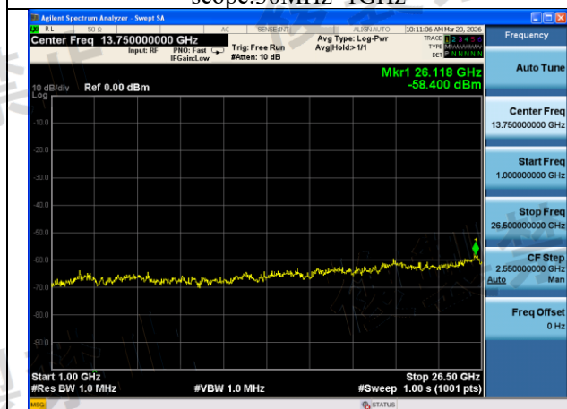
Mode:802.11n HT20 Frequency:5620MHz Ant:Chain1 scope:1GHz~26.5GHz
