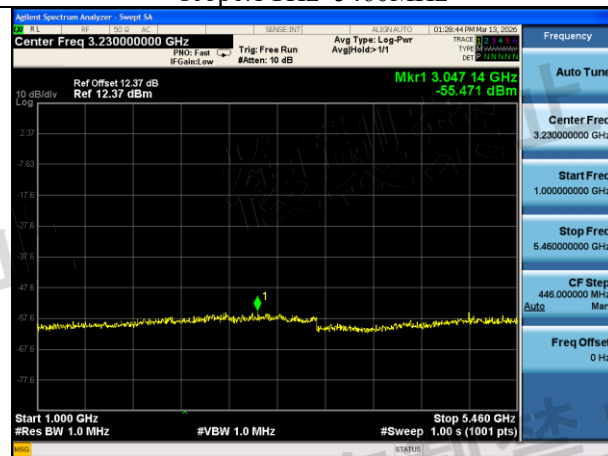
Mode:802.11n HT20 Frequency:5720MHz Ant:Chain0 scope:1GHz~5460MHz
