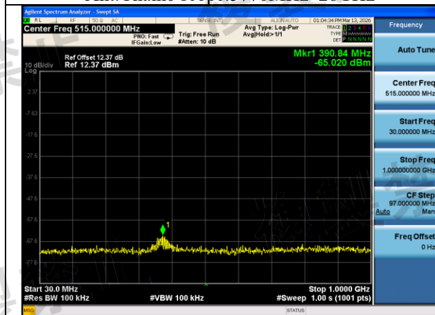
Mode:802.11ax HE40 Frequency:5630MHz Ant:Chain1 scope:30MHz~1GHz
