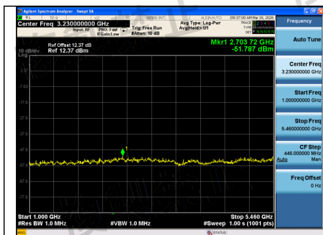
Mode:802.11ac VHT80 Frequency:5530MHz Ant:Chain1 scope:1GHz~5460MHz
