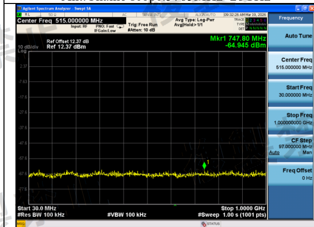
Mode:802.11ac VHT20 Frequency:5620MHz Ant:Chain1 scope:30MHz~1GHz
