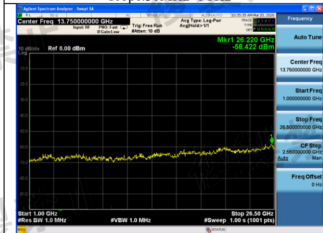
Mode:802.11n HT20 Frequency:5620MHz Ant:Chain0 scope:1GHz~26.5GHz
