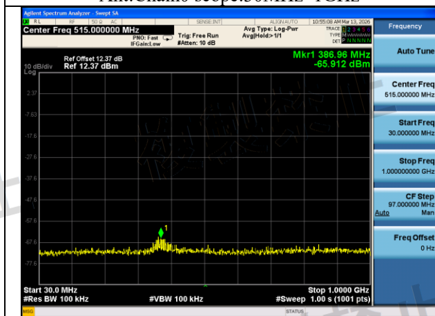
Mode:802.11ax HE20 Frequency:5720MHz Ant:Chain0 scope:30MHz~1GHz
