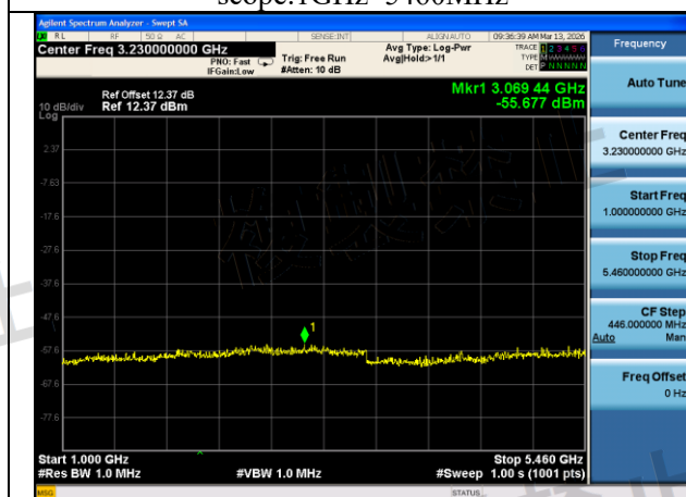
Mode:802.11n HT40 Frequency:5710MHz Ant:Chain1 scope:1GHz~5460MHz
