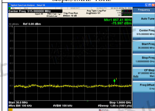
Mode:802.11n HT20 Frequency:5720MHz Ant:Chain1 scope:30MHz~1GHz
