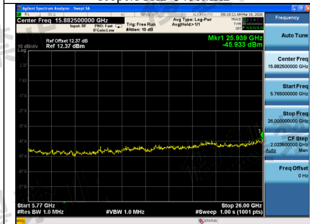
Mode:802.11a Frequency:5600MHz Ant:Chain1 scope:5765MHz~26GHz
