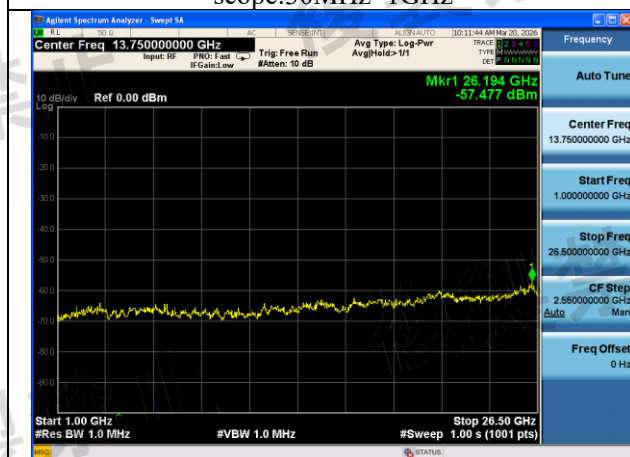
Mode:802.11n HT40 Frequency:5630MHz Ant:Chain1 scope:1GHz~26.5GHz
