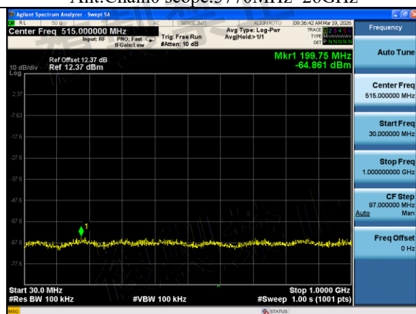
Mode:802.11ac VHT80 Frequency:5530MHz Ant:Chain1 scope:30MHz~1GHz
