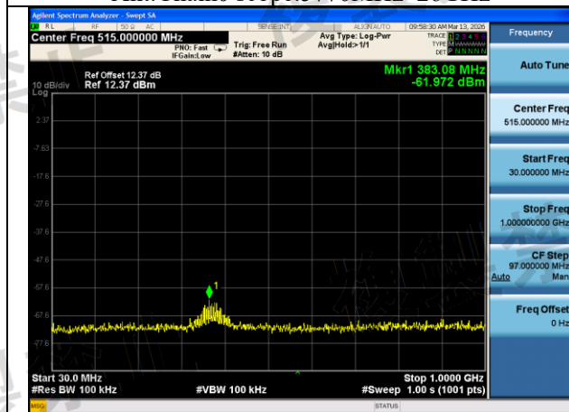
Mode:802.11ac VHT40 Frequency:5630MHz Ant:Chain1 scope:30MHz~1GHz
