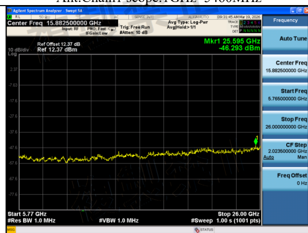
Mode:802.11ac VHT20 Frequency:5500MHz Ant:Chain1 scope:5765MHz~26GHz
