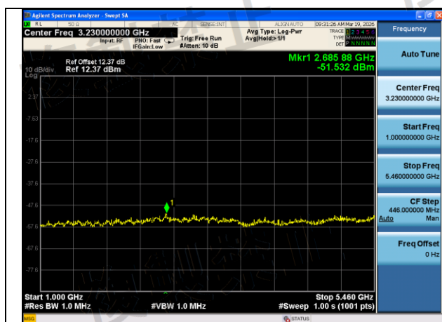
Mode:802.11ac VHT20 Frequency:5500MHz Ant:Chain1 scope:1GHz~5460MHz
