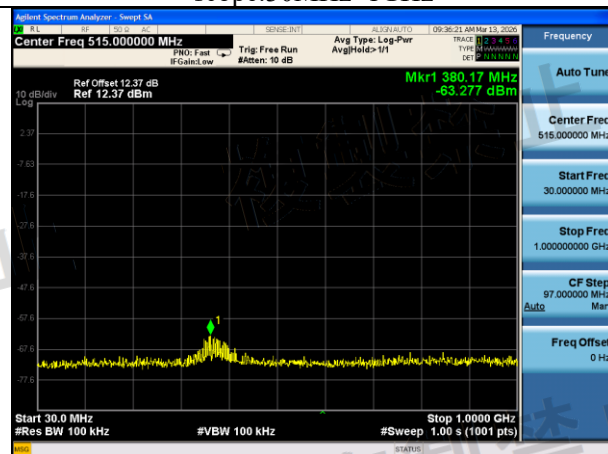
Mode:802.11n HT40 Frequency:5710MHz Ant:Chain1 scope:30MHz~1GHz
