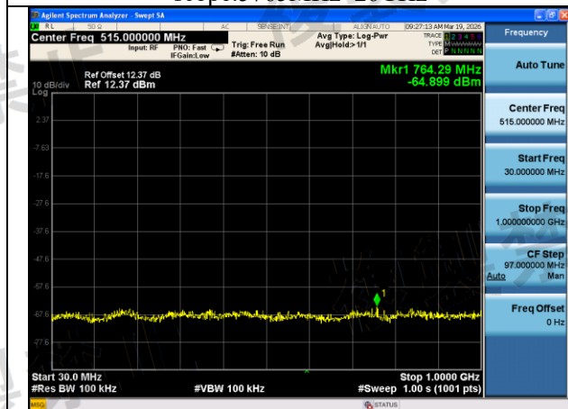
Mode:802.11n HT20 Frequency:5620MHz Ant:Chain1 scope:30MHz~1GHz
