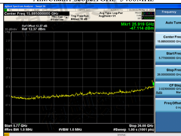
Mode:802.11ax HE40 Frequency:5510MHz Ant:Chain1 scope:5770MHz~26GHz
