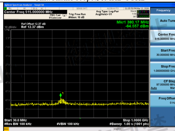
Mode:802.11ax HE40 Frequency:5710MHz Ant:Chain1 scope:30MHz~1GHz
