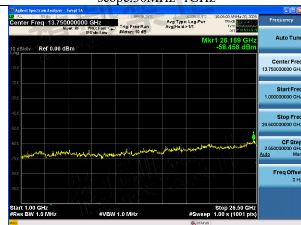
Mode:802.11n HT40 Frequency:5510MHz Ant:Chain1 scope:1GHz~26.5GHz
