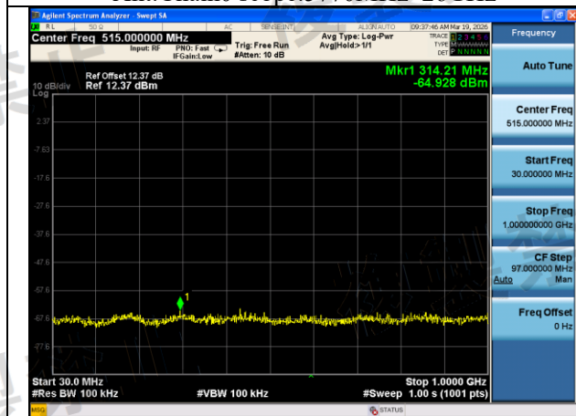
Mode:802.11ac VHT80 Frequency:5610MHz Ant:Chain1 scope:30MHz~1GHz
