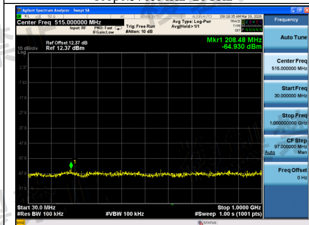
Mode:802.11a Frequency:5600MHz Ant:Chain1 scope:30MHz~1GHz
