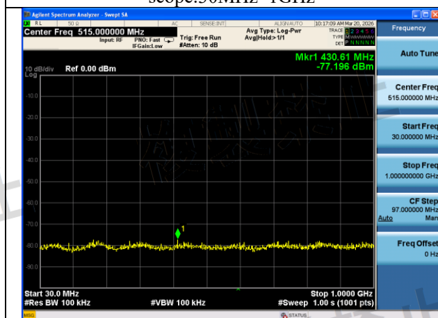
Mode:802.11n HT40 Frequency:5710MHz Ant:Chain1 scope:30MHz~1GHz
