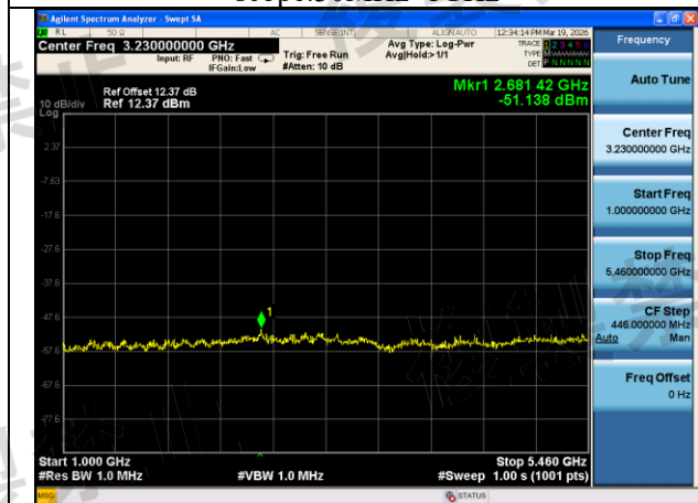
Mode:802.11n HT40 Frequency:5630MHz Ant:Chain0 scope:1GHz~5460MHz
