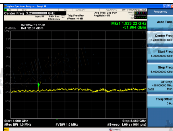
Mode:802.11ax HE80 Frequency:5610MHz Ant:Chain1 scope:1GHz~5460MHz
