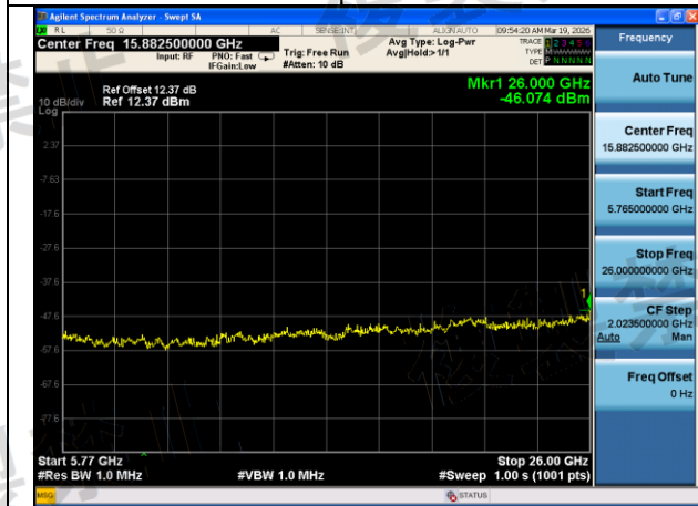
Mode:802.11ax HE20 Frequency:5620MHz Ant:Chain1 scope:5765MHz~26GHz
