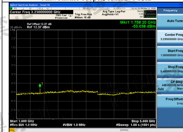
Mode:802.11ax HE20 Frequency:5620MHz Ant:Chain0 scope:1GHz~5460MHz
