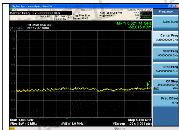
Mode:802.11a Frequency:5500MHz Ant:Chain1 scope:1GHz~5460MHz
