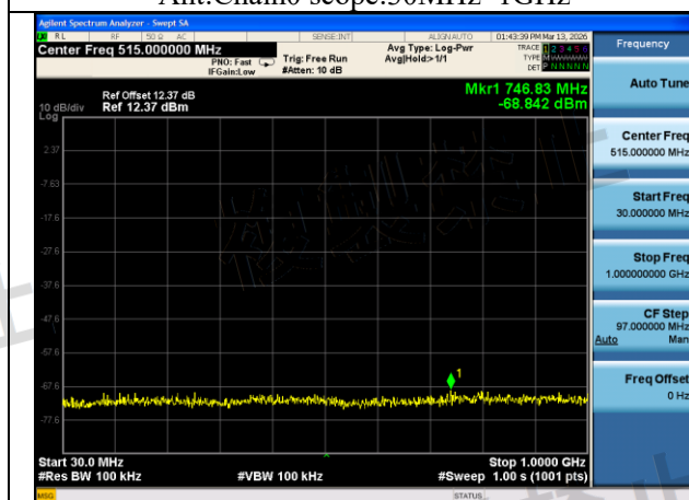
Mode:802.11ax HE80 Frequency:5690MHz Ant:Chain0 scope:30MHz~1GHz
