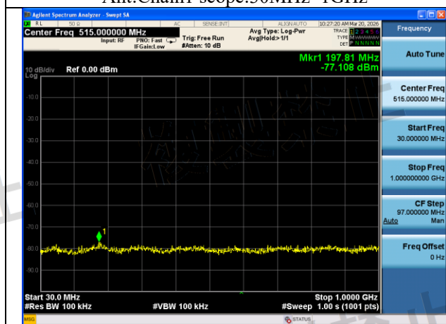
Mode:802.11ac VHT80 Frequency:5690MHz Ant:Chain1 scope:30MHz~1GHz
