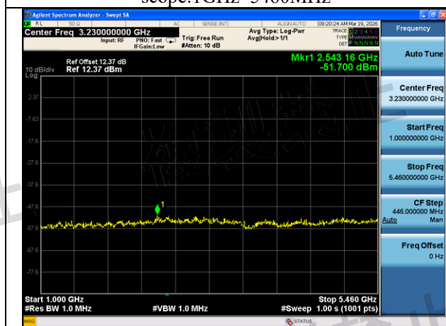
Mode:802.11a Frequency:5720MHz Ant:Chain1 scope:1GHz~5460MHz
