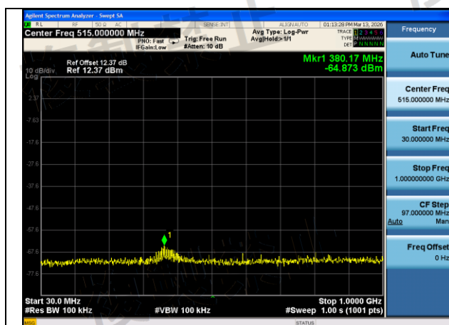
Mode:802.11ax HE80 Frequency:5530MHz Ant:Chain0 scope:30MHz~1GHz
