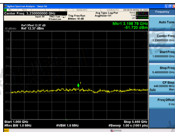
Mode:802.11ac VHT80 Frequency:5610MHz Ant:Chain1 scope:1GHz~5460MHz
