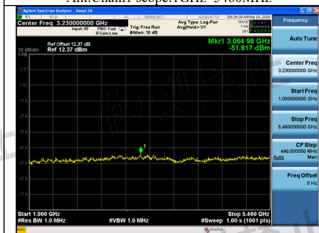
Mode:802.11ac VHT20 Frequency:5720MHz Ant:Chain1 scope:1GHz~5460MHz
