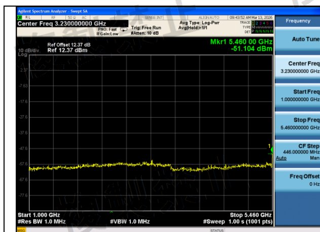
Mode:802.11ac VHT40 Frequency:5510MHz Ant:Chain1 scope:1GHz~5460MHz
