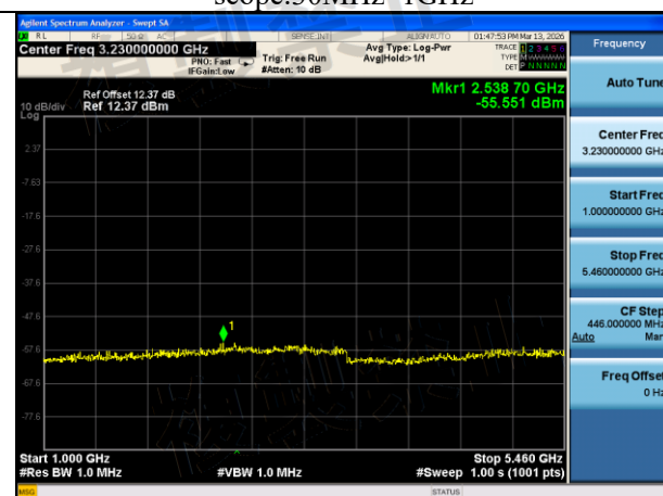
Mode:802.11n HT40 Frequency:5510MHz Ant:Chain0 scope:1GHz~5460MHz
