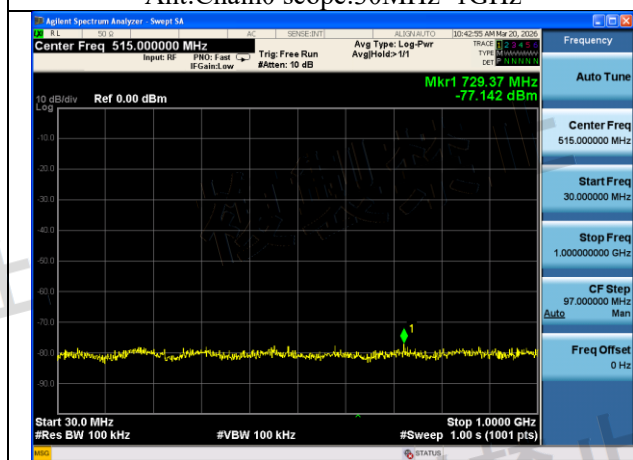
Mode:802.11ac VHT80 Frequency:5690MHz Ant:Chain0 scope:30MHz~1GHz
