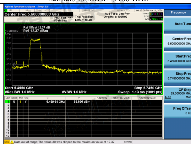
Mode:802.11n HT20 Frequency:5500MHz Ant:Chain1 scope:5455MHz~5460MHz
