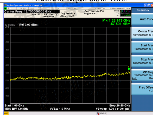
Mode:802.11ac VHT80 Frequency:5530MHz Ant:Chain0 scope:1GHz~26.5GHz
