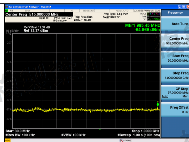
Mode:802.11n HT40 Frequency:5630MHz Ant:Chain0 scope:30MHz~1GHz
