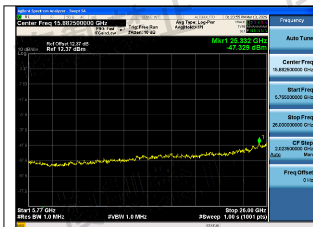
Mode:802.11a Frequency:5500MHz Ant:Chain0 scope:5765MHz~26GHz
