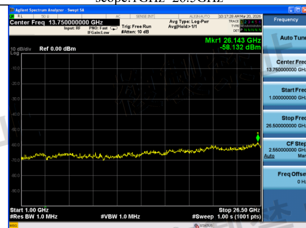
Mode:802.11n HT40 Frequency:5710MHz Ant:Chain1 scope:1GHz~26.5GHz
