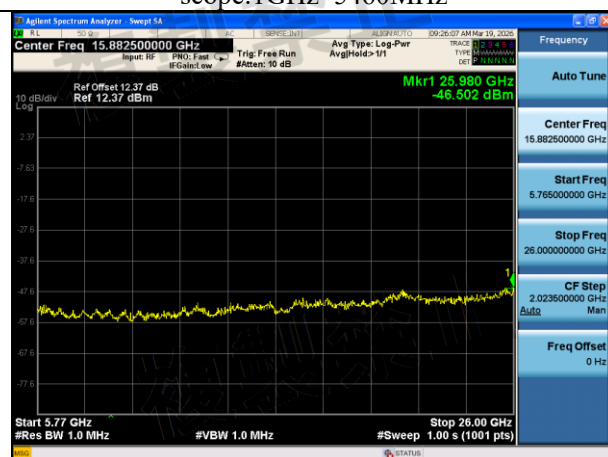
Mode:802.11n HT20 Frequency:5500MHz Ant:Chain1 scope:5765MHz~26GHz
