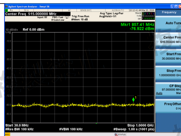
Mode:802.11ac VHT40 Frequency:5630MHz Ant:Chain1 scope:30MHz~1GHz
