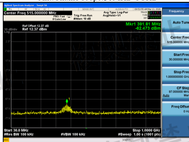
Mode:802.11ac VHT40 Frequency:5710MHz Ant:Chain1 scope:30MHz~1GHz
