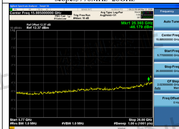
Mode:802.11n HT40 Frequency:5710MHz Ant:Chain0 scope:5770MHz~26GHz
