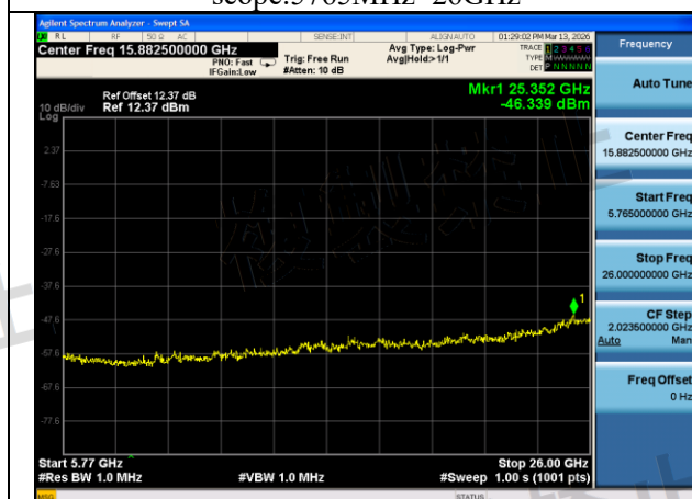
Mode:802.11n HT20 Frequency:5720MHz Ant:Chain0 scope:5765MHz~26GHz
