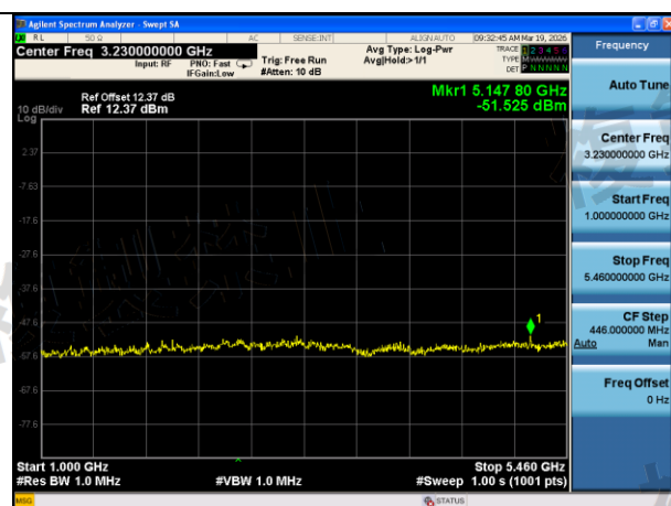
Mode:802.11ac VHT20 Frequency:5620MHz Ant:Chain1 scope:1GHz~5460MHz
