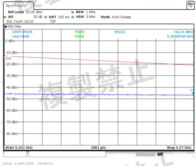
NTNV-11AC40MIMO-Ant1-5190-5251~5270-PASS
