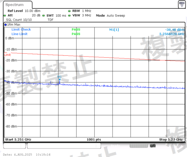
NTNV-11N40MIMO-Ant2-5230-5251~5270-PASS
