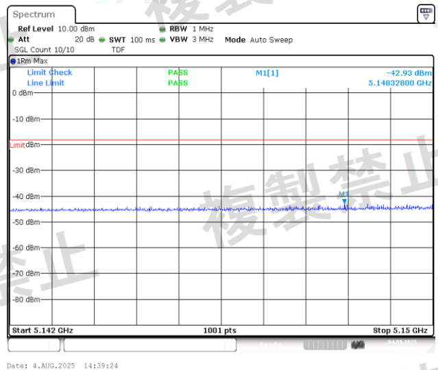
NTNV-11AC20MIMO-Ant2-5180-5142~5150-PASS
