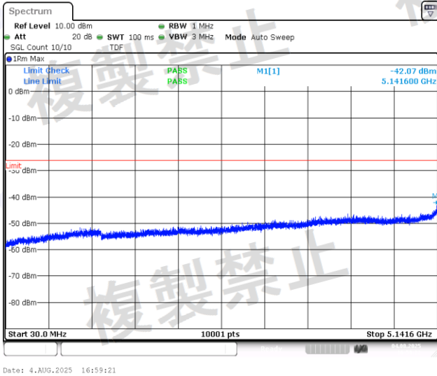
NTNV-11AC40MIMO-Ant2-5190-30~5141.6-PASS
