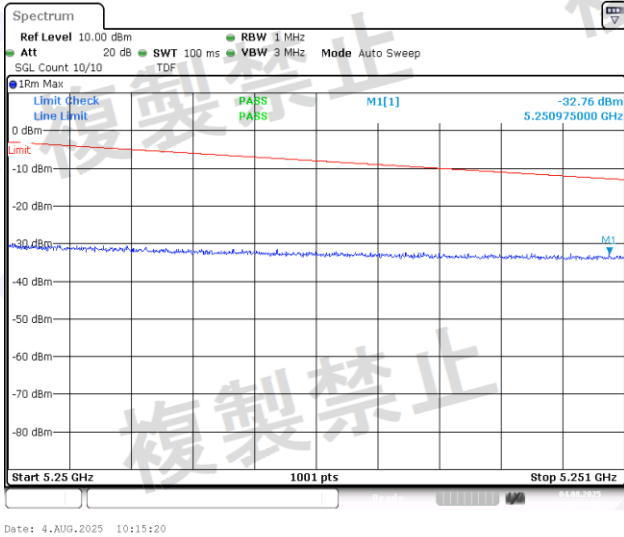
NTVN-11N40MIMO-Ant1-5230-5250~5251-PASS
