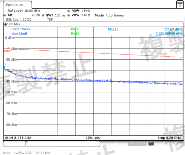
NTNV-11N20MIMO-Ant2-5240-5251~5260-PASS
