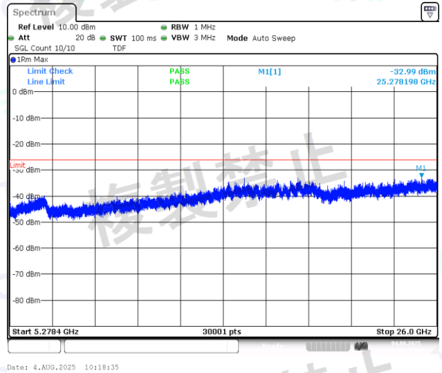
NTNV-11N40MIMO-Ant2-5230-5278.4~26000-PASS
