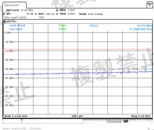
NTNV-11N40MIMO-Ant1-5190-5141.6~5150-PASS
