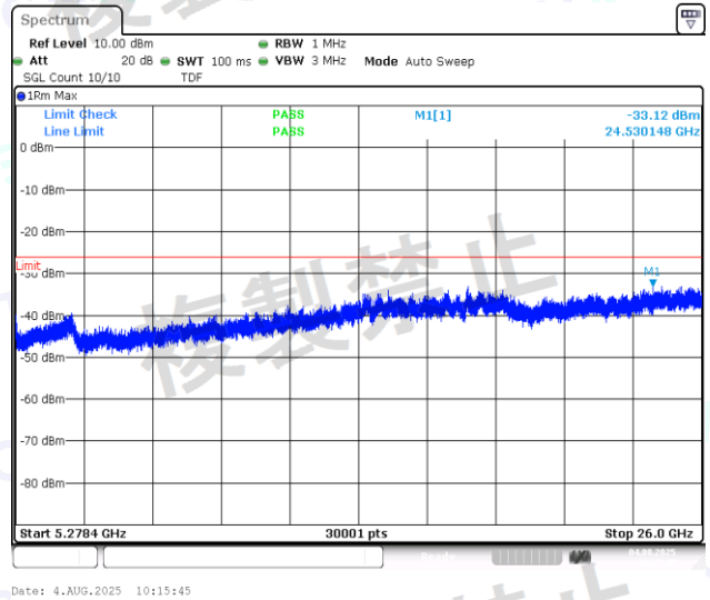
NTNV-11N40MIMO-Ant1-5230-5278.4~26000-PASS
