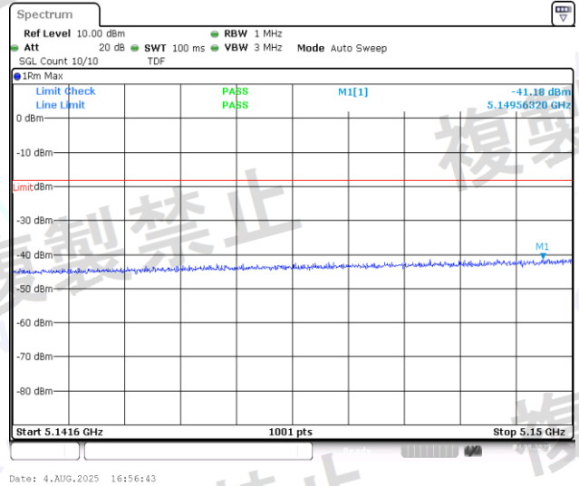
NTNV-11AC40MIMO-Ant1-5190-5141.6~5150-PASS
