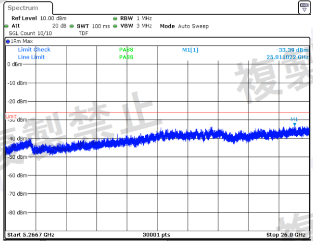
NTNV-11N20MIMO-Ant2-5200-5266.7~26000-PASS
