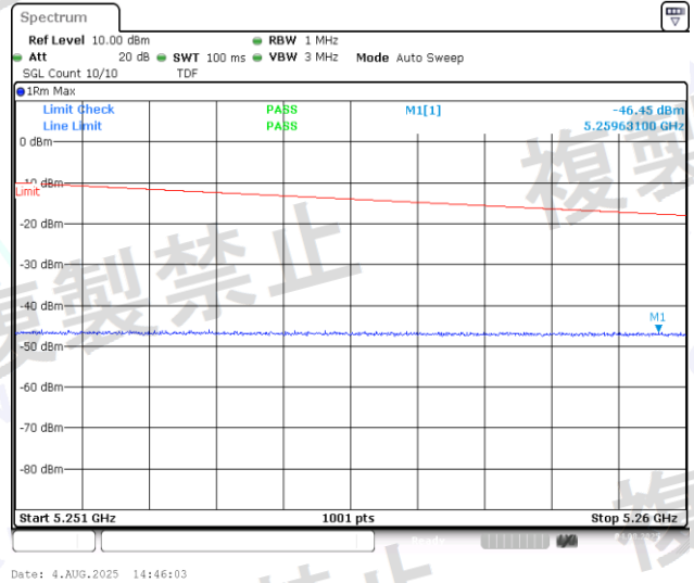
NTNV-11AC20MIMO-Ant2-5200-5251~5260-PASS
