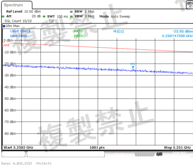
NTNV-11N20MIMO-Ant2-5240-5250.2~5251-PASS
