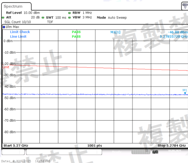
NTNV-11AC40MIMO-Ant1-5190-5270~5278.4-PASS
