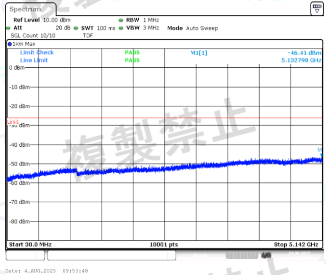
NTNV-11N20MIMO-Ant2-5240-30~5142-PASS
