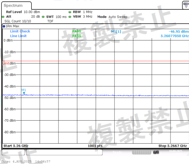
NTNV-11AC20MIMO-Ant1-5180-5260~5266.7-PASS
