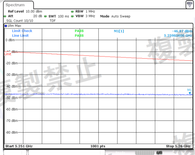
NTNV-11AC20MIMO-Ant2-5180-5251~5260-PASS
