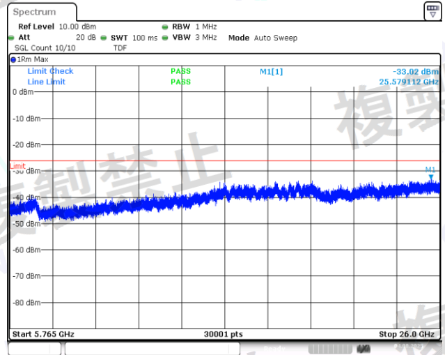
NTNV-11A-Ant2-5500-5765~26000-PASS
