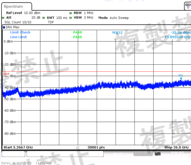
NTNV-11AC20MIMO-Ant1-5240-5266.7~26000-PASS
