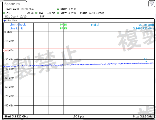
NTNV-11AC80MIMO-Ant1-5210-5132.5~5150-PASS
