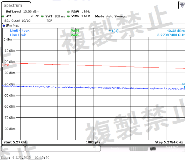
NTNV-11N40MIMO-Ant1-5230-5270~5278.4-PASS
