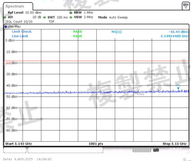
NTNV-11AC20MIMO-Ant1-5180-5142~5150-PASS
