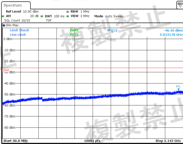
NTNV-11N20MIMO-Ant2-5200-5260~5266.7-PASS
