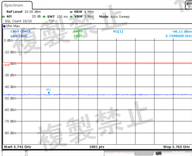
NTNV-11A-Ant2-5500-5745~5765-PASS
