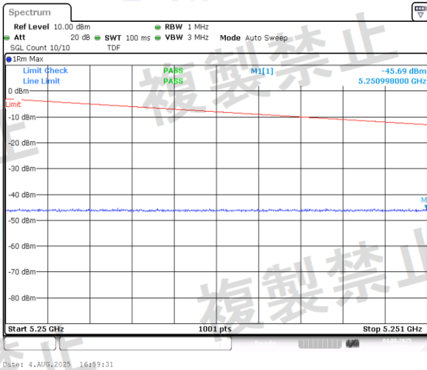
NTNV-11AC40MIMO-Ant2-5190-5250~5251-PASS
