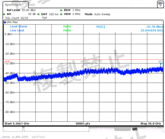
NTNV-11AC20MIMO-Ant1-5180-5266.7~26000-PASS
