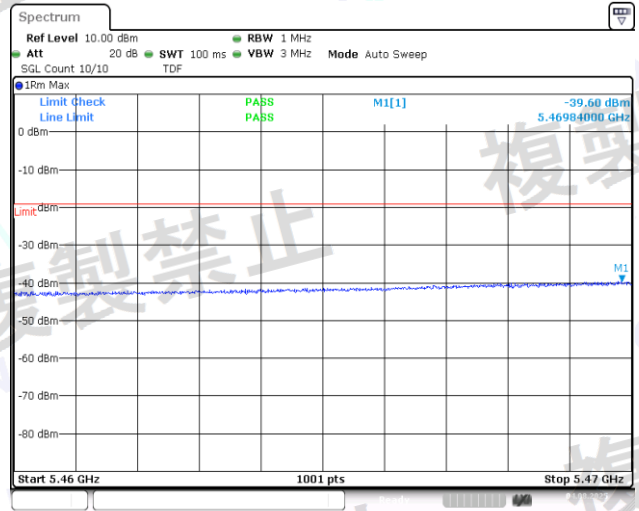
NTNV-11A-Ant1-5500-5460~5470-PASS
