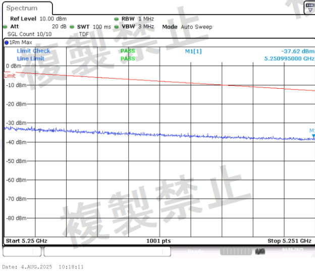
NTNV-11N40MIMO-Ant2-5230-5250~5251-PASS
