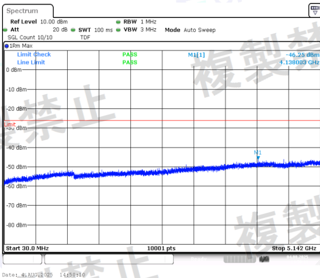
NTNV-11AC20MIMO-Ant1-5240-30~5142-PASS
