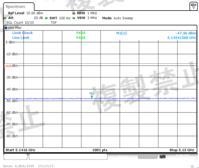
NTNV-11N40MIMO-Ant1-5230-5141.6~5150-PASS
