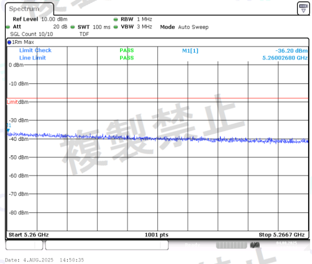
NTNV-11AC20MIMO-Ant1-5240-5260~5266.7-PASS
