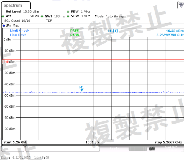
NTNV-11AC20MIMO-Ant2-5200-5260~5266.7-PASS
