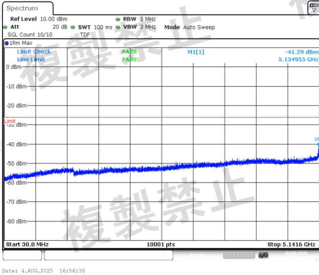
NTNV-11AC40MIMO-Ant1-5190-30~5141.6-PASS
