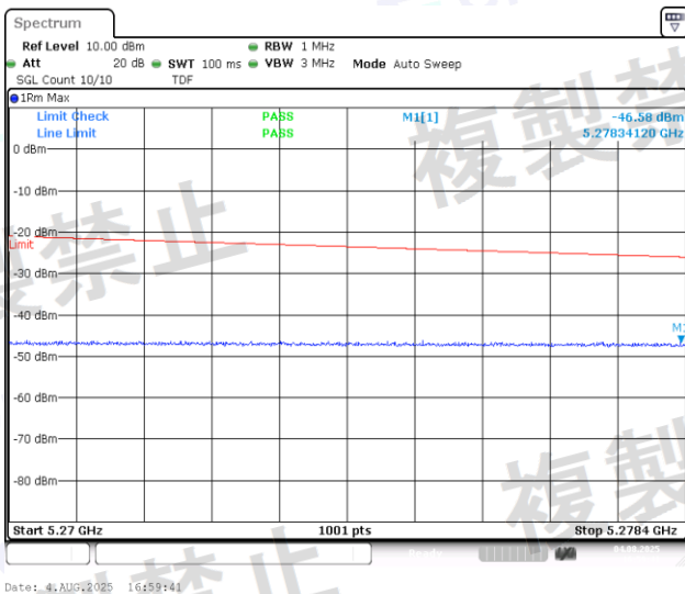
NTNV-11AC40MIMO-Ant2-5190-5270~5278.4-PASS
