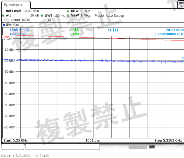
NTNV-11AC20MIMO-Ant1-5240-5250~5250.2-PASS
