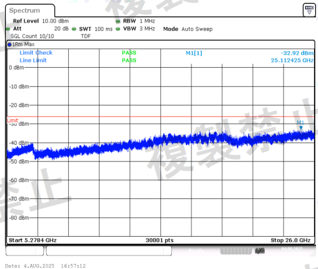
NTNV-11AC40MIMO-Ant1-5190-5278.4~26000-PASS
