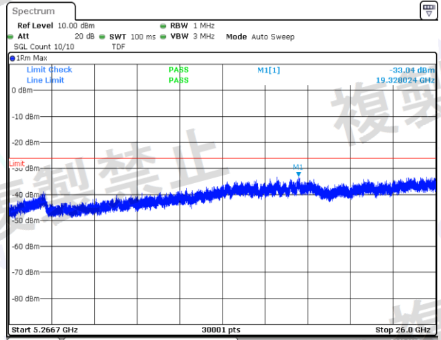
NTNV-11N20MIMO-Ant1-5200-5266.7~26000-PASS
