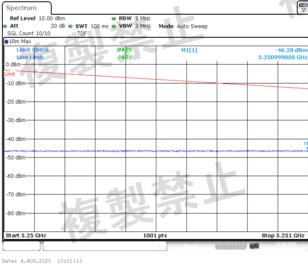
NTNV-11N40MIMO-Ant2-5190-5250~5251-PASS
