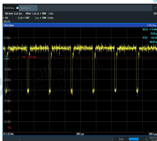
NTNV-11N40SISO-Ant2-5230-PASS
