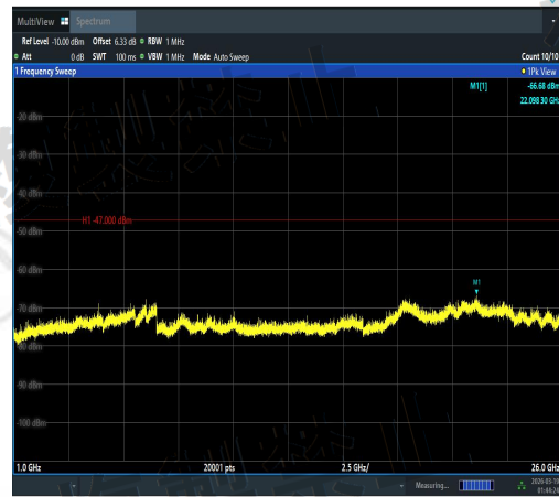
NTVN-11AX20MIMO-Ant1-5180-1000~26000-PA SS
