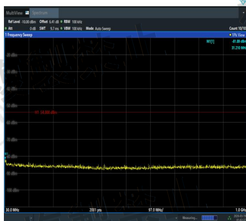
NTNV-11AC40MIMO-Ant3-5230-30~1000-PASS
