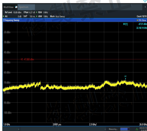
NTNV-11AC40MIMO-Ant2-5230-1000~26000-PASS
