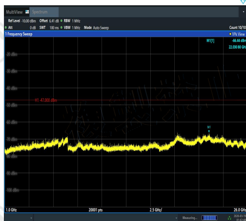
NTNV-11AC40MIMO-Ant3-5230-1000~26000-PASS
