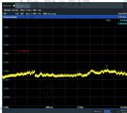
NTNV-11AX20SISO-Ant2-5180-1000~26000-PA SS
