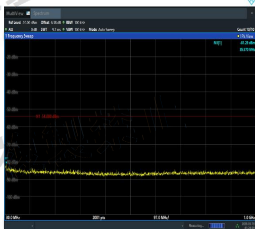
NTNV-11AX20SISO-Ant3-5180-30~1000-PASS
