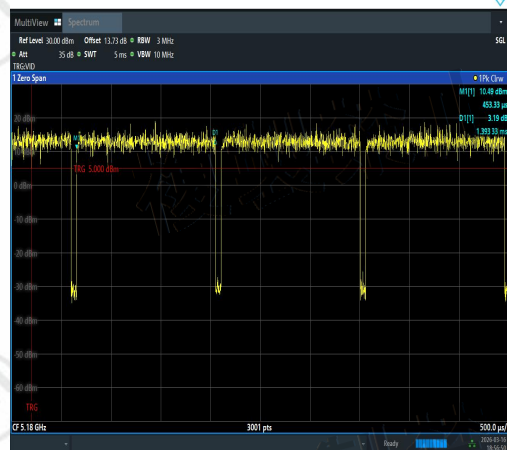
NTNV-11N20SISO-Ant2-5180-PASS
