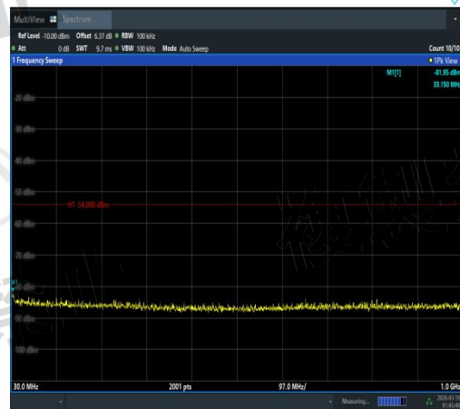
NTVN-11AX20MIMO-Ant2-5220-30~1000-PASS
