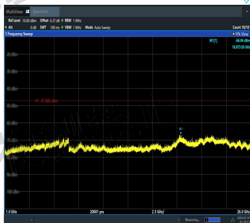
NTNV-11AC20SISO-Ant2-5220-1000~26000-PA
