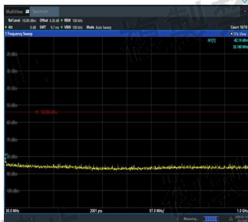
NTNV-11AX20SISO-Ant1-5220-30~1000-PASS
