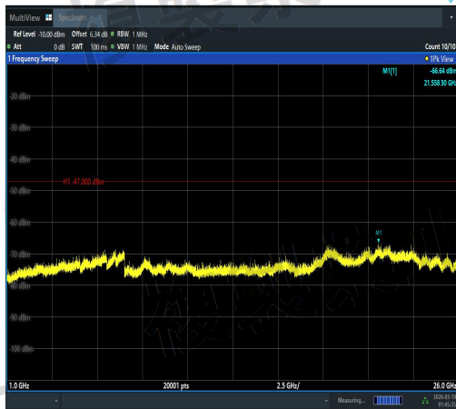
NTVN-11AX20MIMO-Ant2-5180-1000~26000-PA SS
