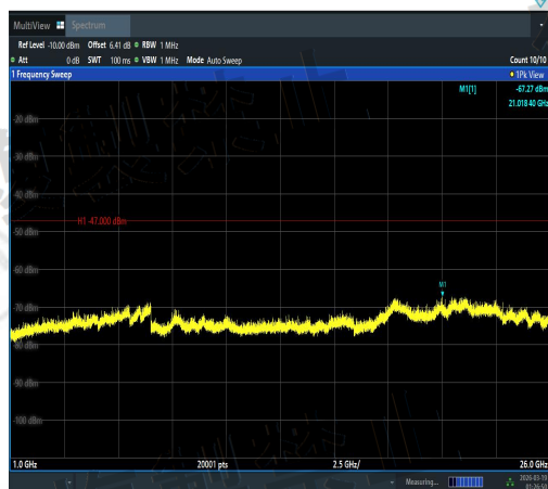
NTNV-11AC20SISO-Ant3-5220-1000~26000-PA
