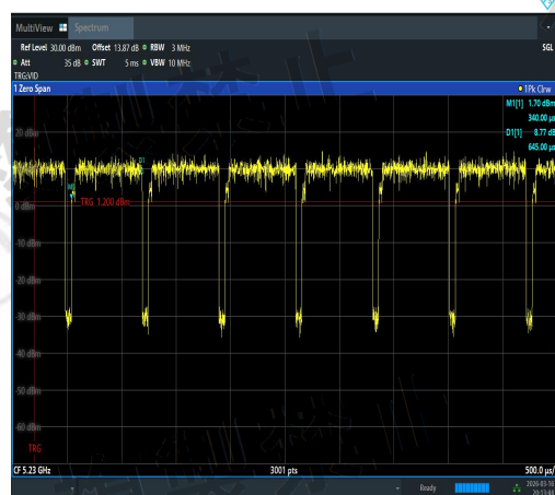
NTNV-11N40SISO-Ant3-5230-PASS
