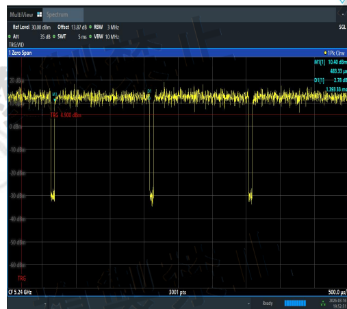
NTNV-11A-Ant3-5240-PASS
