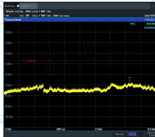
NTVN-11AX20MIMO-Ant3-5180-1000~26000-PA SS
