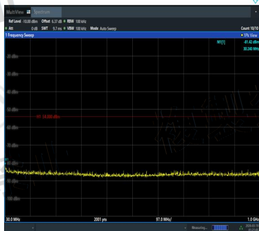
NTNV-11AX20SISO-Ant2-5220-30~1000-PASS
