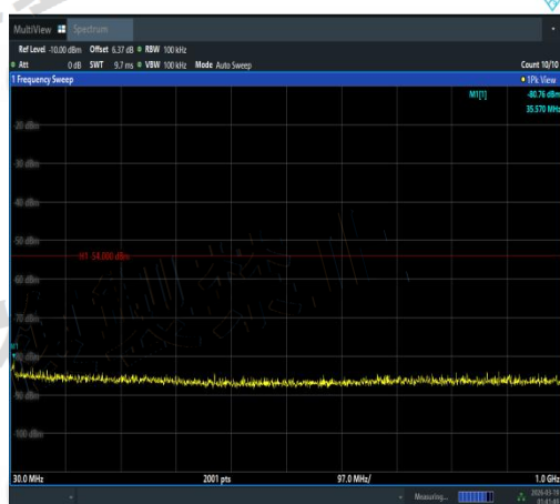
NTNV-11AC40MIMO-Ant2-5230-30~1000-PASS
