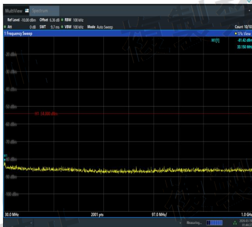
NTVN-11AX20MIMO-Ant1-5220-30~1000-PASS
