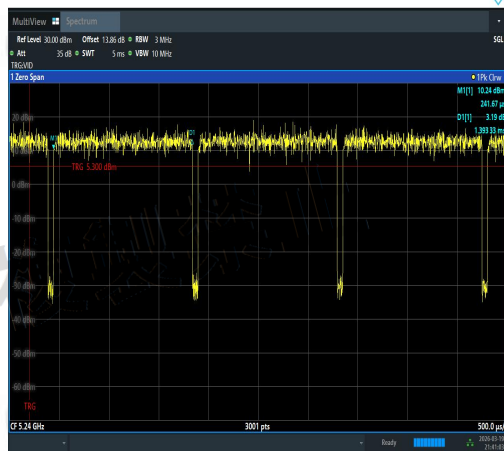
NTNV-11A-Ant2-5240-PASS
