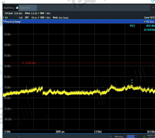
NTNV-11AC20SISO-Ant1-5240-1000~26000-PA
