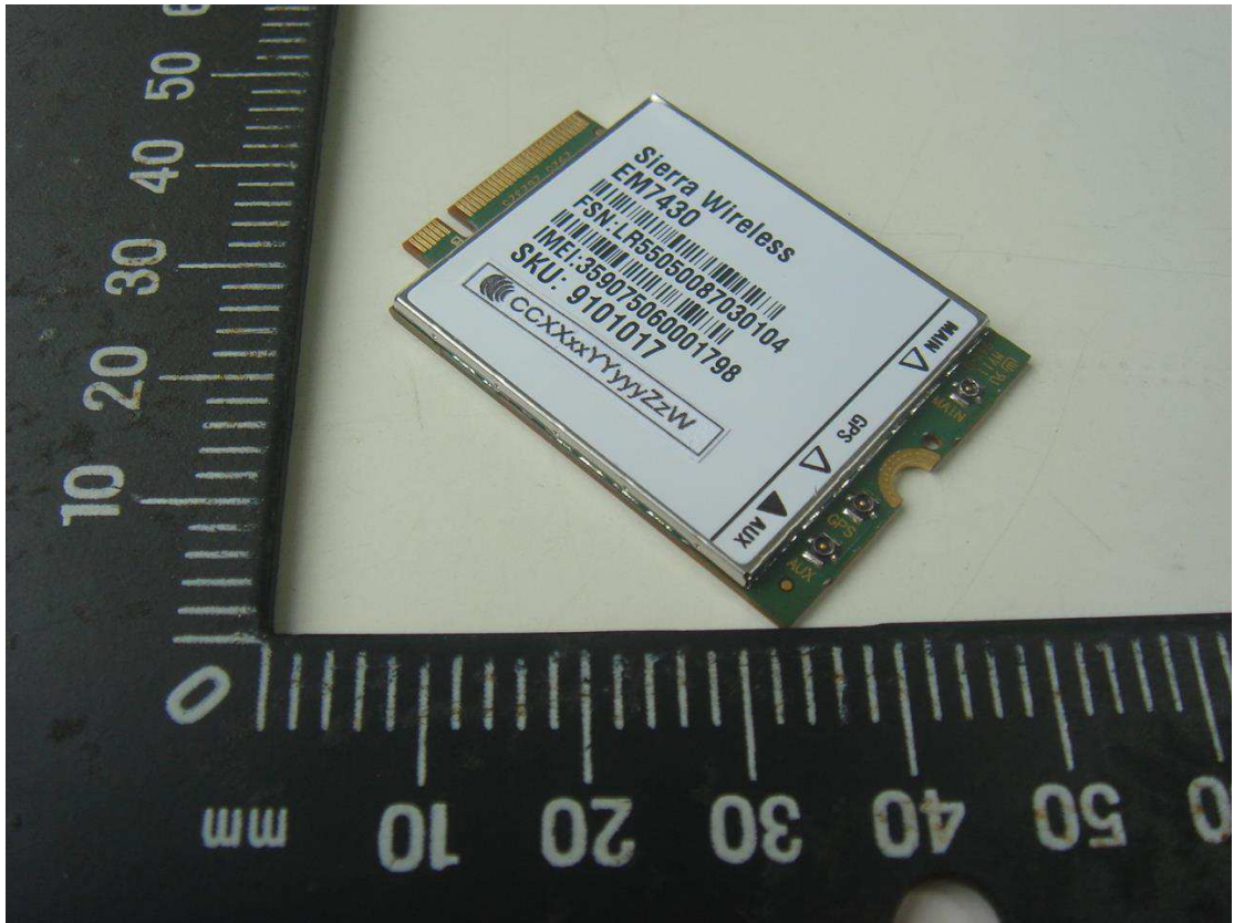
AirPrime EM7430 側面照
