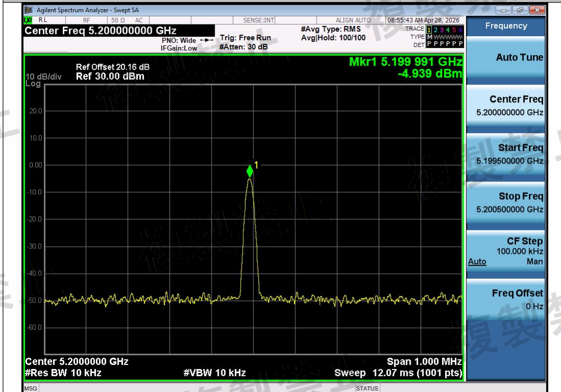
NTNV-11A-Ant1-5200-PASS
