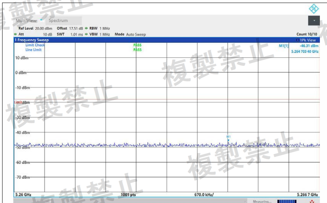
NTNV-11N20MIMO-Ant1-5180-5260~5266.7-PASS
