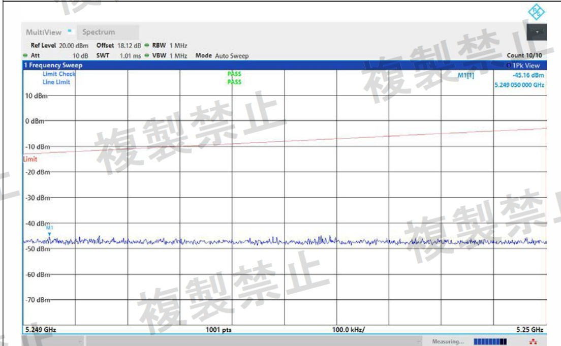
NTNV-11N40MIMO-Ant2-5310-5249~5250-PASS
