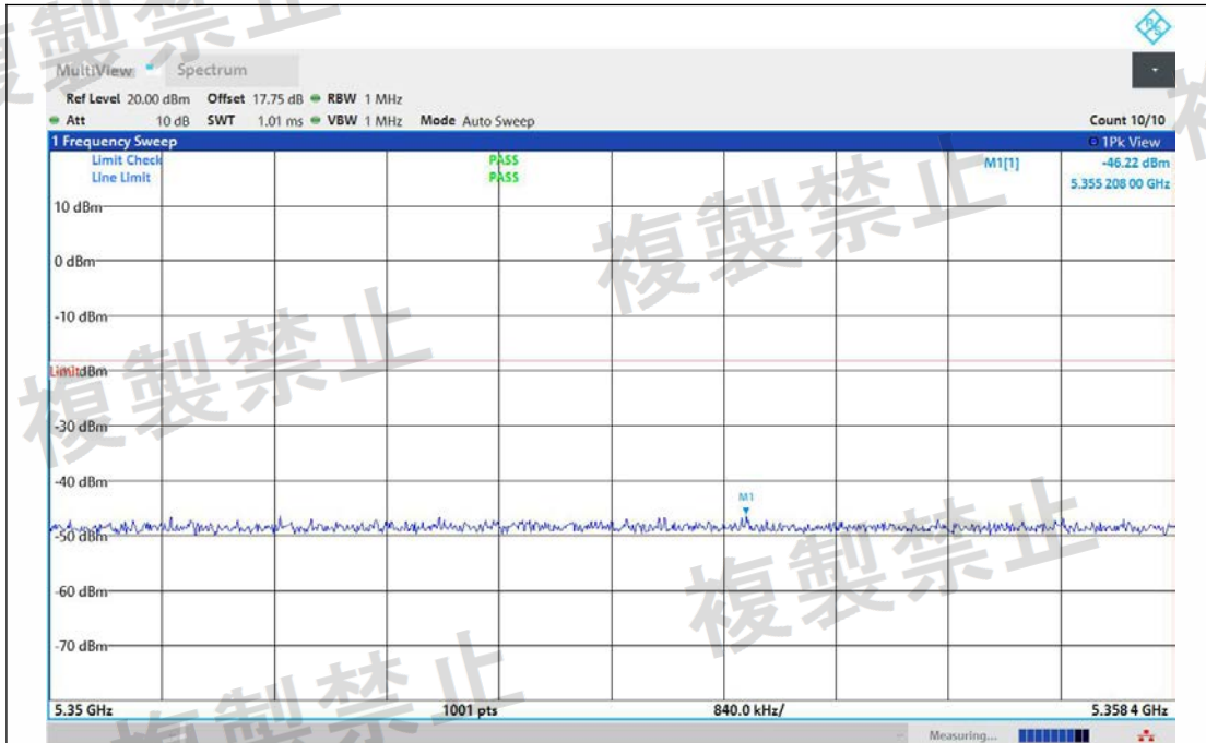
NTNV-11N40MIMO-Ant1-5270-5350~5358.4-PASS
