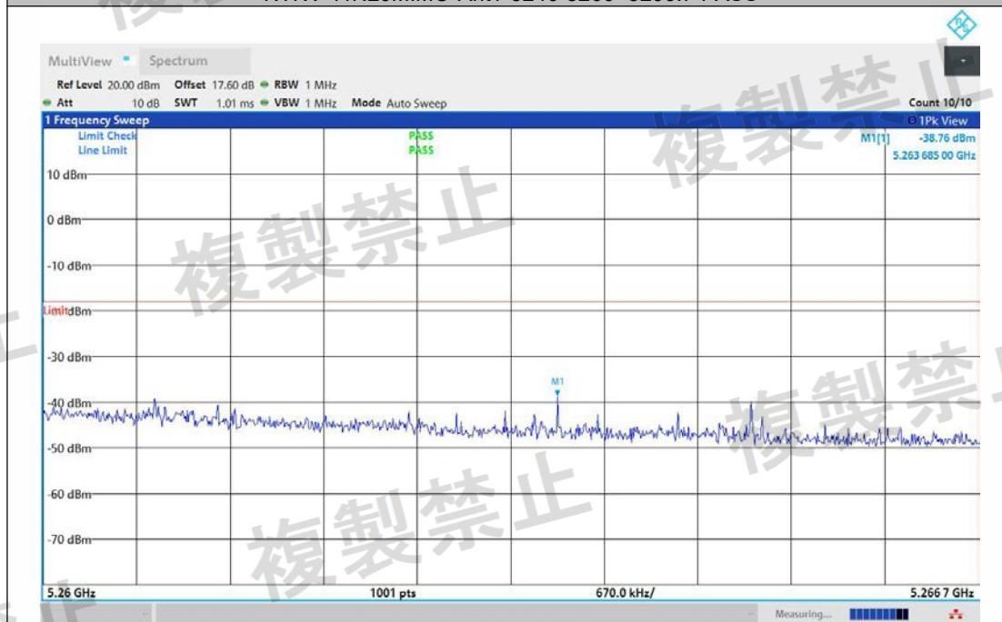
NTNV-11N20MIMO-Ant2-5240-5260~5266.7-PASS
