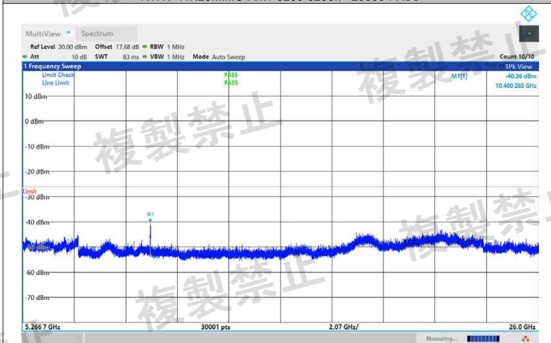
NTNV-11N20MIMO-Ant2-5200-5266.7~26000-PASS
