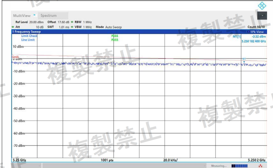
NTNV-11AC20MIMO-Ant2-5240-5250~5250.2-See table below
