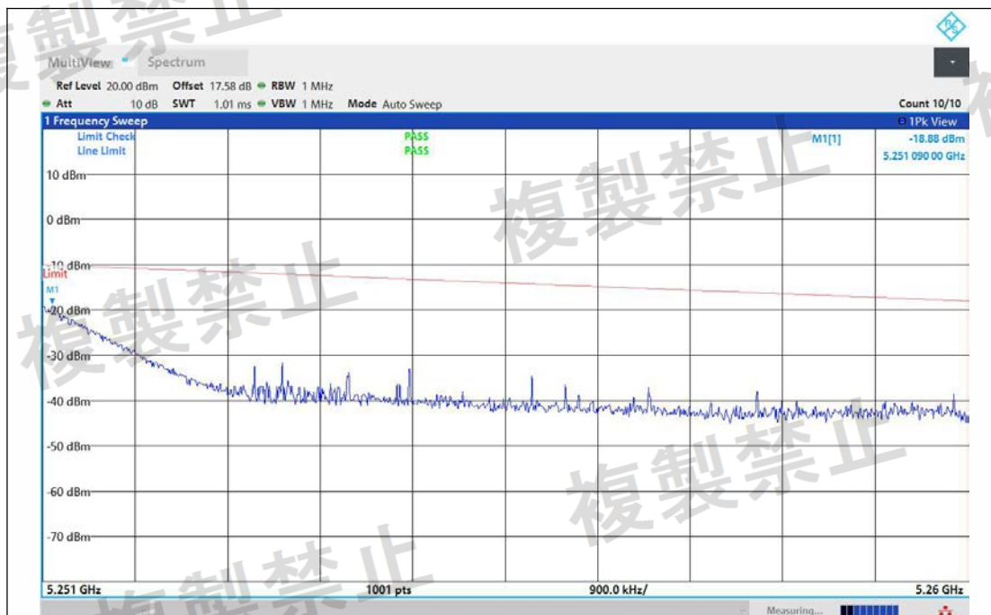
NTNV-11N20MIMO-Ant1-5240-5251~5260-PASS
