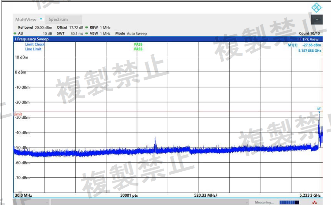
NTNV-11N20MIMO-Ant2-5260-30~5233.3-See table below
