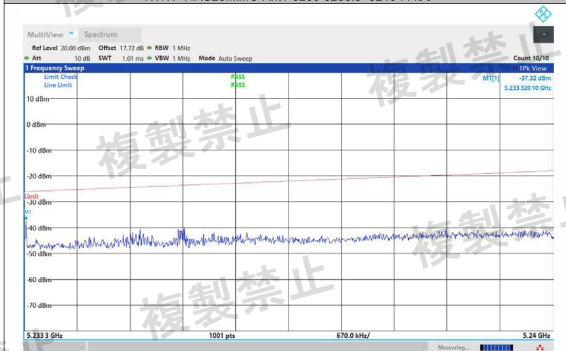
NTNV-11AC20MIMO-Ant2-5260-5233.3~5240-PASS
