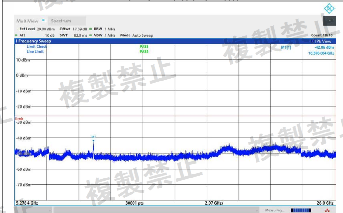
NTNV-11N40MIMO-Ant2-5190-5278.4~26000-PASS
