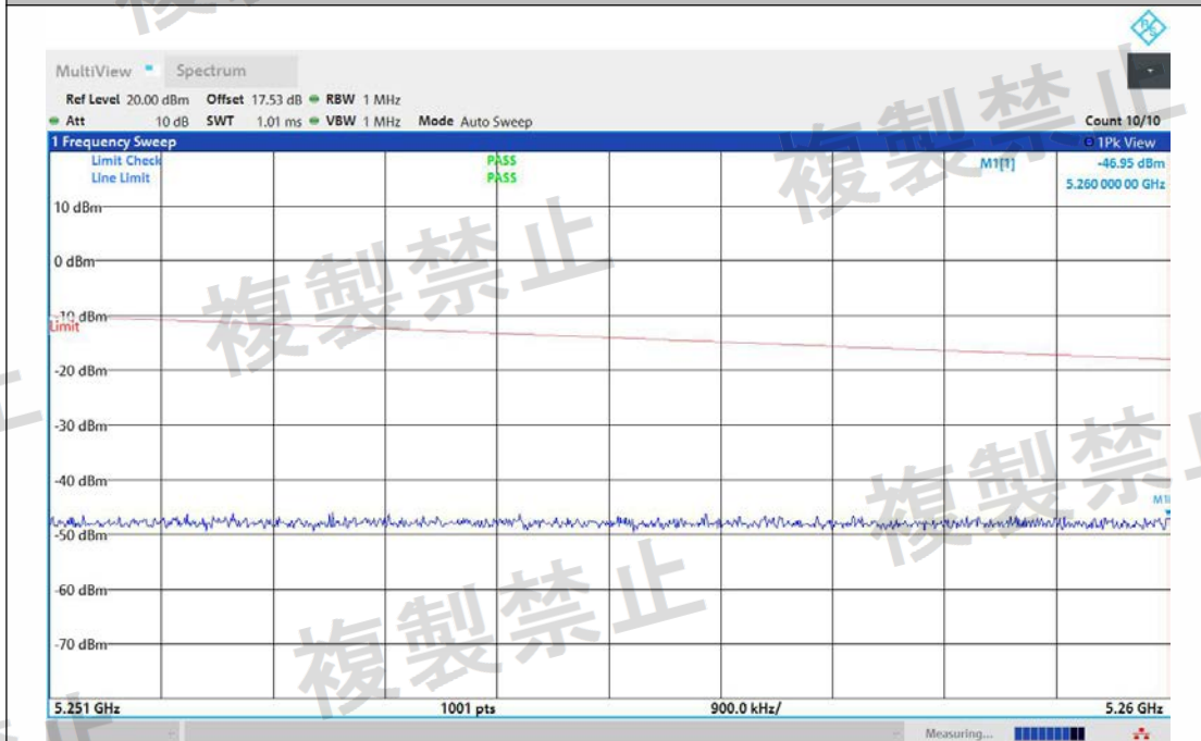
NTNV-11N20MIMO-Ant2-5180-5251~5260-PASS
