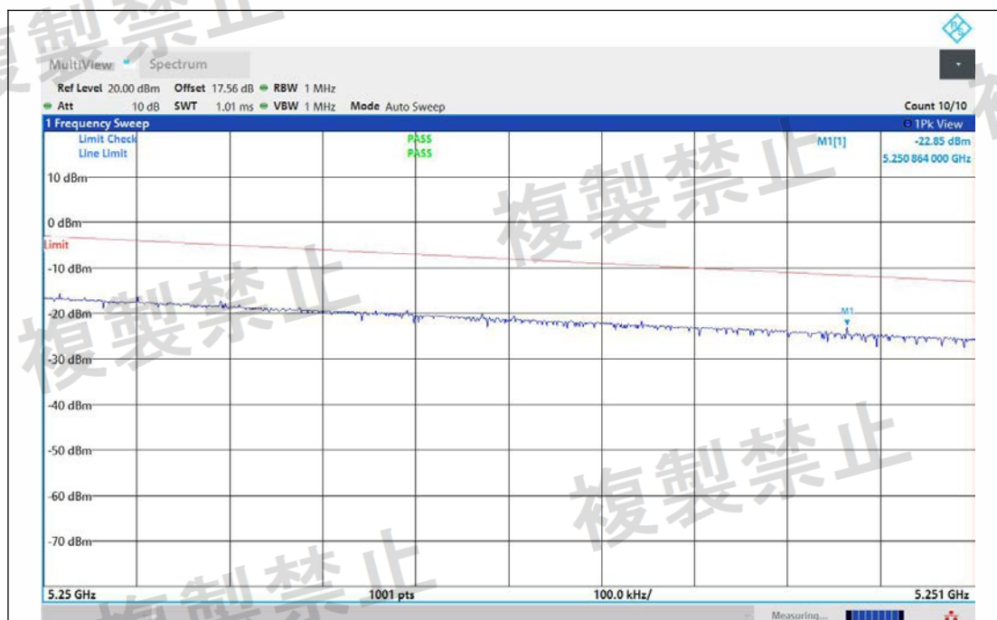
NTNV-11N40MIMO-Ant1-5230-5250~5251-PASS
