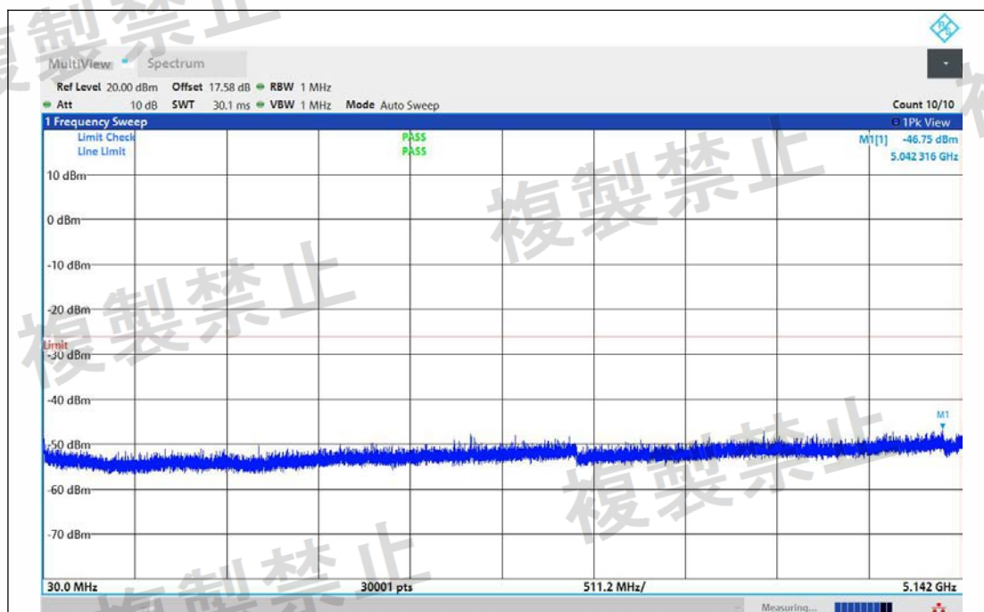
NTNV-11AC20MIMO-Ant1-5240-30~5142-PASS
