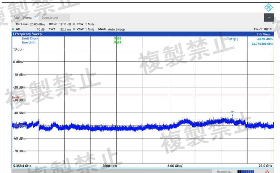
NTNV-11N40MIMO-Ant1-5310-5358.4~26000-PASS
