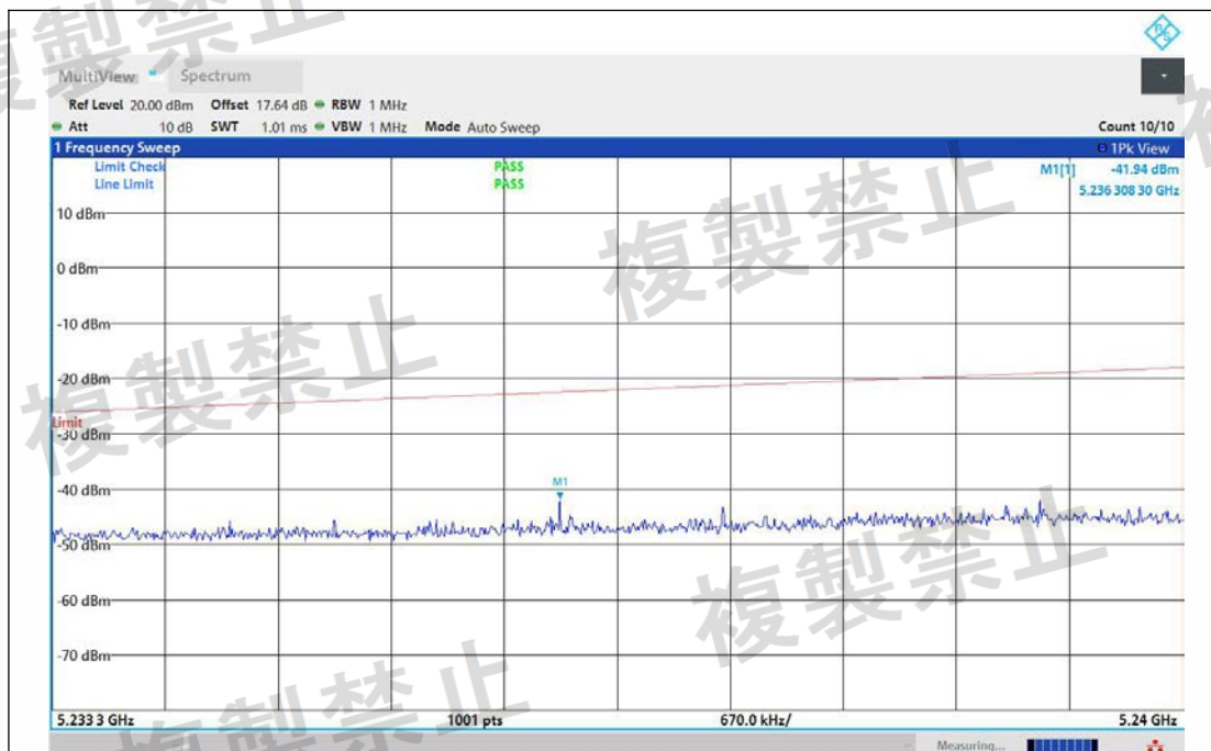
NTNV-11AC20MIMO-Ant1-5260-5233.3~5240-PASS
