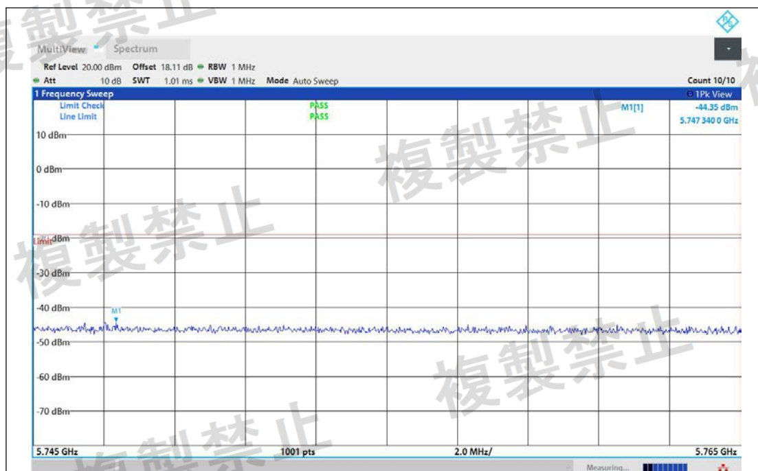
NTNV-11A-Ant1-5700-5745~5765-PASS
