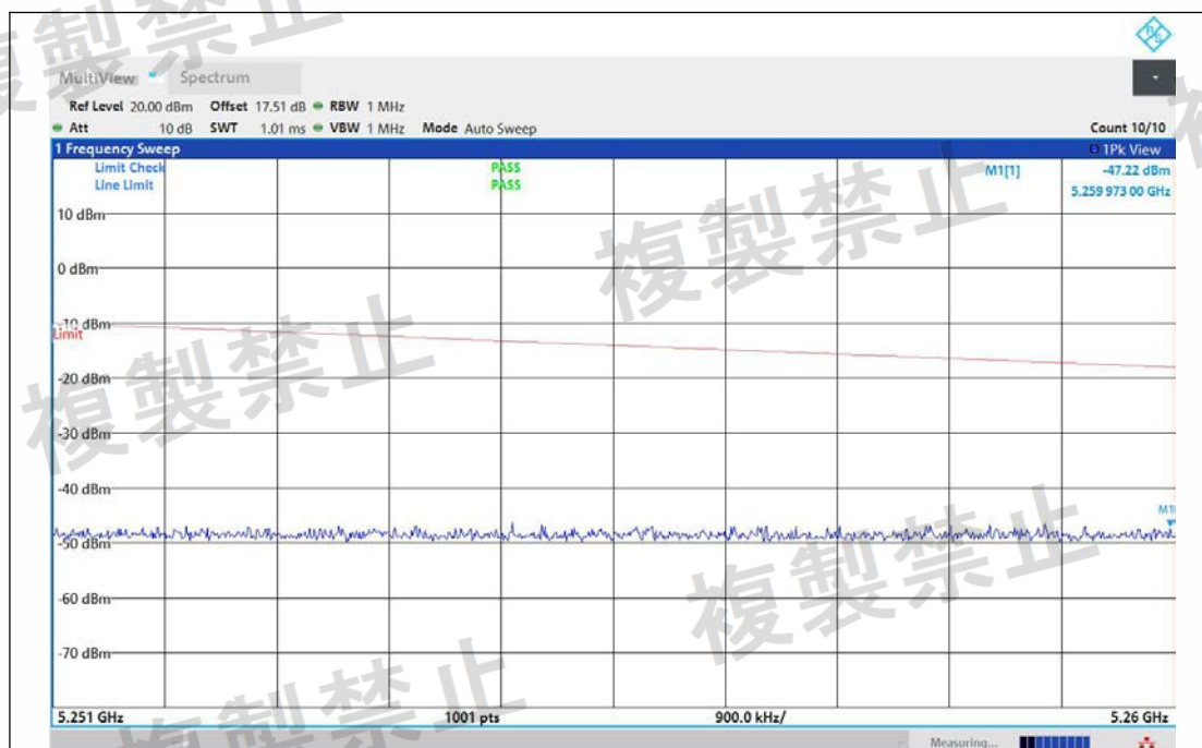
NTNV-11AC20MIMO-Ant1-5180-5251~5260-PASS
