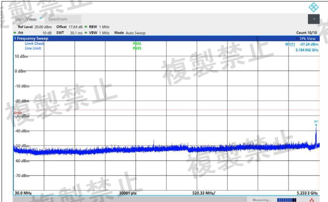
NTNV-11N20MIMO-Ant1-5260-30~5233.3-PASS
