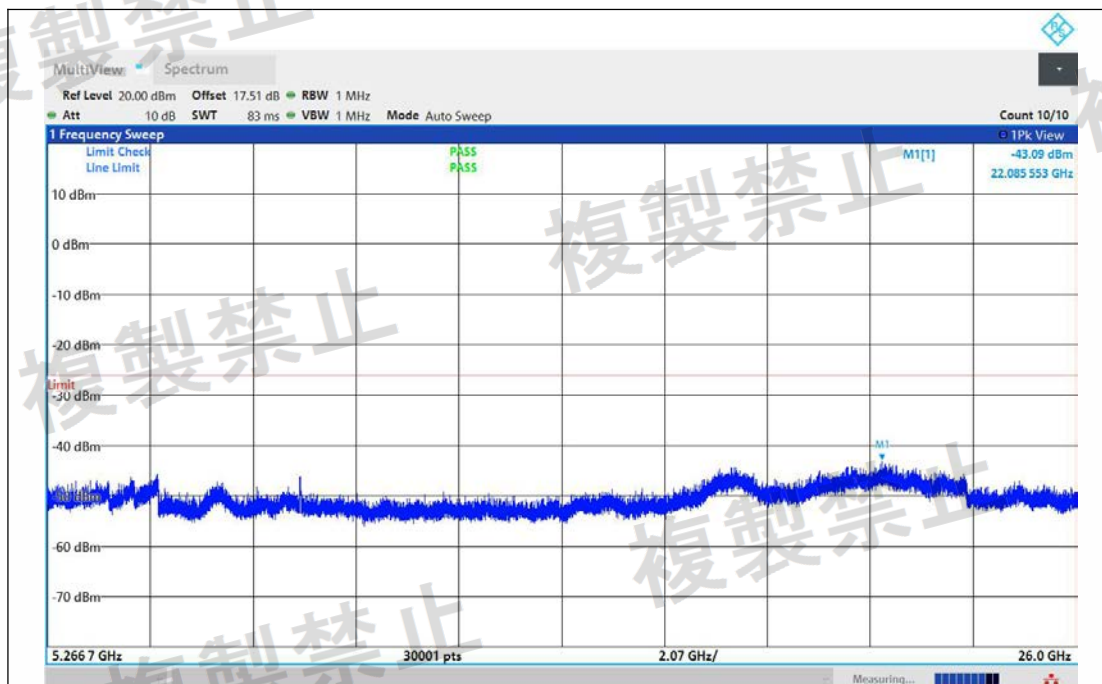
NTNV-11AC20MIMO-Ant1-5180-5266.7~26000-PASS
