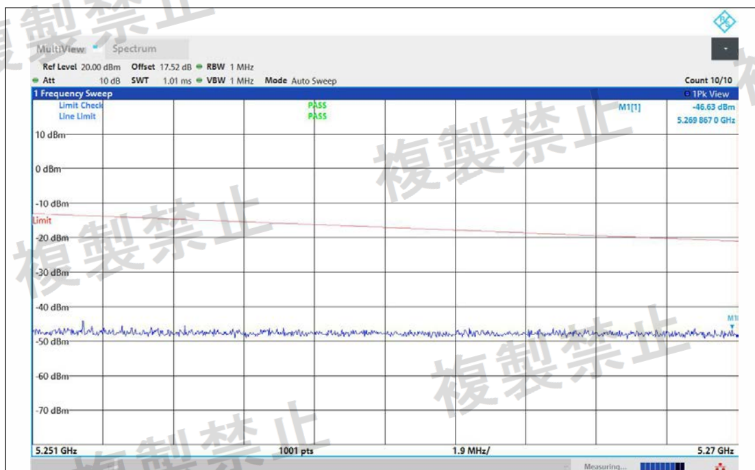
NTNV-11N40MIMO-Ant1-5190-5251~5270-PASS
