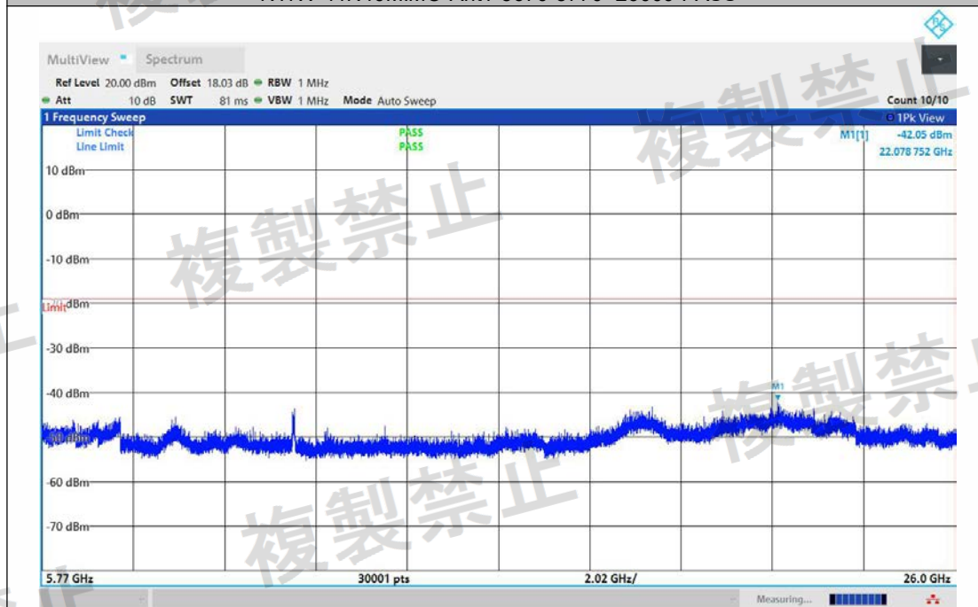
NTNV-11N40MIMO-Ant2-5670-5770~26000-PASS
