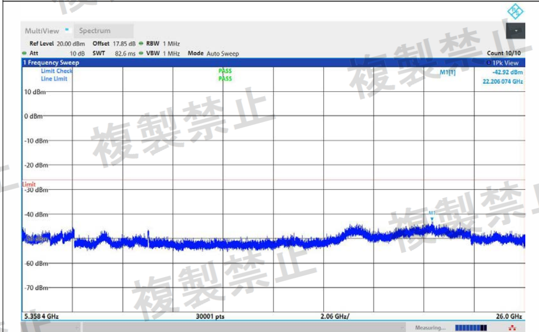
NTNV-11N40MIMO-Ant2-5270-5358.4~26000-PASS
