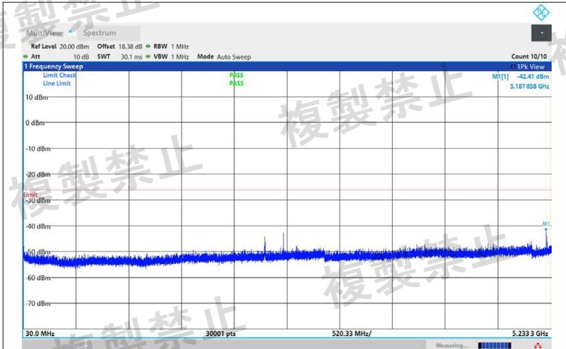
NTNV-11N20MIMO-Ant1-5320-30~5233.3-PASS
