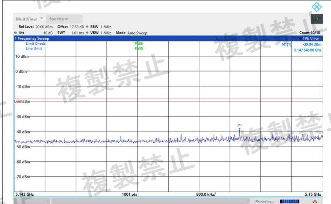
NTNV-11N20MIMO-Ant2-5180-5142~5150-PASS
