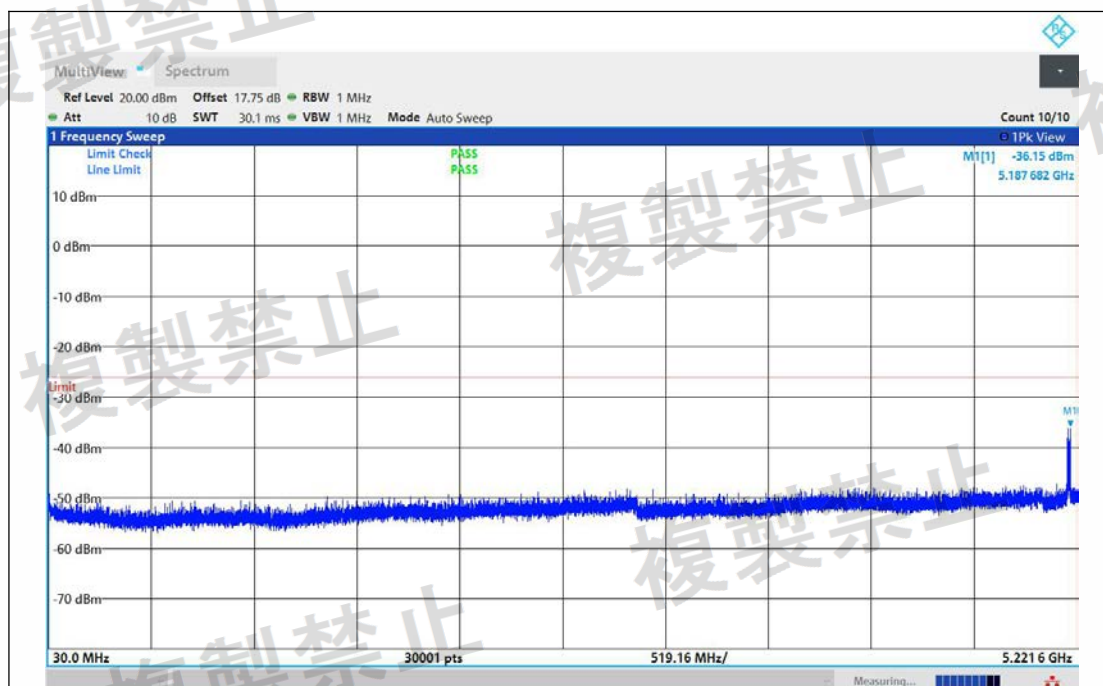
NTNV-11N40MIMO-Ant1-5270-30~5221.6-PASS
