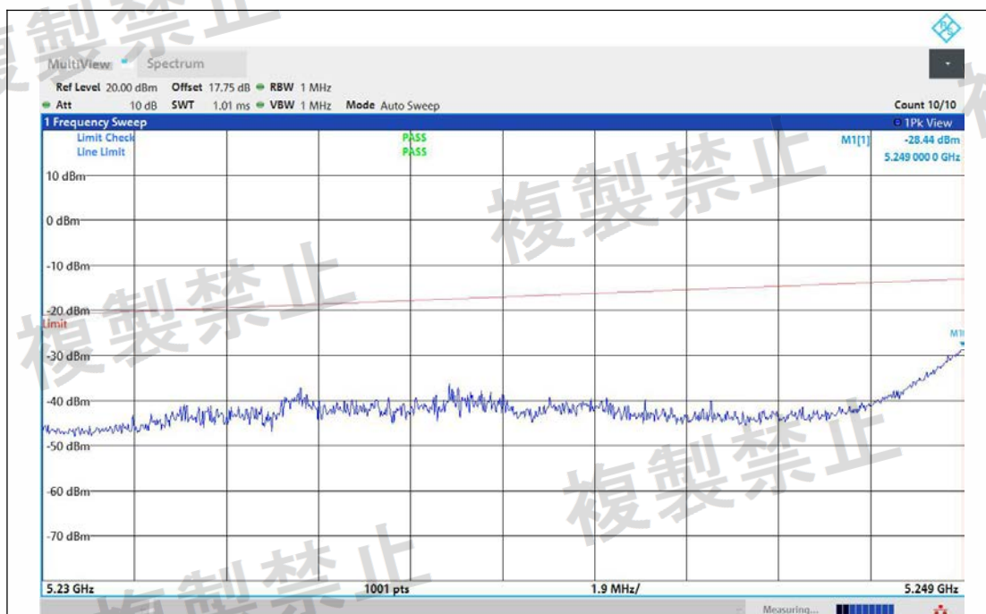
NTNV-11N40MIMO-Ant1-5270-5230~5249-PASS
