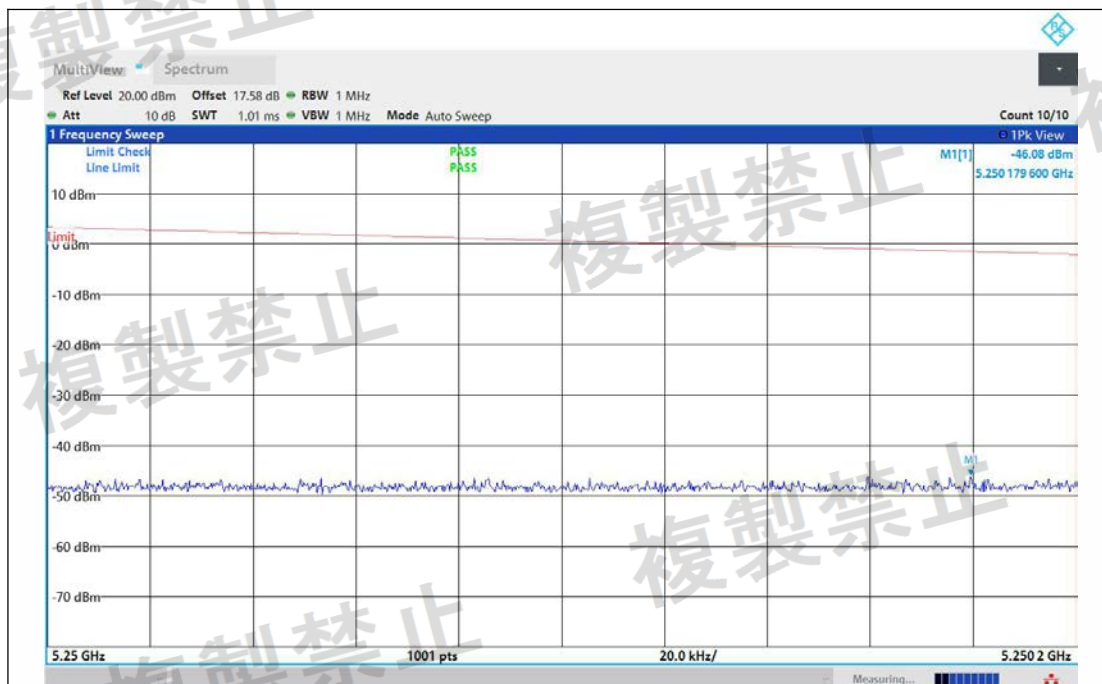
NTNV-11N20MIMO-Ant1-5200-5250~5250.2-PASS
