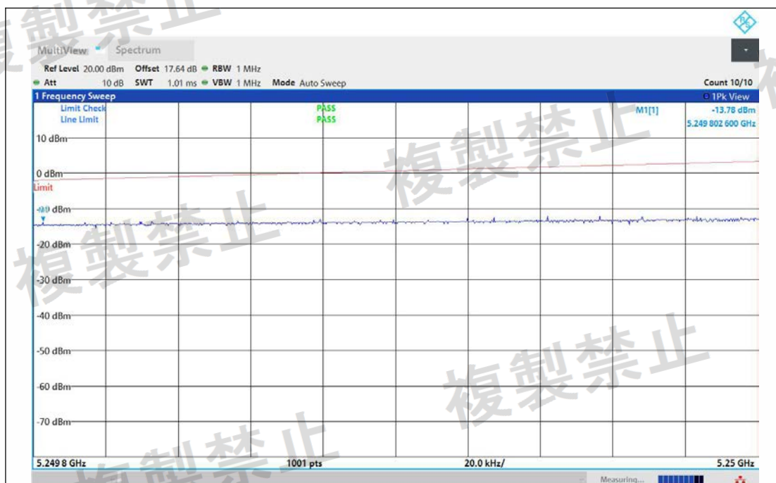
NTNV-11N20MIMO-Ant1-5260-5249.8~5250-PASS
