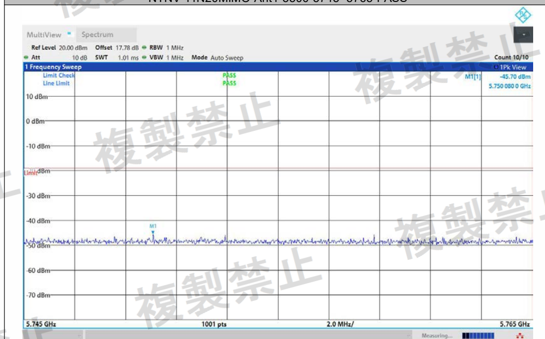
NTNV-11N20MIMO-Ant2-5500-5745~5765-PASS
