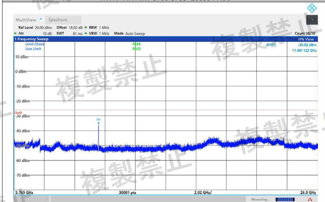
NTNV-11A-Ant2-5700-5765~26000-PASS
