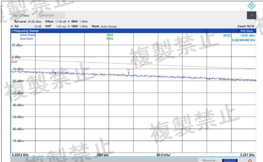
NTVN-11N20MIMO-Ant1-5240-5250.2~5251-PASS
