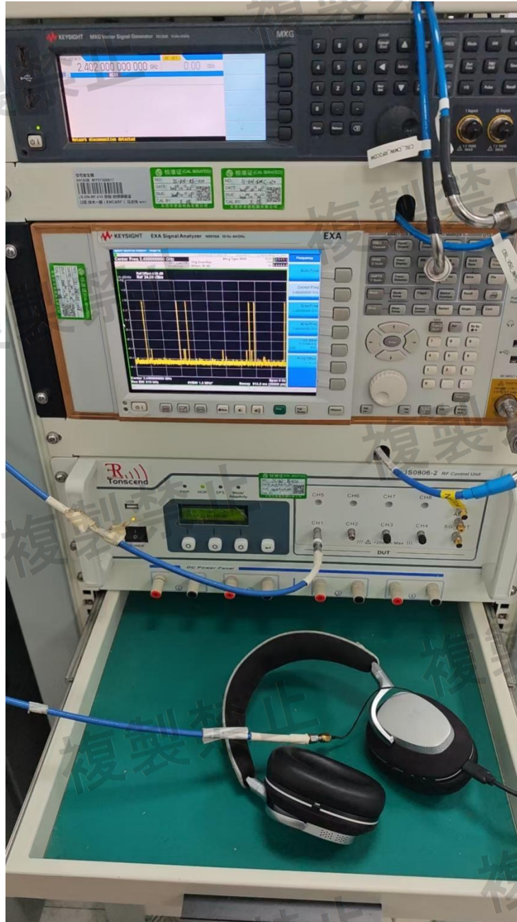
Antenna Terminal Test View
