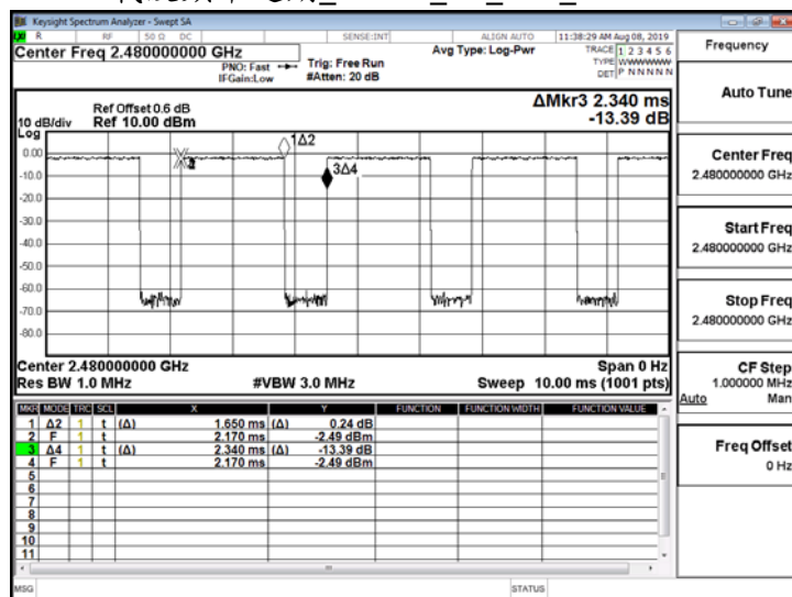
載波頻率週期_8DPSK_3M_DH3_2480MHz
