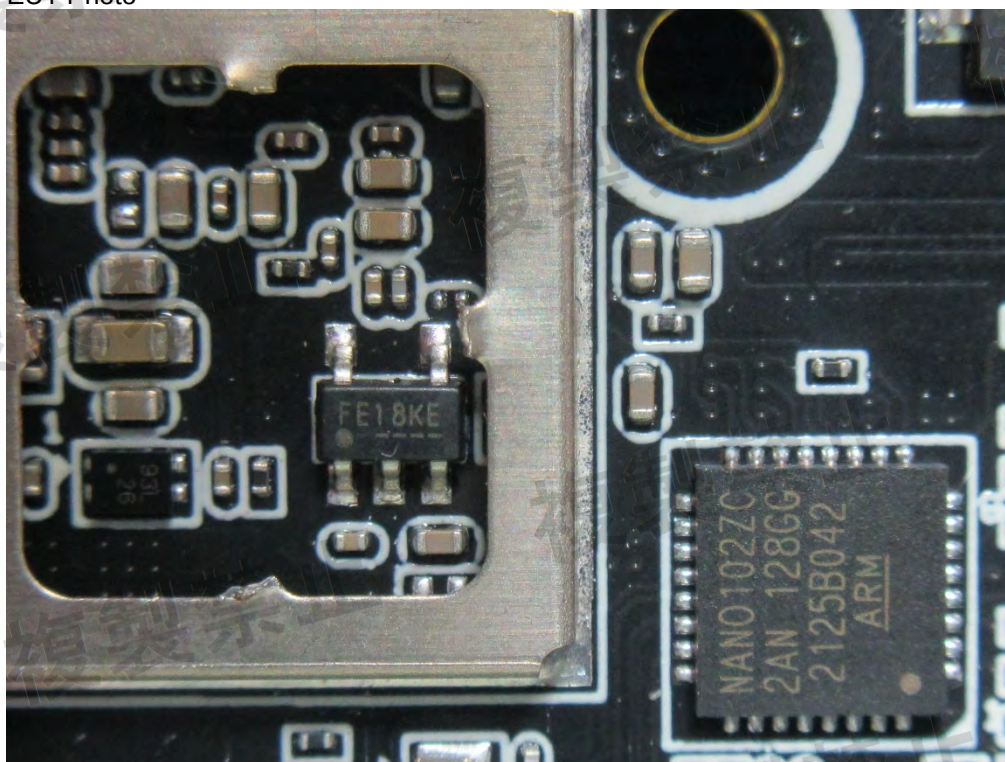
(26) EUT Photo
