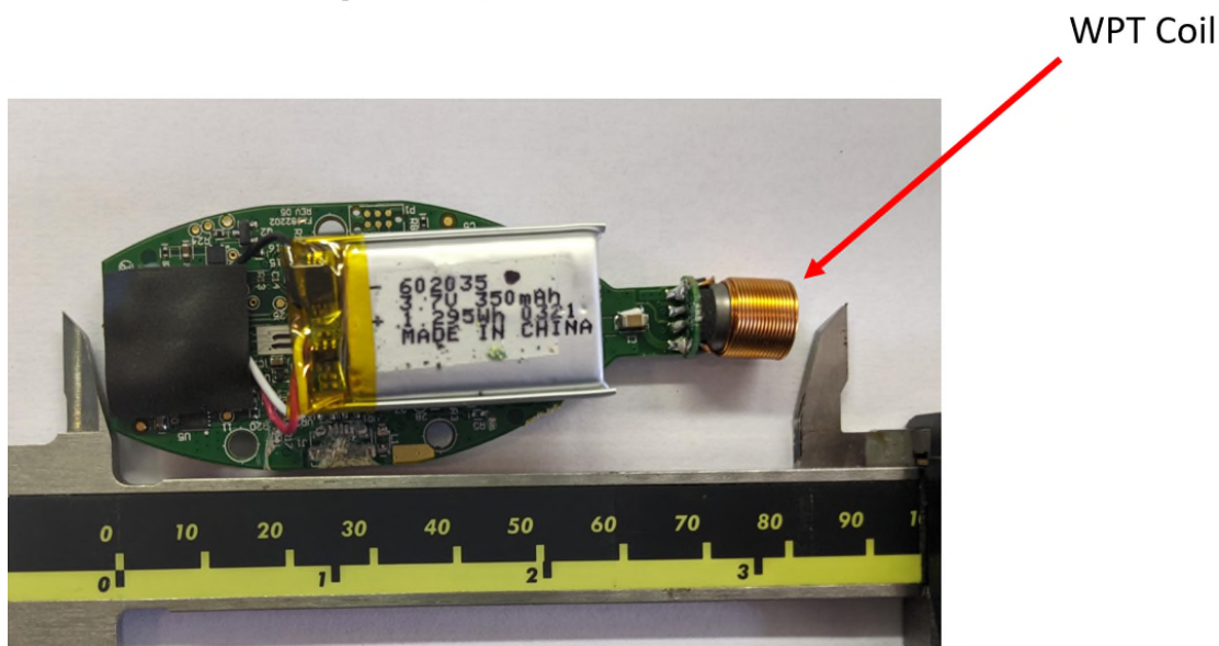
Photo 1.4-1 – Top View of the PCB
