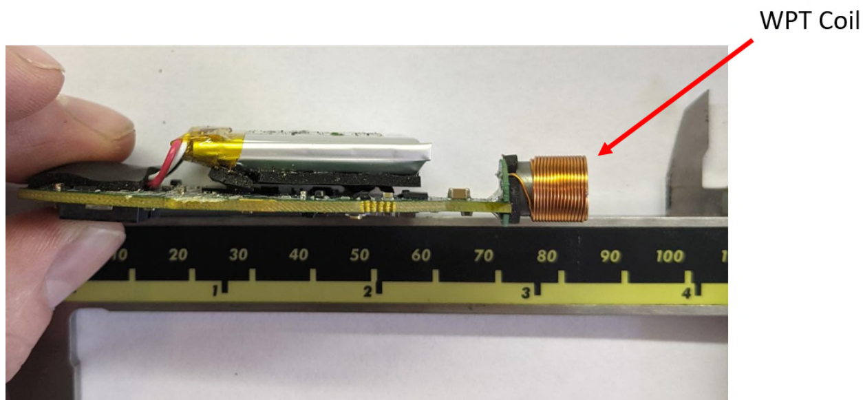
Photo 1.4-3 – Right Side View of the PCB
