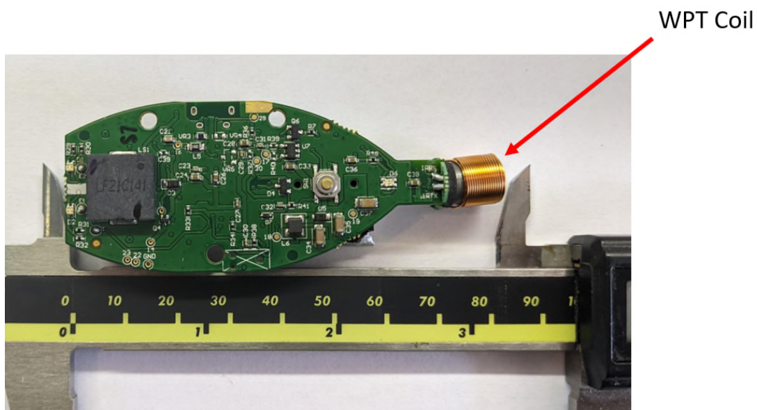
Photo 1.4-2 – Bottom View of the PCB
