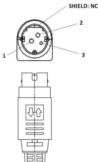
Fig. 3.2: Ion R4301P Plug Cable Connector
