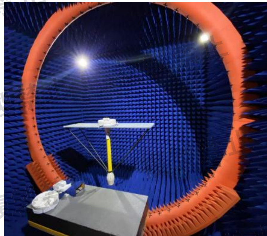
Testing 3D microwave darkroom(6m*6m*6m)
