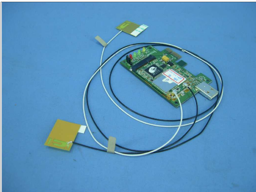
天線 91 (Brand: FOXCONN / Model: WDAN-TQ (Tx1), WDAN-TQ (Tx2))
