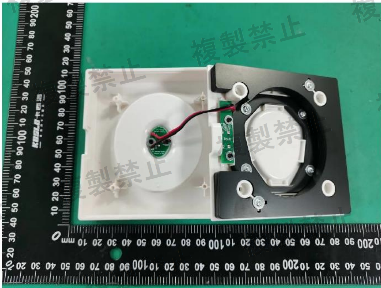
Figure 4: Internal view for charging base
