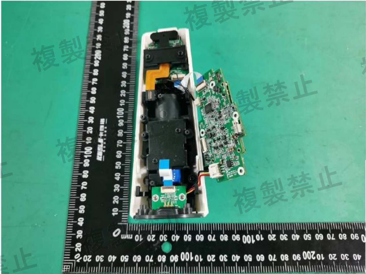
Figure 9: Internal view_2 of product
