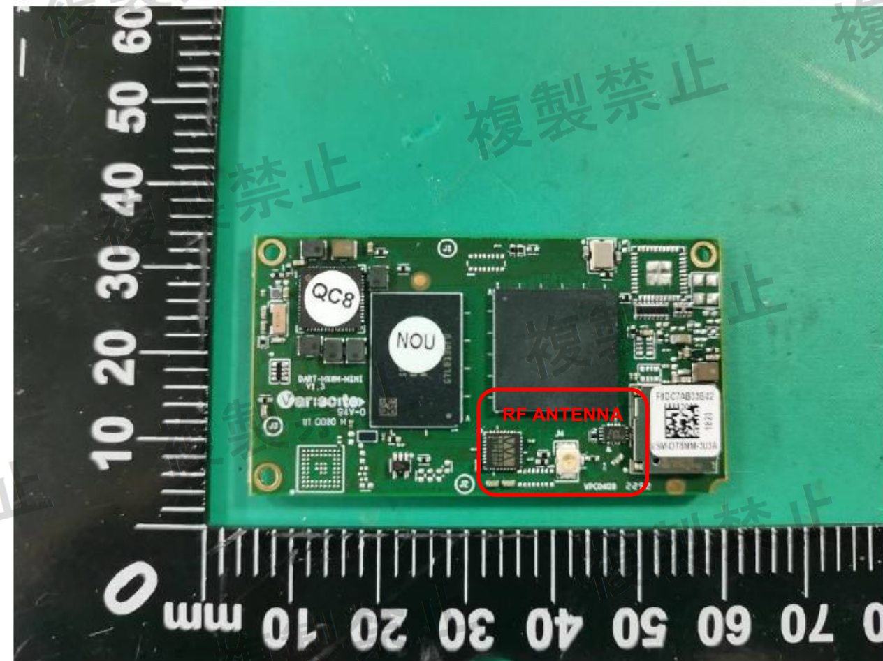
Figure 13: Main board view_4 of product
