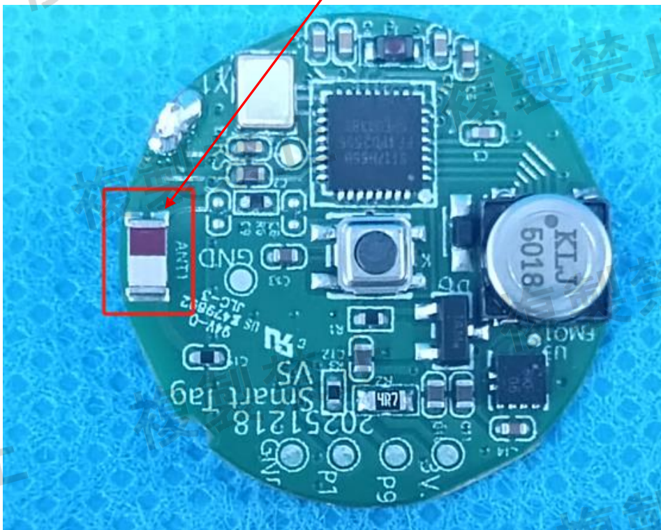
View of RF antenna
