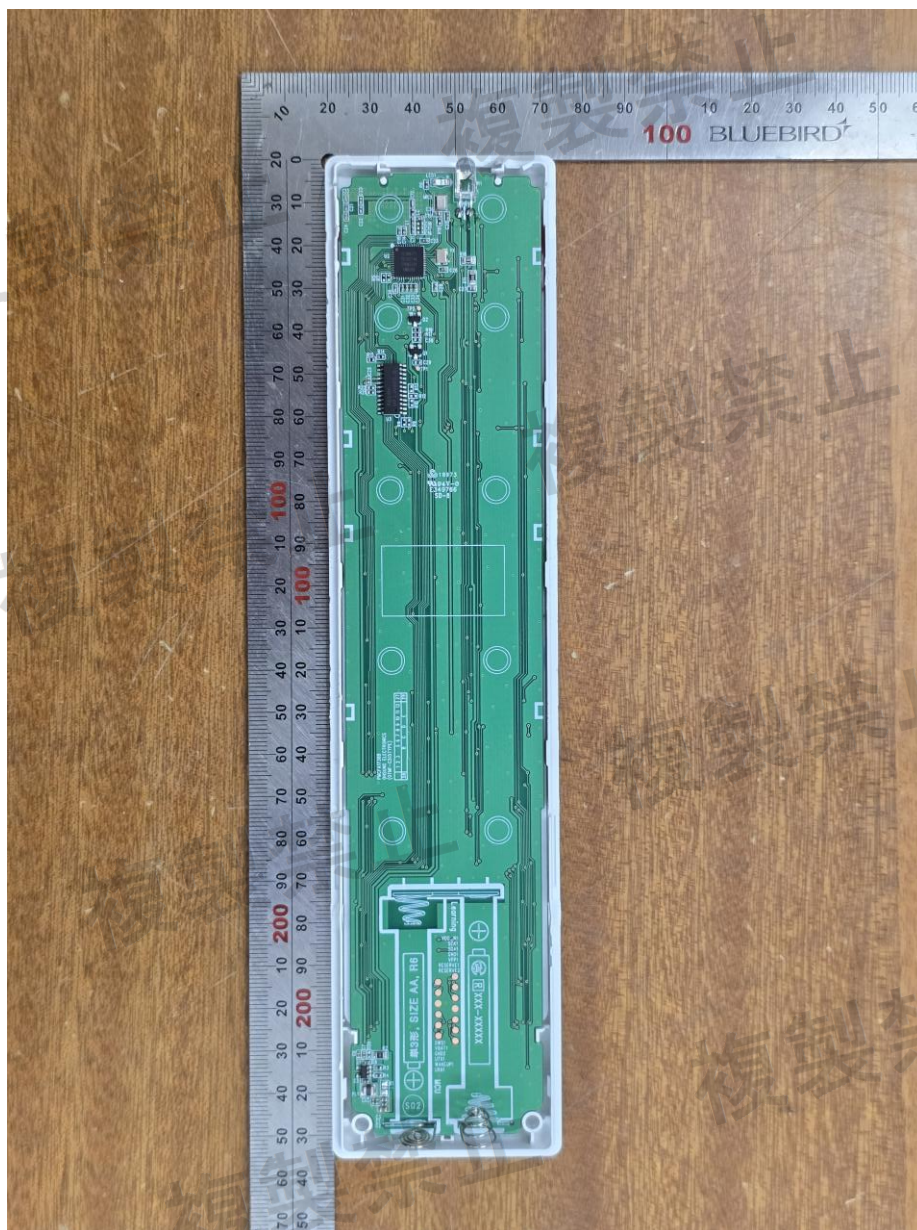
< Inside view >
