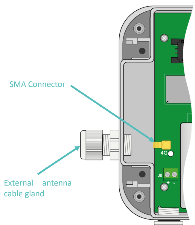
External Antenna
