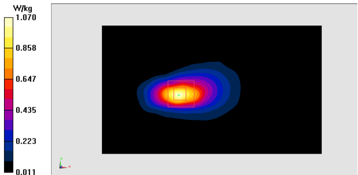
Fig.10 1700 MHz
