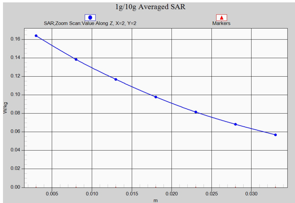
Fig. 22-1 Z-Scan at power reference point (LTE Band12)
