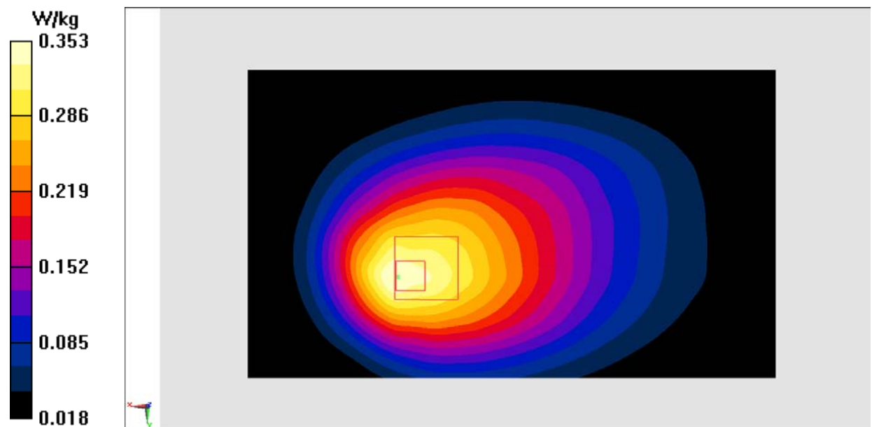
Fig.23 LTE Band12
