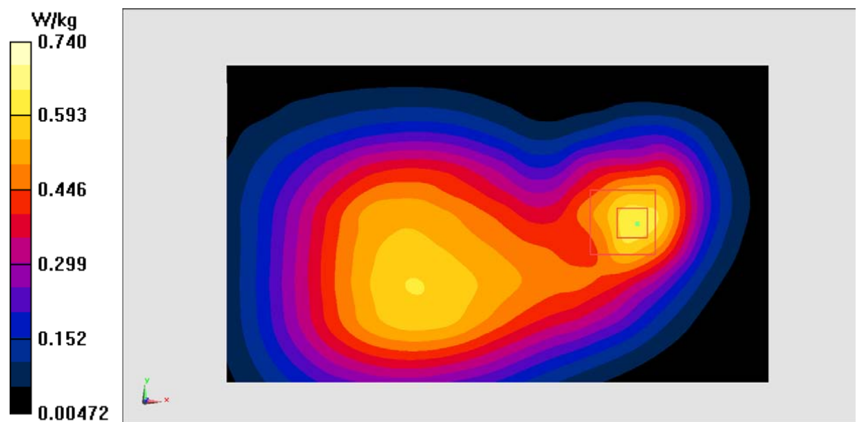
Fig.2 850 MHz
