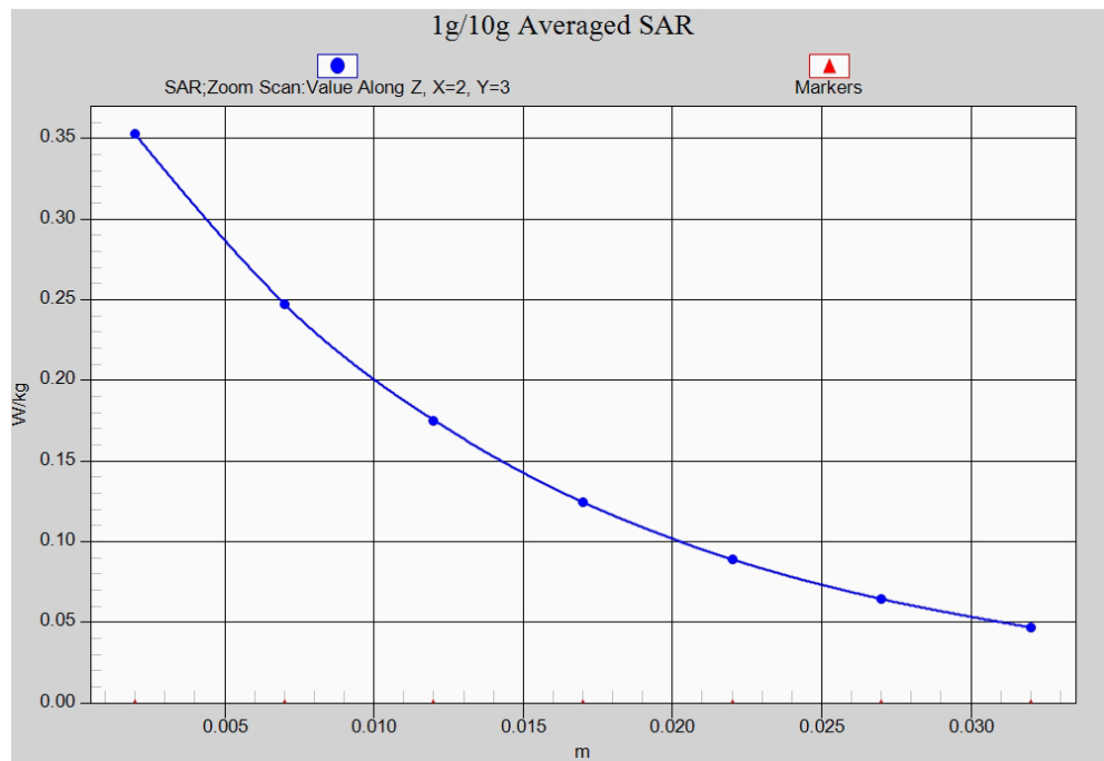
Fig. 23-1 Z-Scan at power reference point (LTE Band12)
