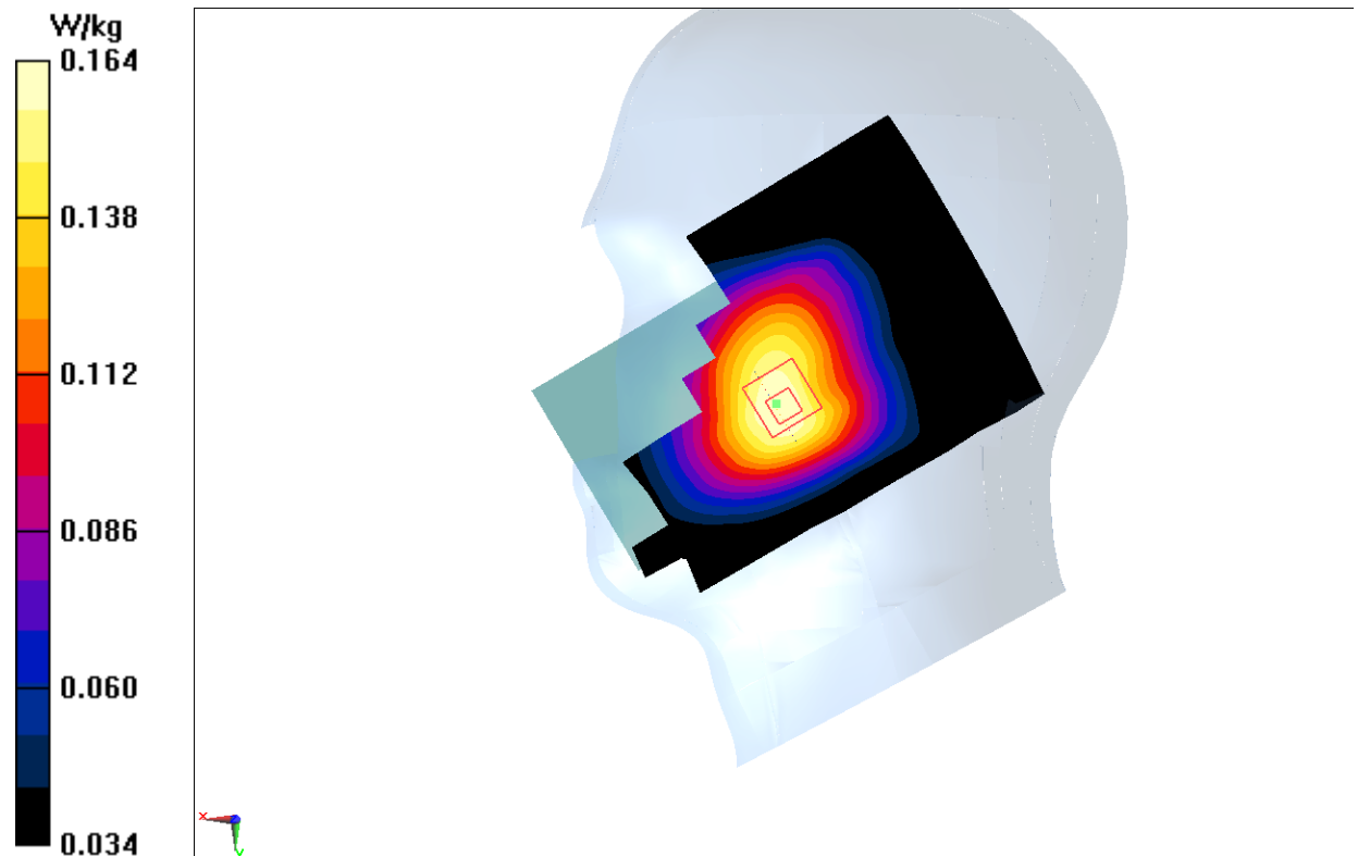
Fig.22 LTE Band12
