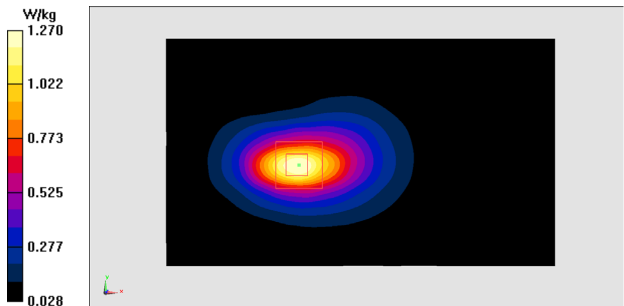
Fig.9 1700 MHz
