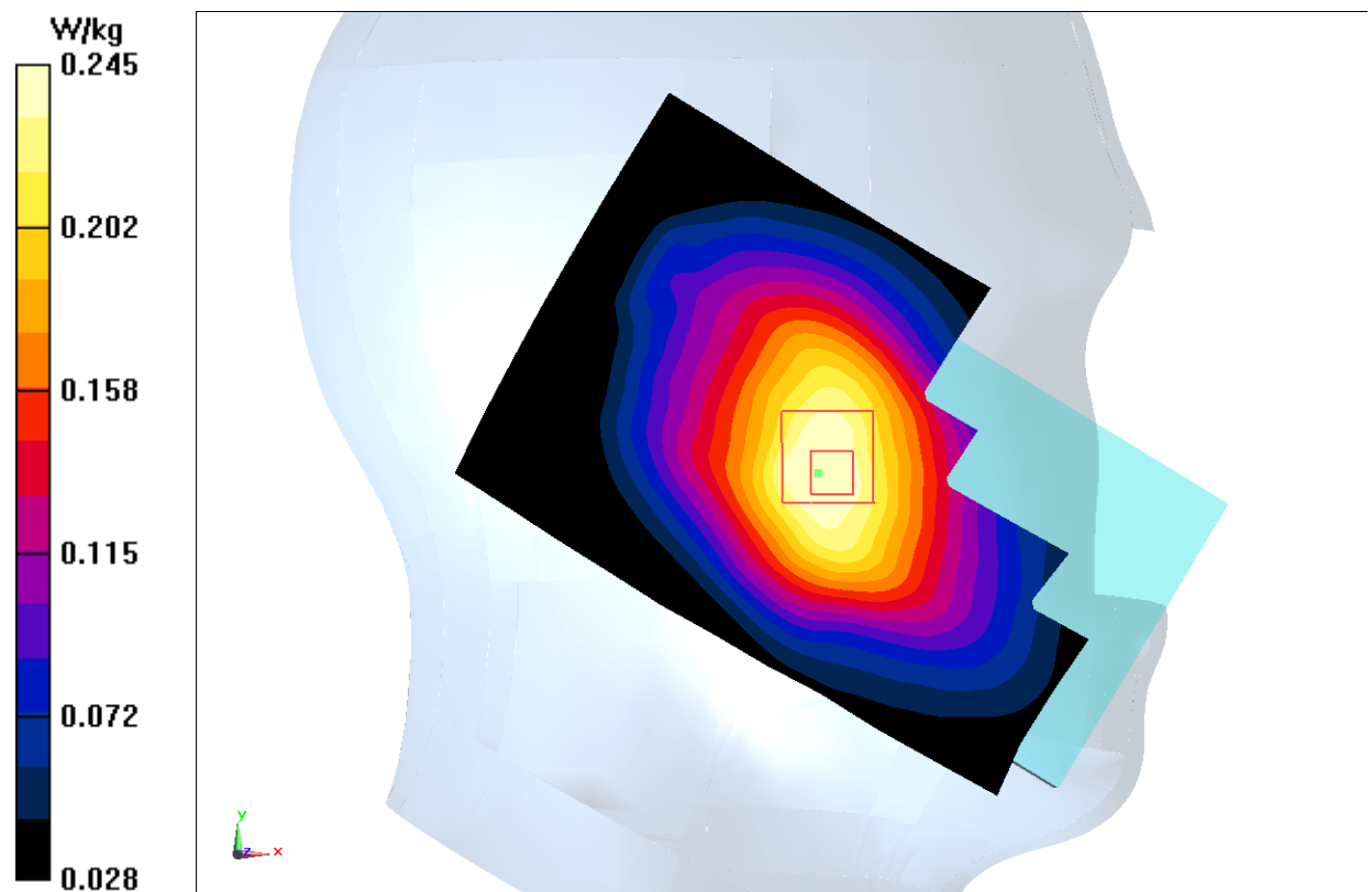
Fig.20 LTE Band5
