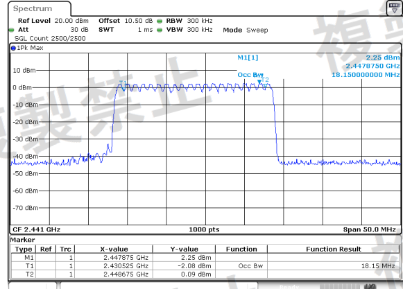
Spreading Bandwidth
