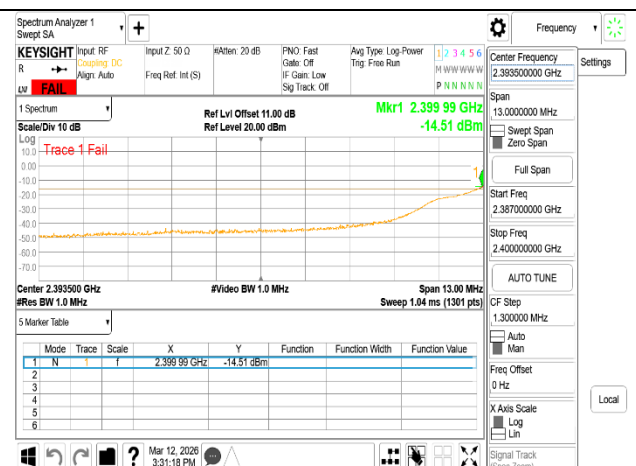
TX 2387MHz~2400MHz Proprietary mode 2403MHz
