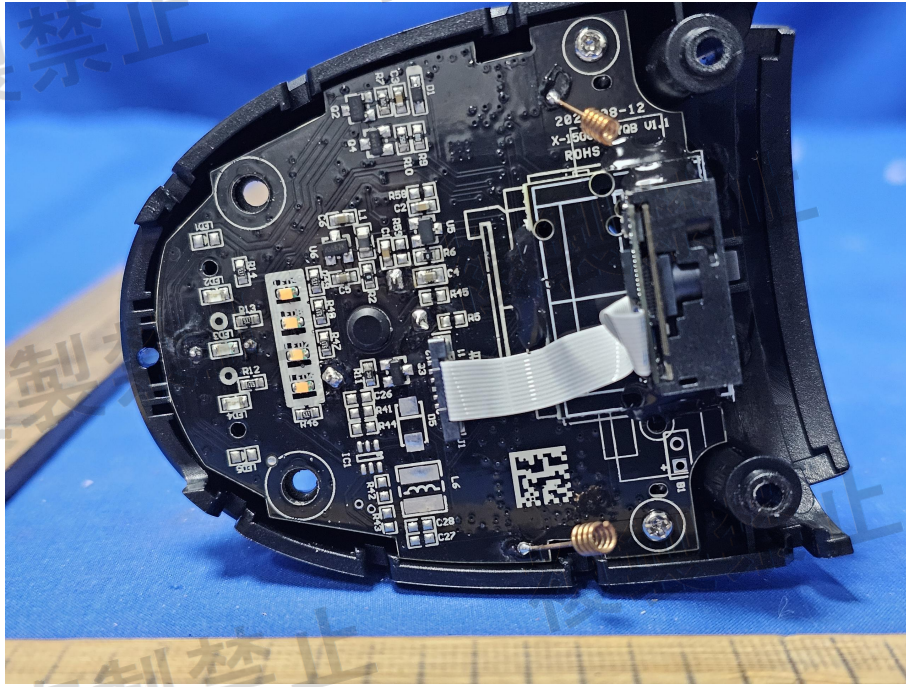
Antenna 1
