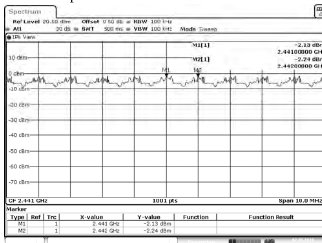
Channel Separation
