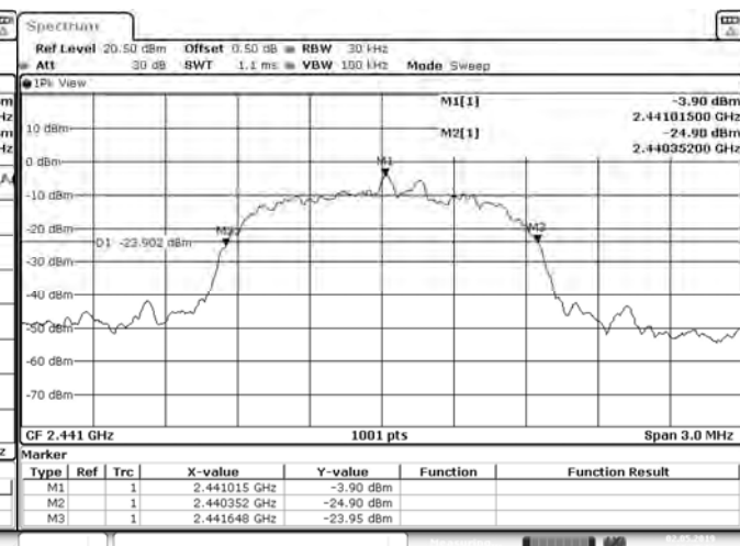
20dB Bandwidth
