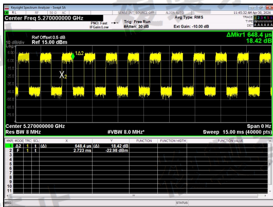
NT/NV_Antenna 0_IEEE 802.11n_40_Channel 54
