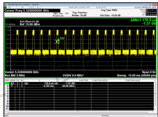
NT/NV_Antenna 1_IIEEE 802.11a_Channel 64
