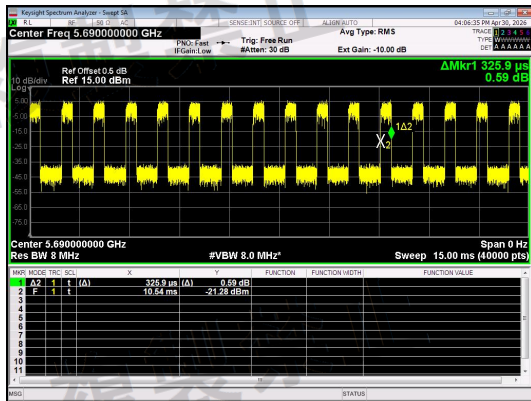
NT/NV_Antenna 0_IIEEE 802.11ac_80_Channel 138
