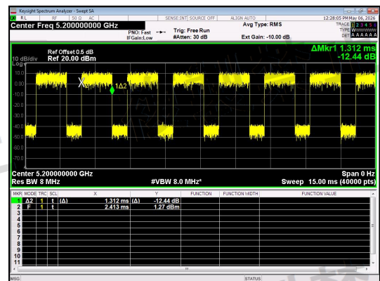
NT/NV_Antenna 1_IIEEE 802.11ac_20_Channel 40
