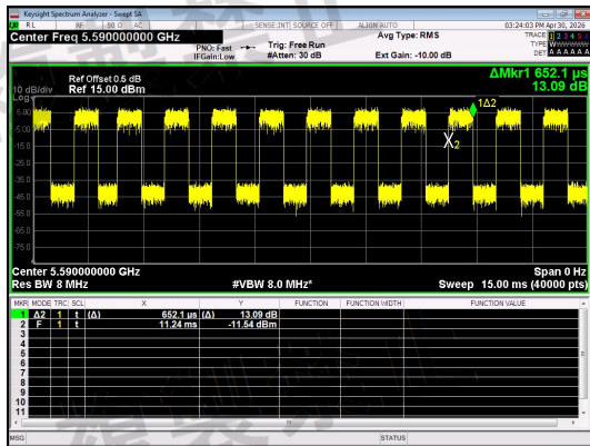
NT/NV_Antenna 0_IIEEE 802.11ac_40_Channel 118
