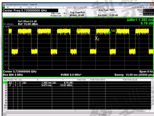
NT/NV_Antenna 0_IIEEE 802.11n_20_Channel 144
