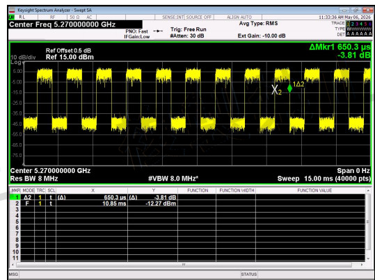
NT/NV_Antenna 1_IEEE 802.11n_40_Channel 54
