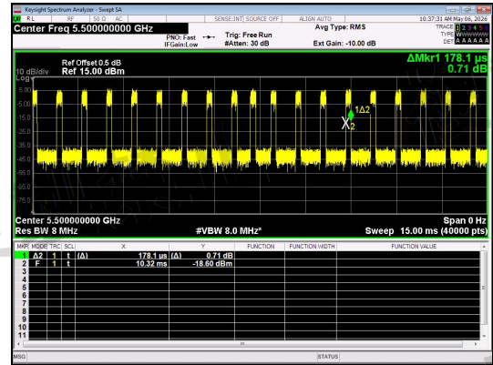
NT/NV_Antenna 1_IIEEE 802.11a_Channel 100
