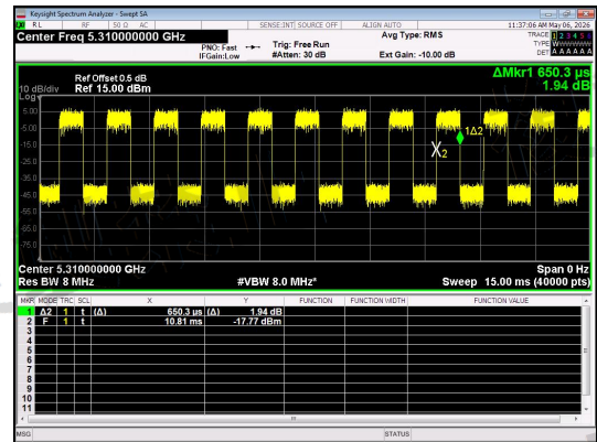
NT/NV_Antenna 1_IIEEE 802.11n_40_Channel 62
