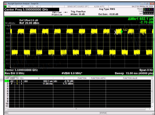
NT/NV_Antenna 1_IIEEE 802.11ac_40_Channel 118
