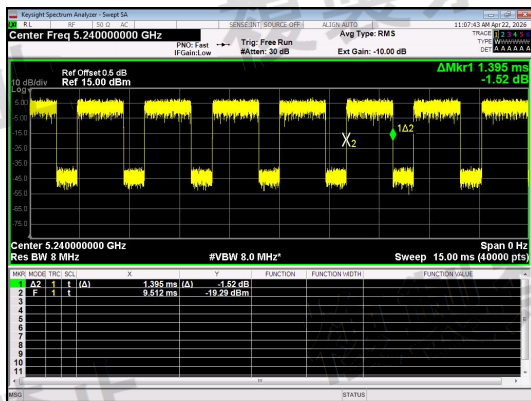
NT/NV_Antenna 0_IEEE 802.11n_20_Channel 48
