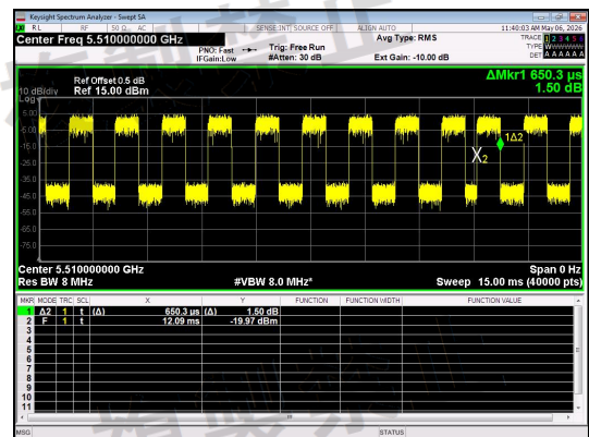
NT/NV_Antenna 1_IIEEE 802.11n_40_Channel 102
