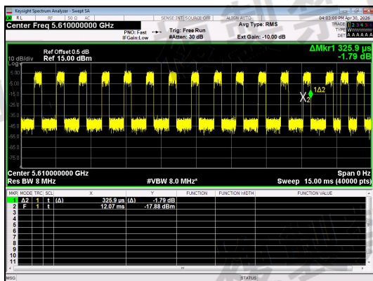
NT/NV_Antenna 0_IIEEE 802.11ac_80_Channel 122
