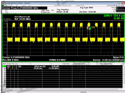
NT/NV_Antenna 0_IIEEE 802.11ac_80_Channel 42
