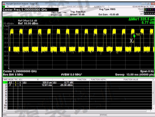
NT/NV_Antenna 0_IIEEE 802.11ac_80_Channel 58
