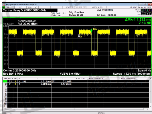
NT/NV_Antenna 0_IIEEE 802.11ac_20_Channel 40
