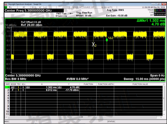
NT/NV_Antenna 1_ IEEE 802.11n_20_Channel 60
