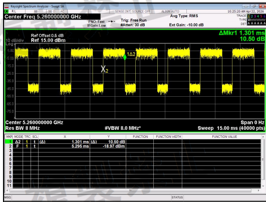
NT/NV_Antenna 0_IIEEE 802.11a_Channel 52
