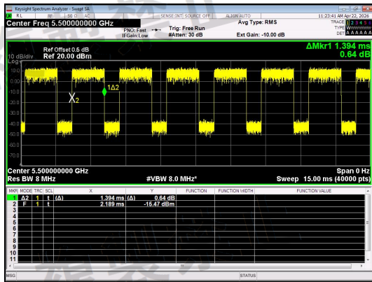
NT/NV_Antenna 0_IIEEE 802.11n_20_Channel 100
