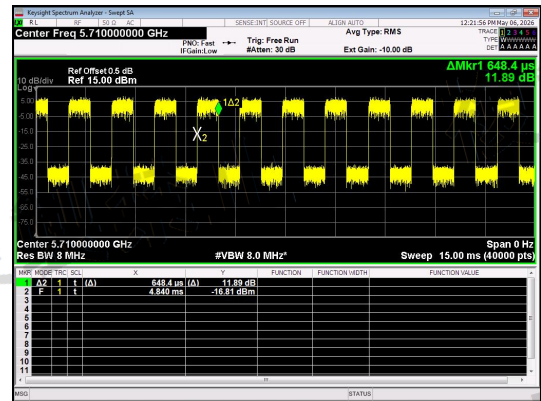
NT/NV_Antenna 1_IIEEE 802.11n_40_Channel 142
