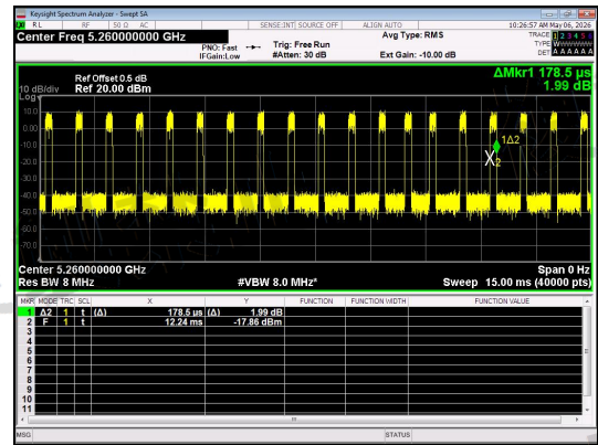
NT/NV_Antenna 1_IIEEE 802.11a_Channel 52
