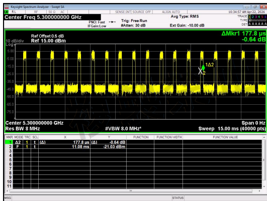
NT/NV_Antenna 0_IIEEE 802.11a_Channel 60
