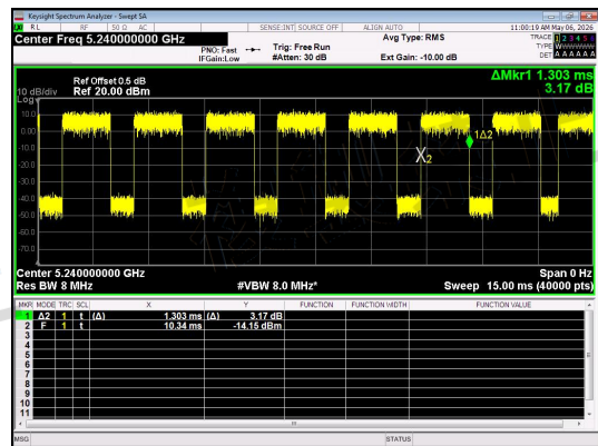
NT/NV_Antenna 1_IEEE 802.11n_20_Channel 48
