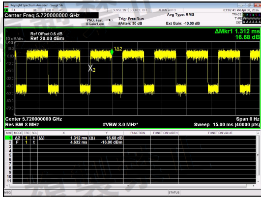
NT/NV_Antenna 0_IIEEE 802.11ac_20_Channel 144
