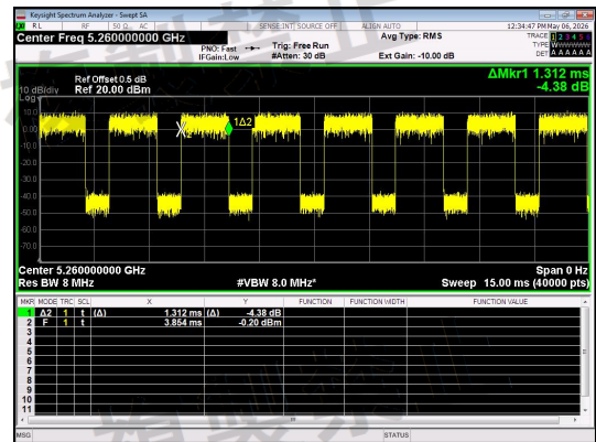
NT/NV_Antenna 1_IIEEE 802.11ac_20_Channel 52
