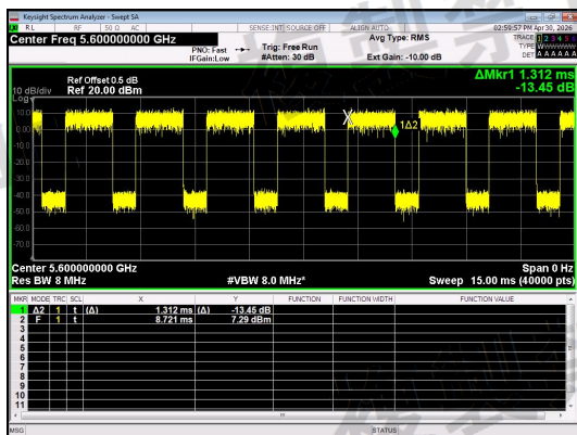
NT/NV_Antenna 0_IIEEE 802.11ac_20_Channel 120
