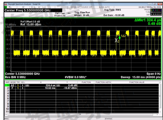
NT/NV_Antenna 1_IIEEE 802.11ac_80_Channel 106
