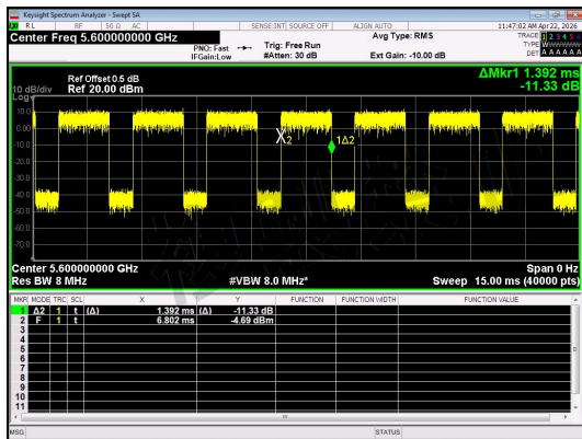
NT/NV_Antenna 0_IIEEE 802.11n_20_Channel 120
