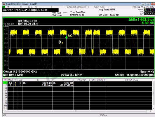
NT/NV_Antenna 0_IIEEE 802.11ac_40_Channel 62
