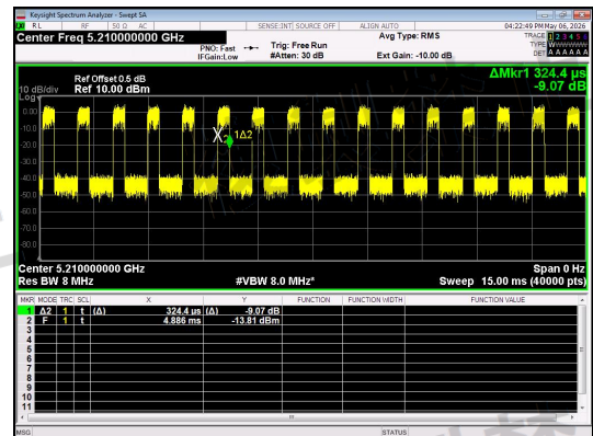
NT/NV_Antenna 1_IIEEE 802.11ac_80_Channel 42
