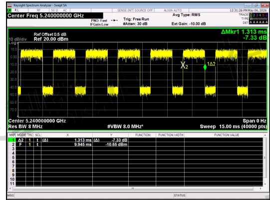
NT/NV_Antenna 1_IIEEE 802.11ac_20_Channel 48
