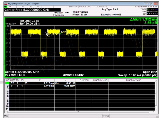
NT/NV_Antenna 1_IIEEE 802.11ac_20_Channel 64
