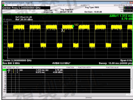
NT/NV_Antenna 0_IIEEE 802.11ac_20_Channel 48
