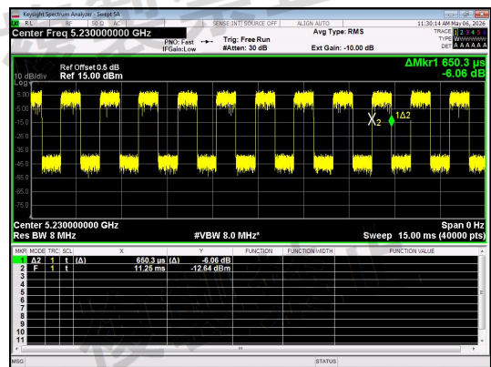
NT/NV_Antenna 1_IEEE 802.11n_40_Channel 46
