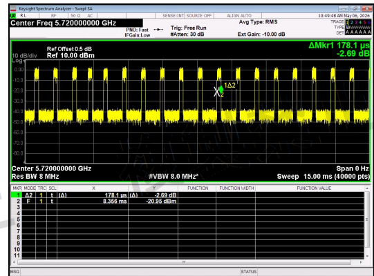
NT/NV_Antenna 1_IIEEE 802.11a_Channel 144
