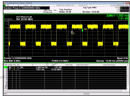
NT/NV_Antenna 1_ IEEE 802.11n_20_Channel 64
