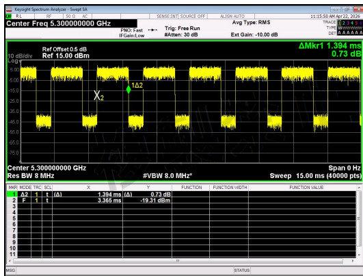
NT/NV_Antenna 0_ IEEE 802.11n_20_Channel 60
