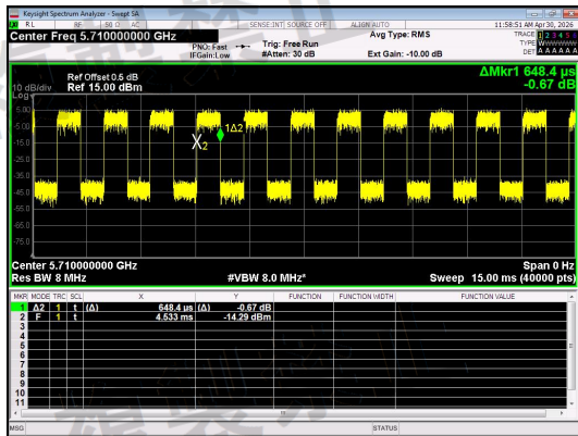
NT/NV_Antenna 0_IIEEE 802.11n_40_Channel 142
