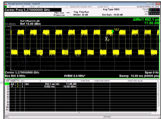
NT/NV_Antenna 1_IIEEE 802.11ac_40_Channel 54
