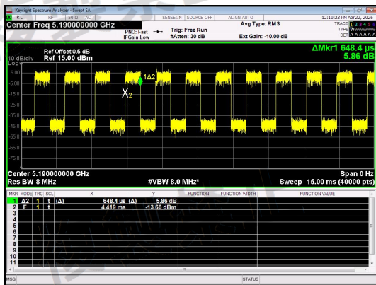
NT/NV_Antenna 0_IEEE 802.11n_40_Channel 38
