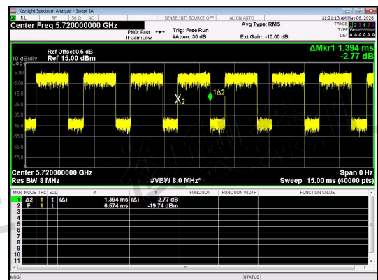
NT/NV_Antenna 1_IIEEE 802.11n_20_Channel 144
