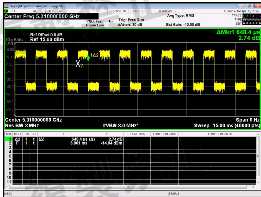
NT/NV_Antenna 0_IIEEE 802.11n_40_Channel 62
