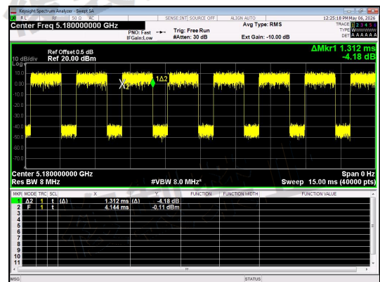
NT/NV_Antenna 1_IIEEE 802.11ac_20_Channel 36
