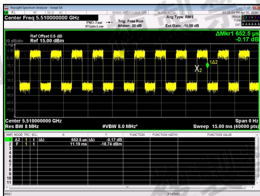
NT/NV_Antenna 0_IIEEE 802.11ac_40_Channel 102
