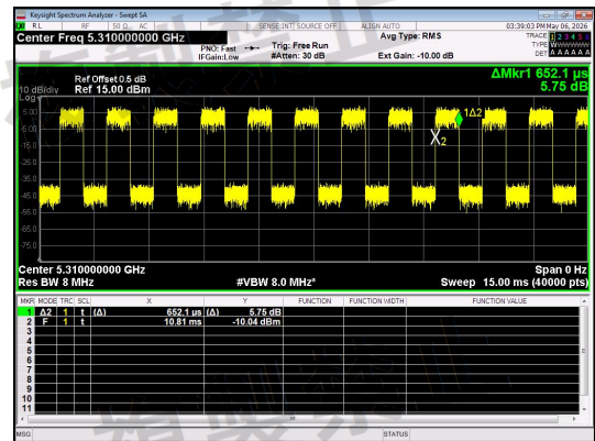
NT/NV_Antenna 0_IIEEE 802.11ac_40_Channel 62
