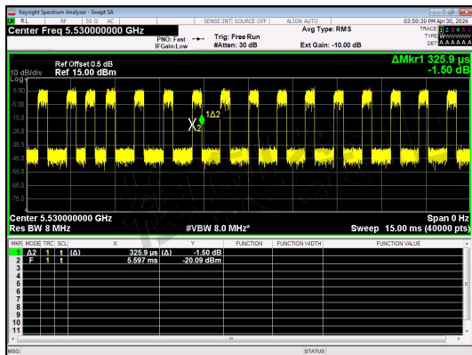
NT/NV_Antenna 0_IIEEE 802.11ac_80_Channel 106
