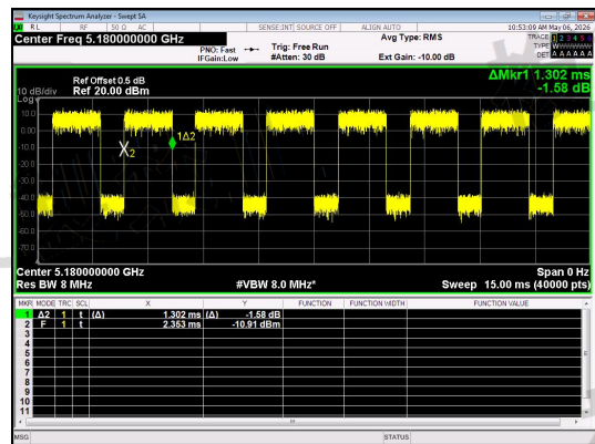
NT/NV_Antenna 1_IEEE 802.11n_20_Channel 36
