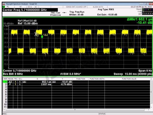
NT/NV_Antenna 0_IIEEE 802.11ac_40_Channel 142
