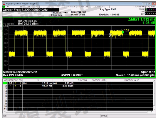
NT/NV_Antenna 0_IIEEE 802.11ac_20_Channel 64
