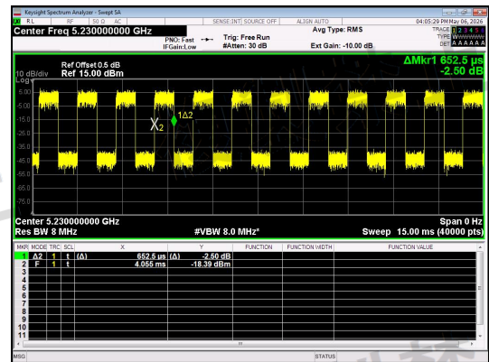
NT/NV_Antenna 1_IIEEE 802.11ac_40_Channel 46
