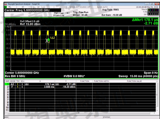
NT/NV_Antenna 1_IIEEE 802.11a_Channel 120
