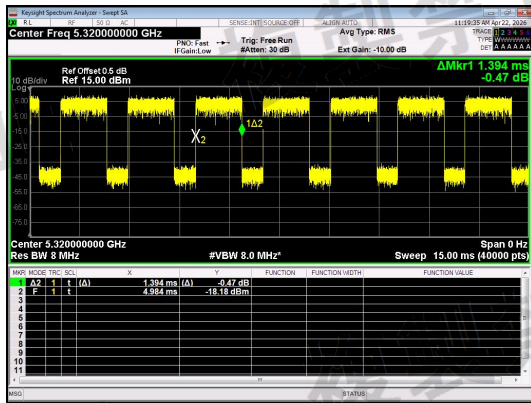
NT/NV_Antenna 0_ IEEE 802.11n_20_Channel 64
