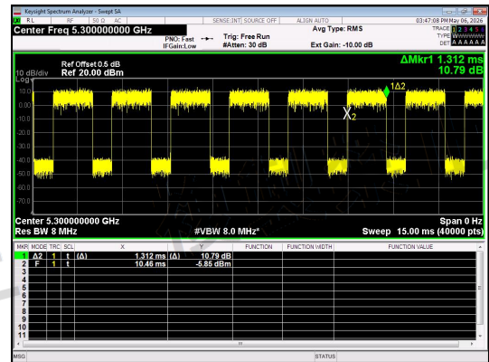
NT/NV_Antenna 1_IIEEE 802.11ac_20_Channel 60
