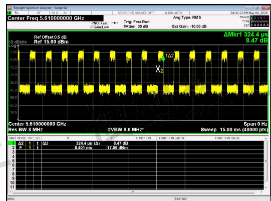
NT/NV_Antenna 1_IIEEE 802.11ac_80_Channel 122
