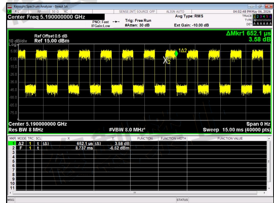
NT/NV_Antenna 1_IIEEE 802.11ac_40_Channel 38
