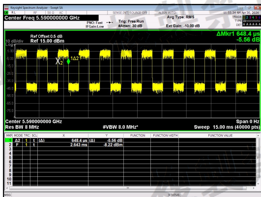
NT/NV_Antenna 0_IIEEE 802.11n_40_Channel 118
