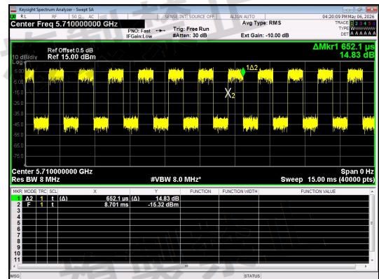
NT/NV_Antenna 1_IIEEE 802.11ac_40_Channel 142
