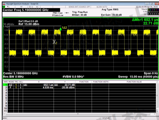
NT/NV_Antenna 0_IIEEE 802.11ac_40_Channel 38
