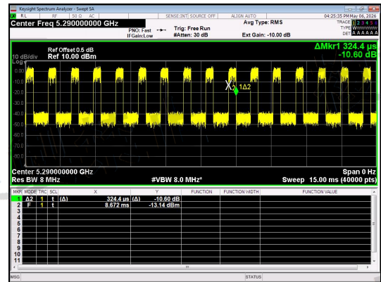
NT/NV_Antenna 1_IIEEE 802.11ac_80_Channel 58
