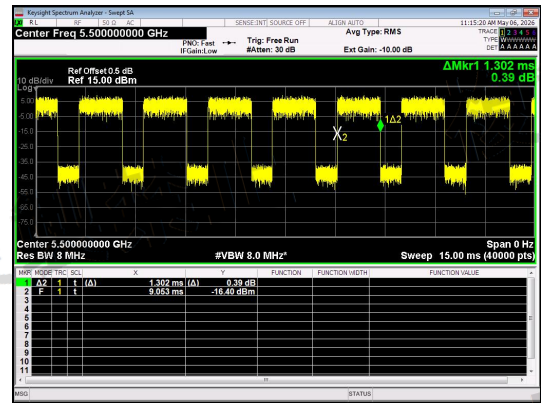
NT/NV_Antenna 1_IIEEE 802.11n_20_Channel 100
