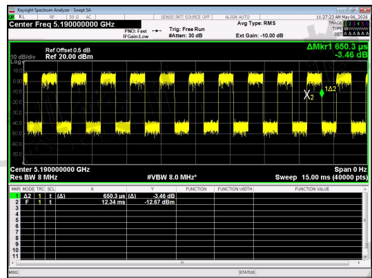
NT/NV_Antenna 1_IEEE 802.11n_40_Channel 38
