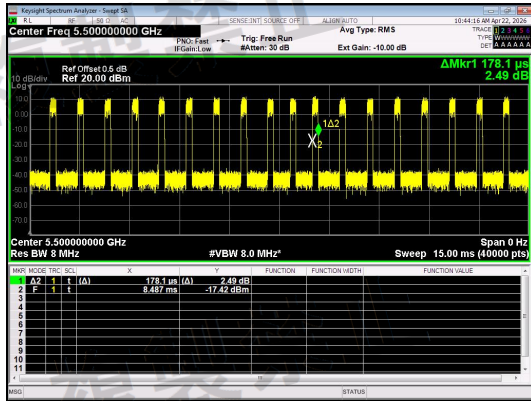
NT/NV_Antenna 0_IIEEE 802.11a_Channel 100
