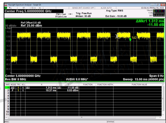
NT/NV_Antenna 1_IIEEE 802.11ac_20_Channel 120
