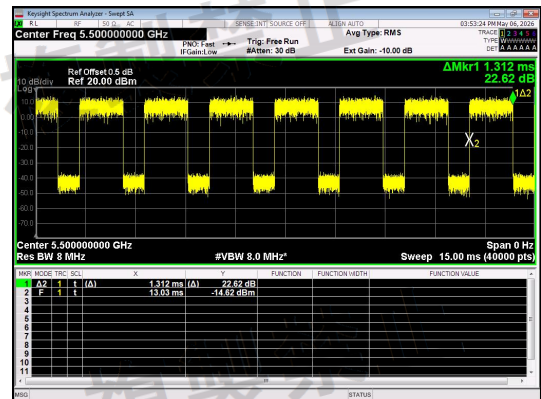
NT/NV_Antenna 1_IIEEE 802.11ac_20_Channel 100
