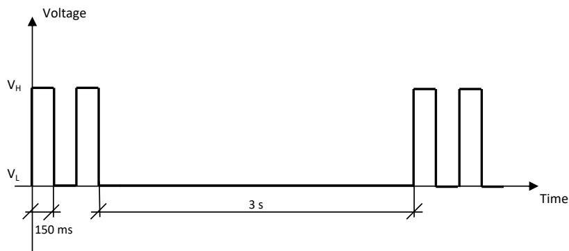
Figure 8: GPIO pin progress for registered roaming 4G
