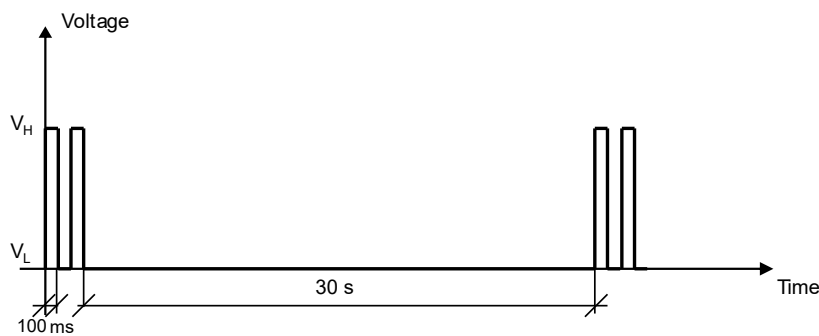
Figure 9: GPIO pin progress for registered roaming NB-IoT
