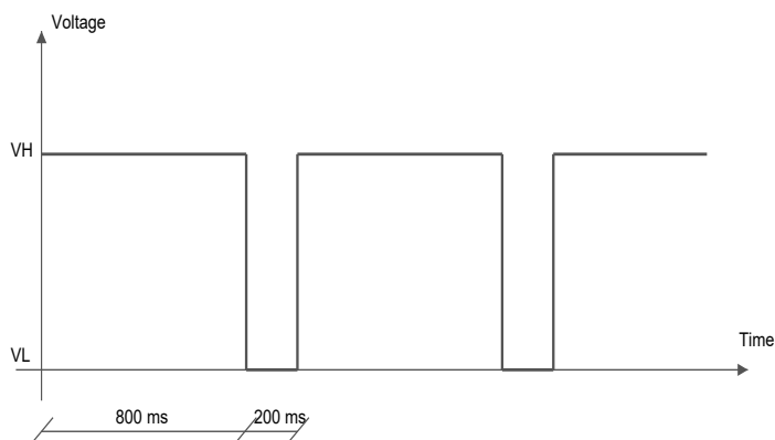
Figure 11: GPIO pin progress for data transmission roaming
