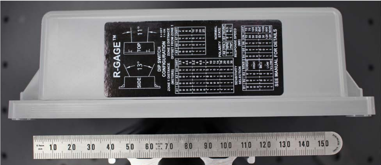
Figure 3, Switch Settings
