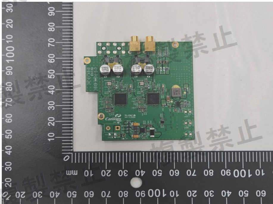
Sub Board #1 Front Side (CTS-CISW-PNA2, CTS-CISW-PNX2 are the same.)
