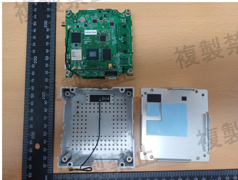
Cover opened #2 (CTS-CISW-PNA4, CTS-CISW-PNA3, CTS-CISW-PNA2, CTS-CISW-PNX4, CTS-CISW-PNX2 are the same.)
