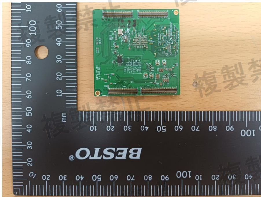
RF Board Rear Side (CTS-CISW-PNA4, CTS-CISW-PNA3, CTS-CISW-PNA2, CTS-CISW-PNX4, CTS-CISW-PNX2 are the same.)
