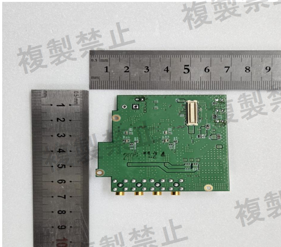
Sub Board #1 Rear Side (CTS-CISW-PNA4, CTS-CISW-PNX4 are the same.)
