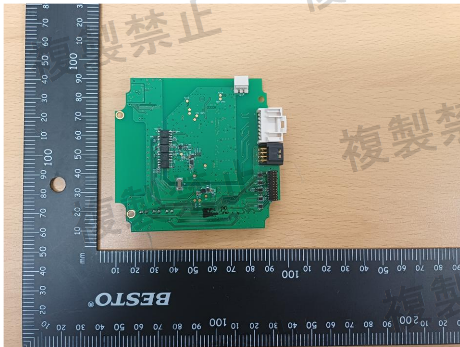
Sub Board #2 Rear Side (This board is used only in the models CTS-CISW-PNA4, CTS-CISW-PNA3, and CTS-CISW-PNA2. It is removed in the models CTS-CISW-PNX4 and CTS-CISW-PNX2.)
