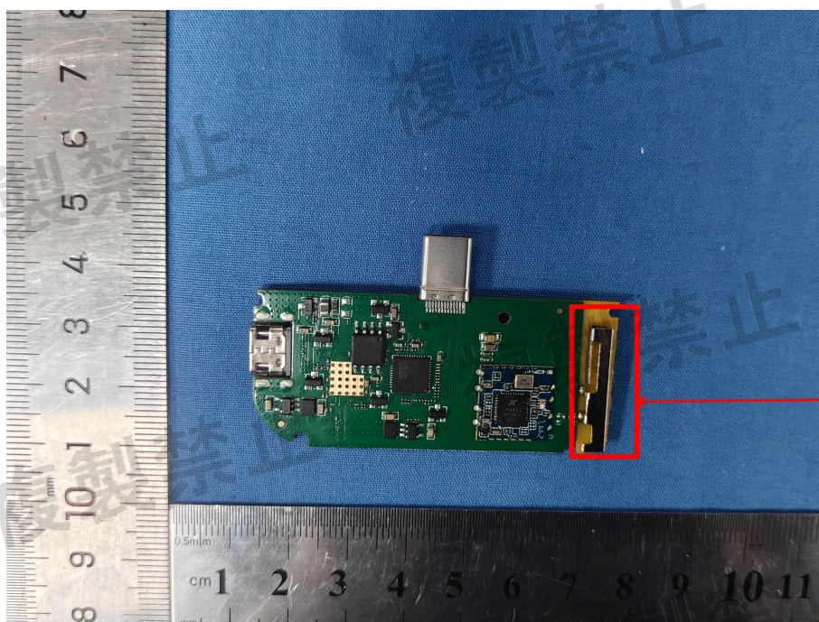
5.6GWIFI ANT: Integral antenna
