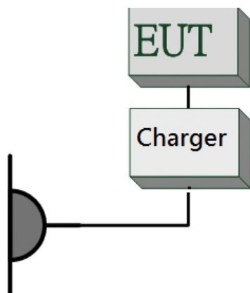
Radiated Emission & Conduction (AC Power Line)
