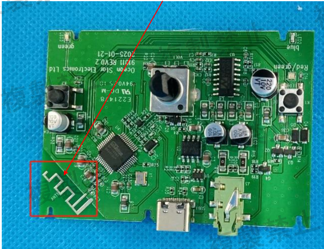
wireless antenna
