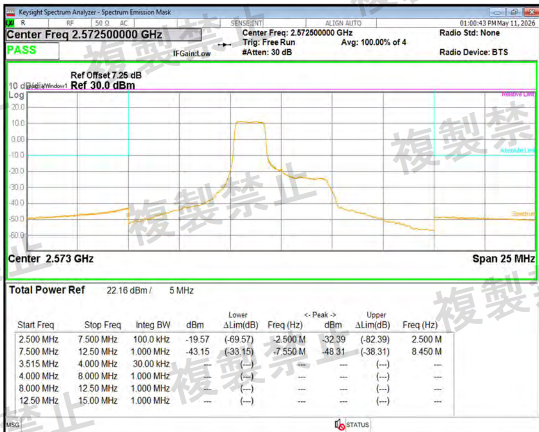
Band38(2570-2620) QPSK BW=5MHz Channel=37775 RB Size=8 Position=#Max
