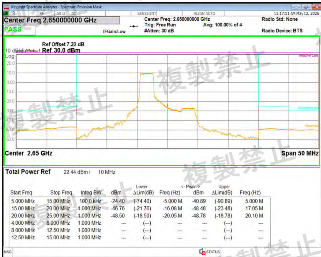
Band41(2555-2655) QPSK BW=10MHz Channel=41190 RB Size=12 Position=#Max
