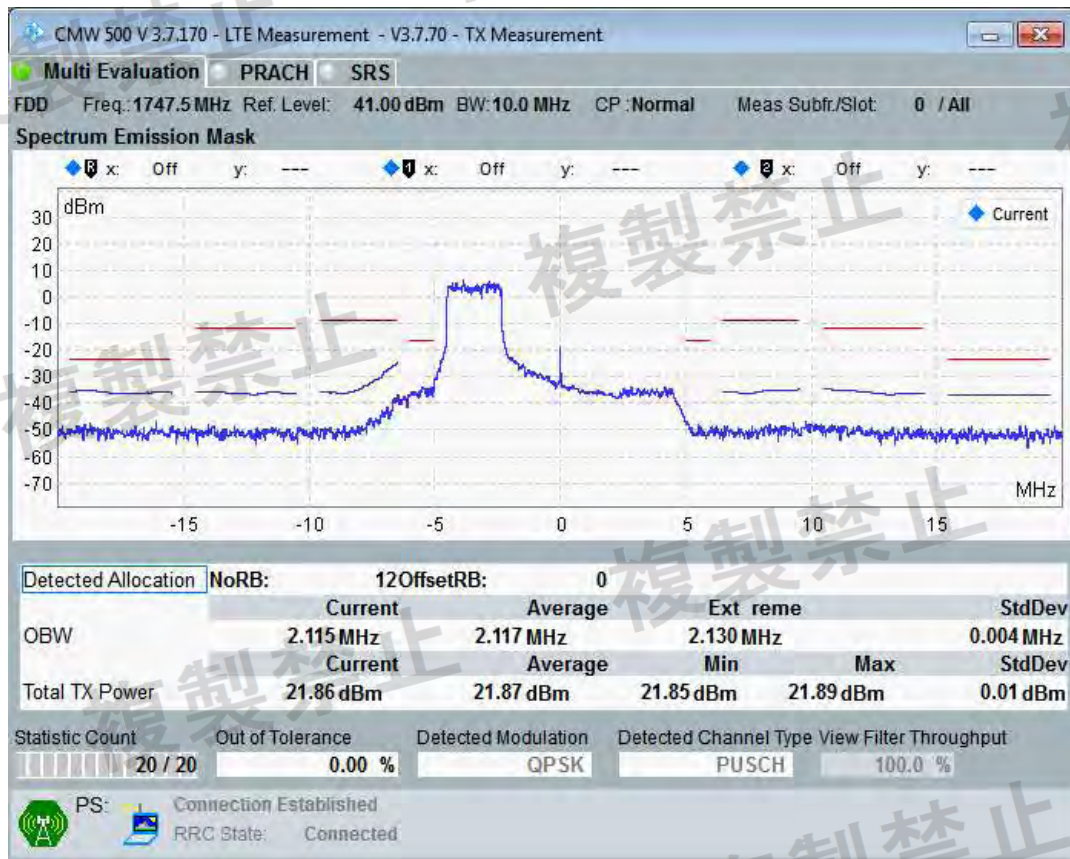
Band3(1710-1785) QPSK BW=10MHz Channel=19575 RB Size=12 Position=#Max
