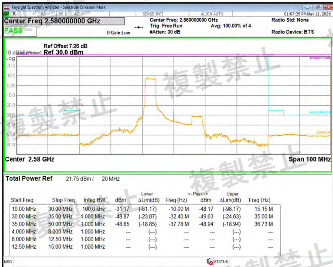
Band38(2570-2620) QPSK BW=20MHz Channel=37850 RB Size=18 Position=#Max
