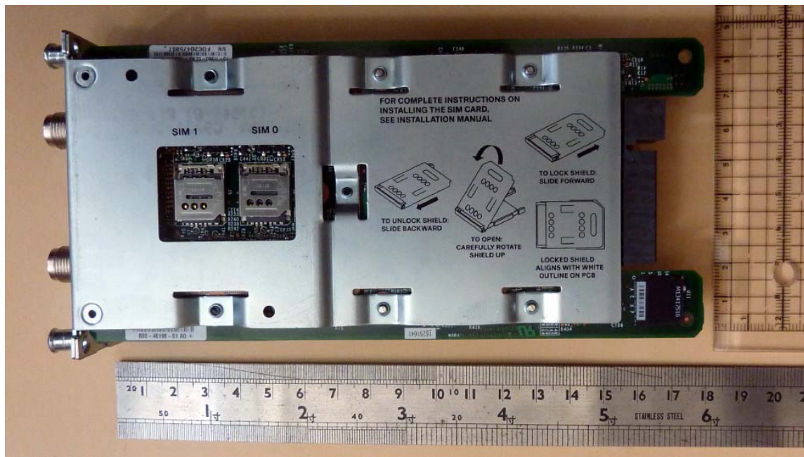
Bottom View
