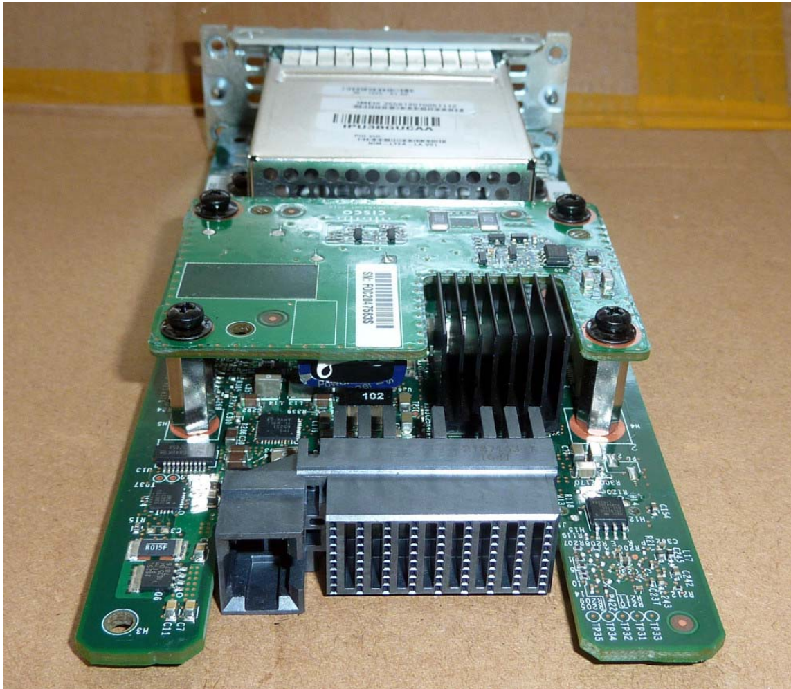
Rear View
