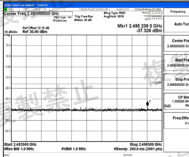
NTHV-DH5-Ant1-2441-2483.5~2496.5-PASS
