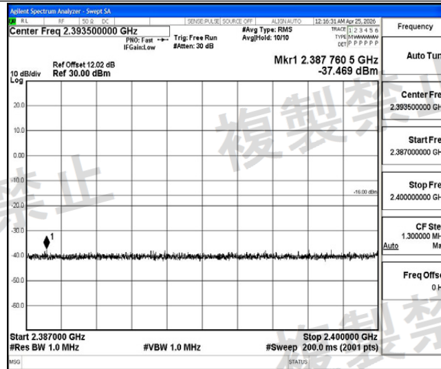
NTNV-3DH5-Ant1-2402-2387~2400-PASS
