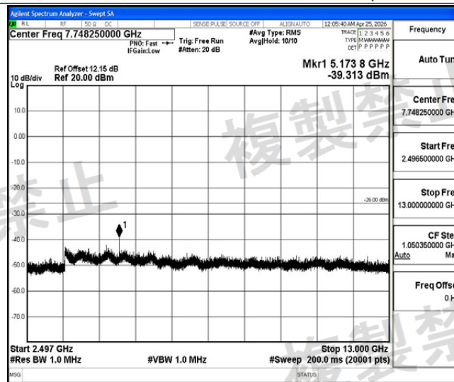
NTNV-DH5-Ant1-2441-2496.5~13000-PASS
