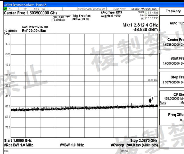
NTNV-3DH5-Ant1-2402-1000~2387-PASS
