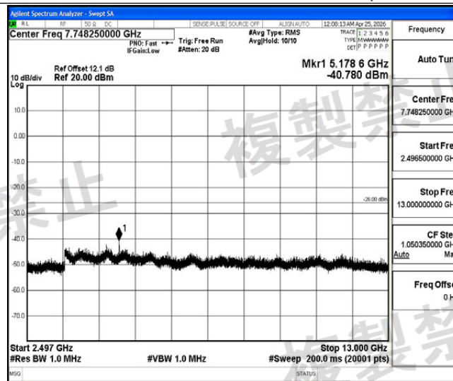
NTNV-DH5-Ant1-2480-2496.5~13000-PASS
