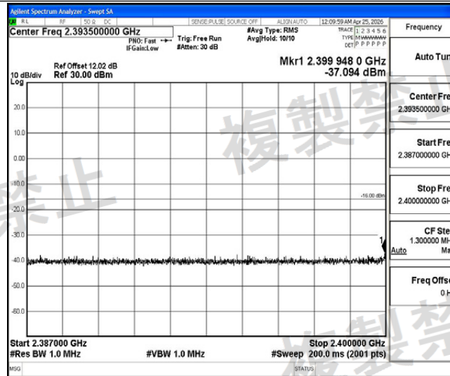
NTNV-2DH5-Ant1-2402-2387~2400-PASS
