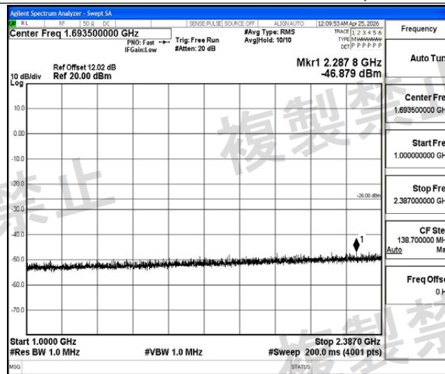
NTNV-2DH5-Ant1-2402-1000~2387-PASS
