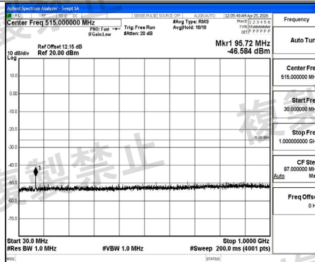
NTHV-DH5-Ant1-2441-30~1000-PASS
