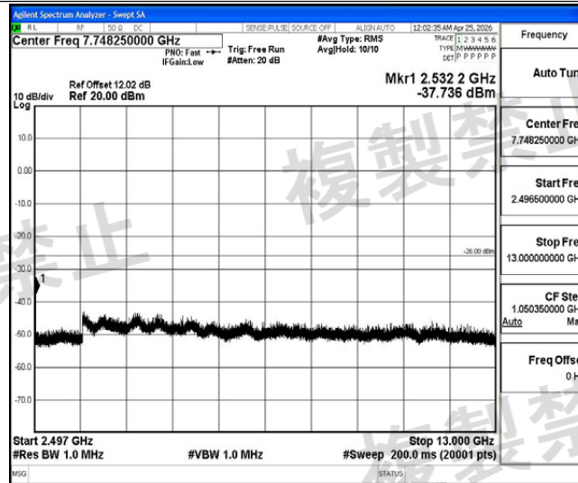
NTNV-DH5-Ant1-2402-2496.5~13000-PASS
