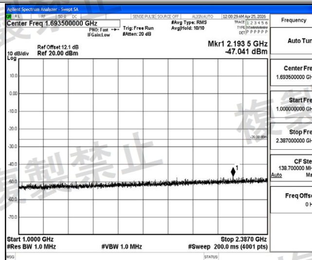
NTHV-DH5-Ant1-2480-1000~2387-PASS
