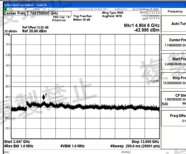
NTHV-3DH5-Ant1-2402-2496.5~13000-PASS
