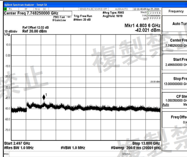
NTNV-3DH5-Ant1-2402-2496.5~13000-PASS
