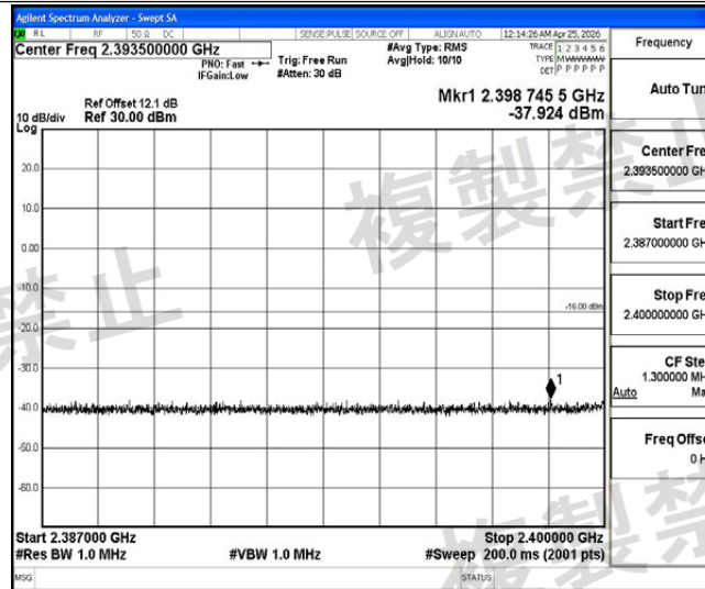
NTNV-2DH5-Ant1-2480-2387~2400-PASS
