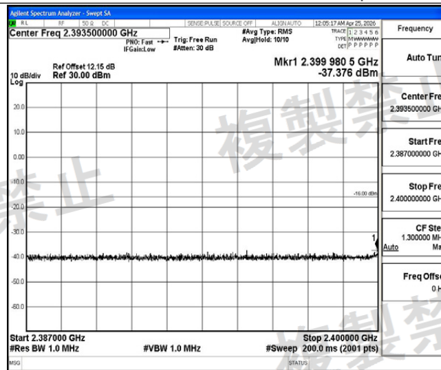
NTNV-DH5-Ant1-2441-2387~2400-PASS
