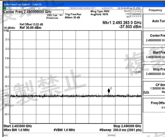
NTHV-2DH5-Ant1-2402-2483.5~2496.5-PASS
