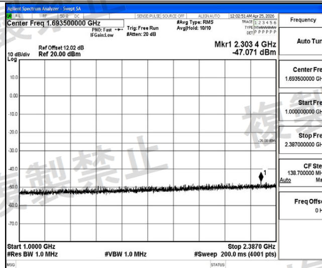
NTHV-DH5-Ant1-2402-1000~2387-PASS
