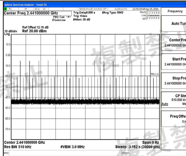
NTHV-3DH3-Ant1-Hop-PASS
