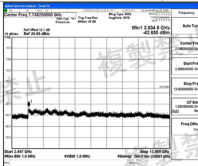
NTNV-2DH5-Ant1-2480-2496.5~13000-PASS
