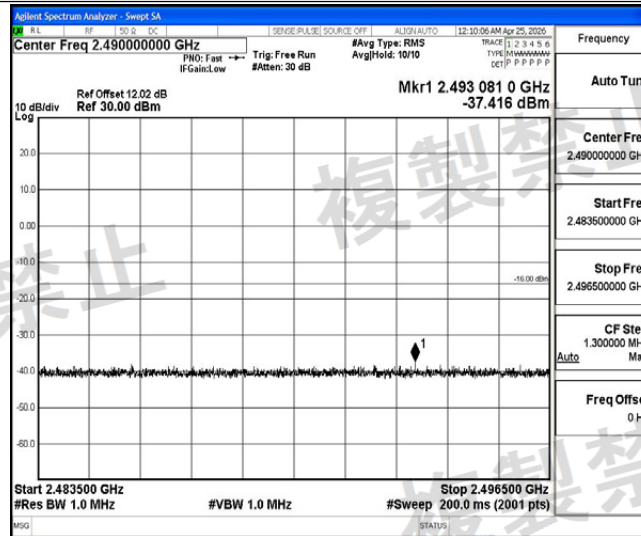
NTNV-2DH5-Ant1-2402-2483.5~2496.5-PASS
