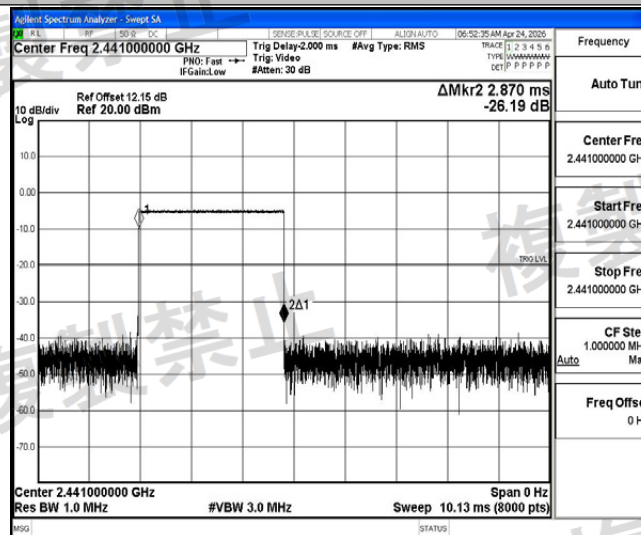
NTHV-DH5-Ant1-Hop-PASS
