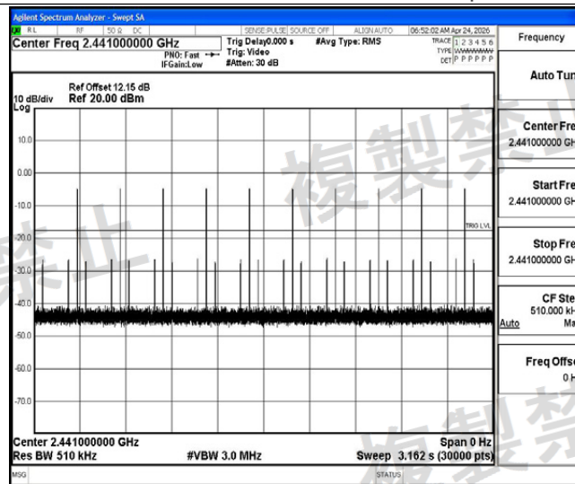
NTHV-DH5-Ant1-Hop-PASS
