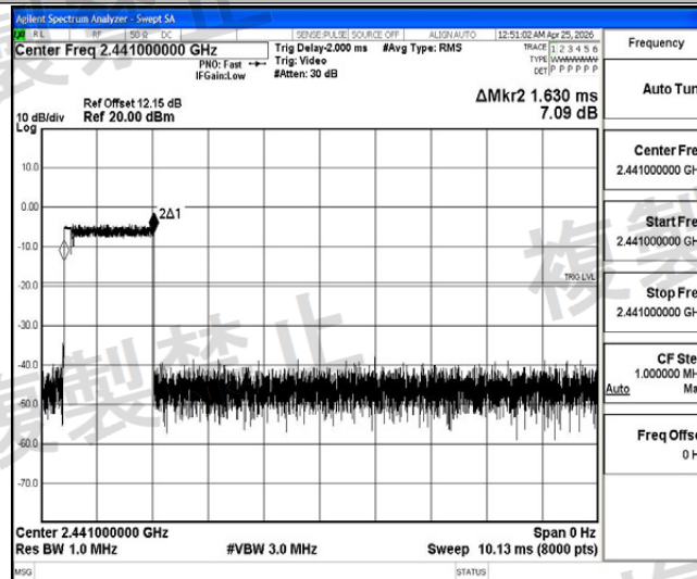
NTHV-3DH3-Ant1-Hop-PASS
