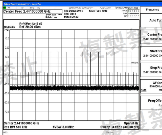
NTHV-DH3-Ant1-Hop-PASS
