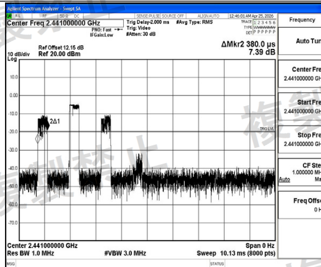
NTHV-3DH1-Ant1-Hop-PASS
