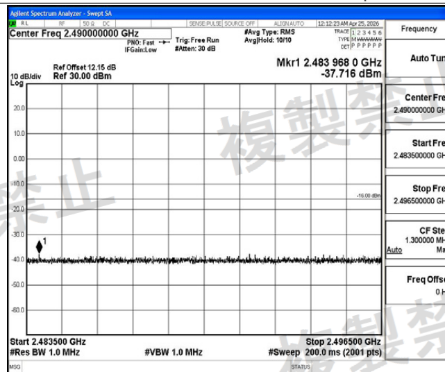
NTNV-2DH5-Ant1-2441-2483.5~2496.5-PASS
