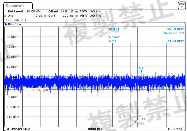
NTNV-11N40MIMO-Ant1-5190-30~1000-PASS
