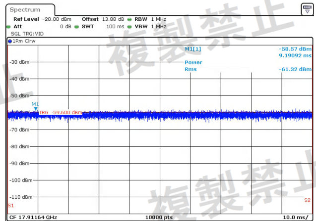
NTNV-11AC20MIMO-Ant2-5180-1000~26000-PASS
