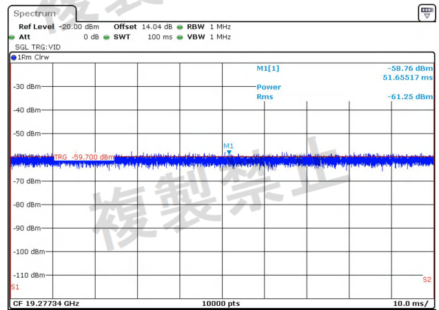
NTNV-11AC20-Ant2-5240-1000~26000-PASS
