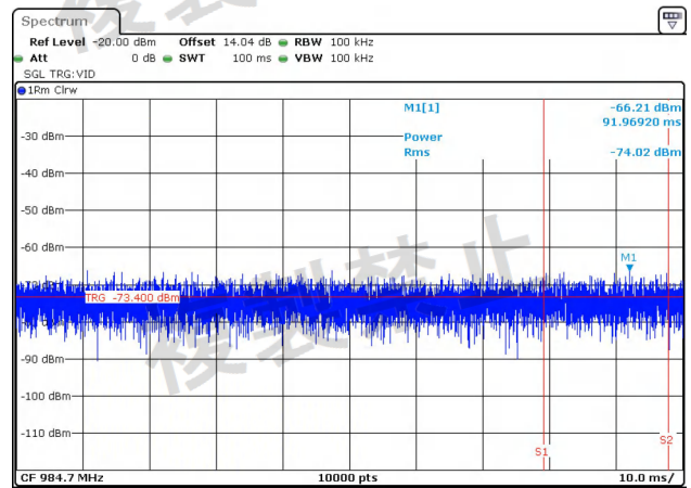
NTNV-11N40-Ant2-5230-30~1000-PASS
