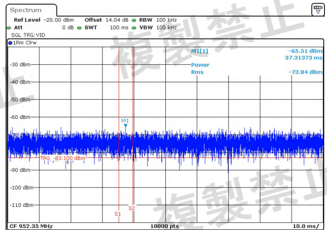
NTNV-11AC40-Ant2-5230-30~1000-PASS
