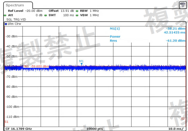
NTNV-11N40MIMO-Ant2-5190-1000~26000-PASS
