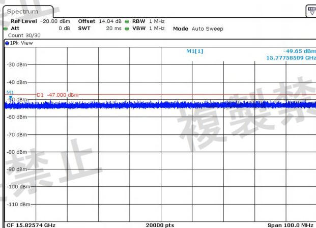
NTNV-11N40MIMO-Ant2-5230-1000~26000-PASS
