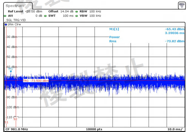
NTNV-11N40MIMO-Ant2-5230-30~1000-PASS
