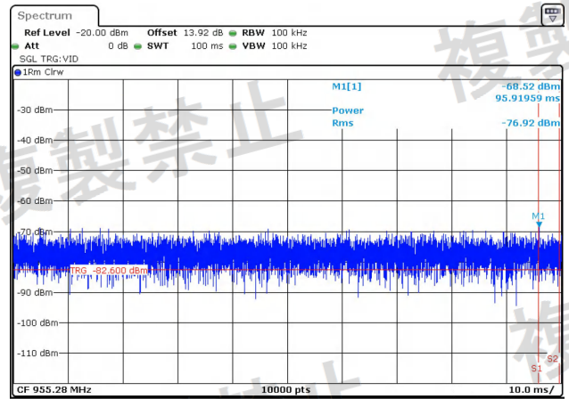
NTNV-11AC20MIMO-Ant1-5200-30~1000-PASS
