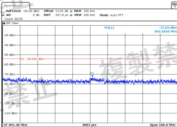
NTNV-11N40MIMO-Ant1-5190-30~1000-PASS
