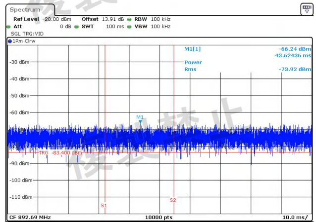
NTNV-11N40MIMO-Ant2-5190-30~1000-PASS
