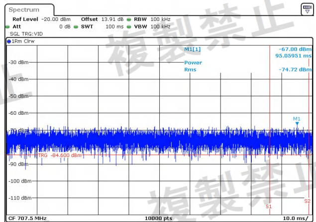
NTNV-11AC20MIMO-Ant1-5180-30~1000-PASS
