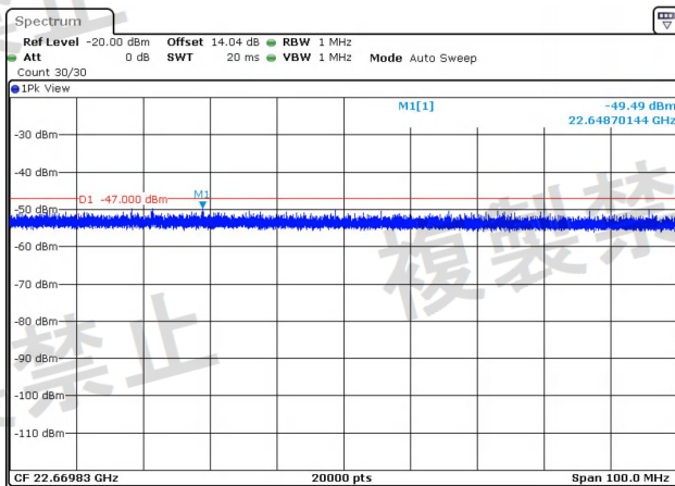
NTNV-11AC20-Ant2-5240-1000~26000-PASS
