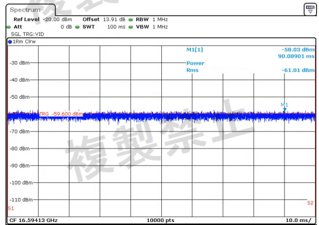
NTNV-11AC20MIMO-Ant2-5180-1000~26000-PASS
