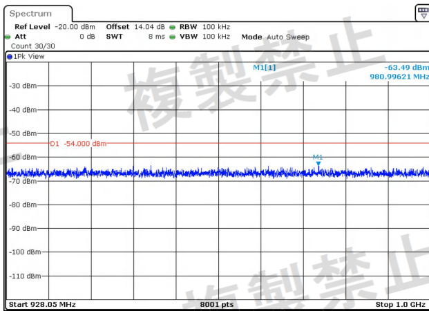
NTNV-11N40MIMO-Ant2-5230-30~1000-PASS
