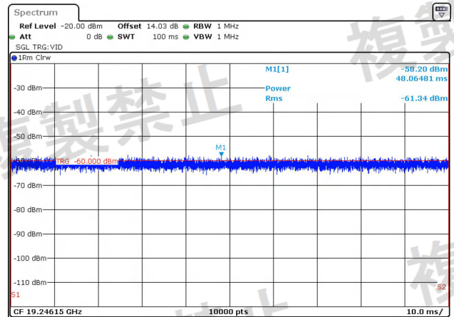
NTNV-11AC20MIMO-Ant2-5200-1000~26000-PASS
