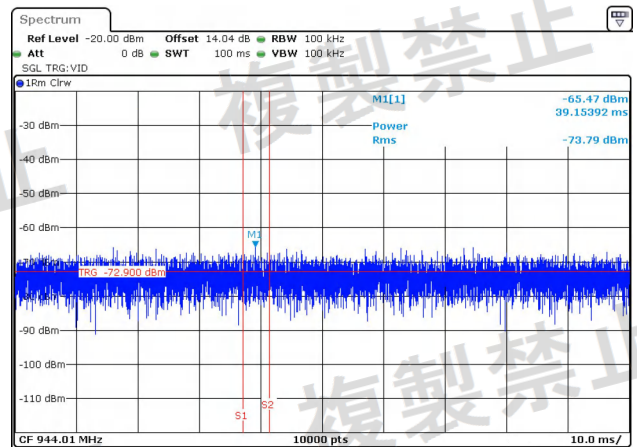
NTNV-11N40MIMO-Ant2-5230-30~1000-PASS
