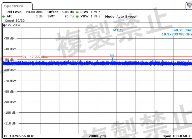
NTNV-11AC20-Ant2-5240-1000~26000-PASS
