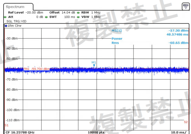
NTNV-11N40MIMO-Ant1-5230-1000~26000-PASS
