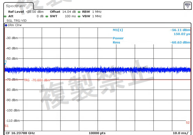
NTNV-11N40MIMO-Ant2-5230-1000~26000-PASS
