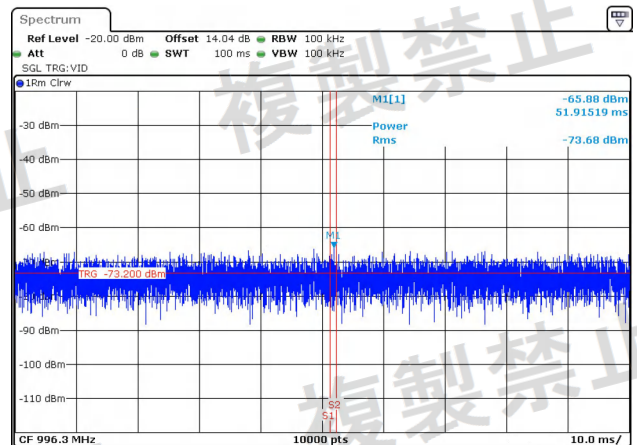
NTNV-11AC20-Ant1-5240-30~1000-PASS
