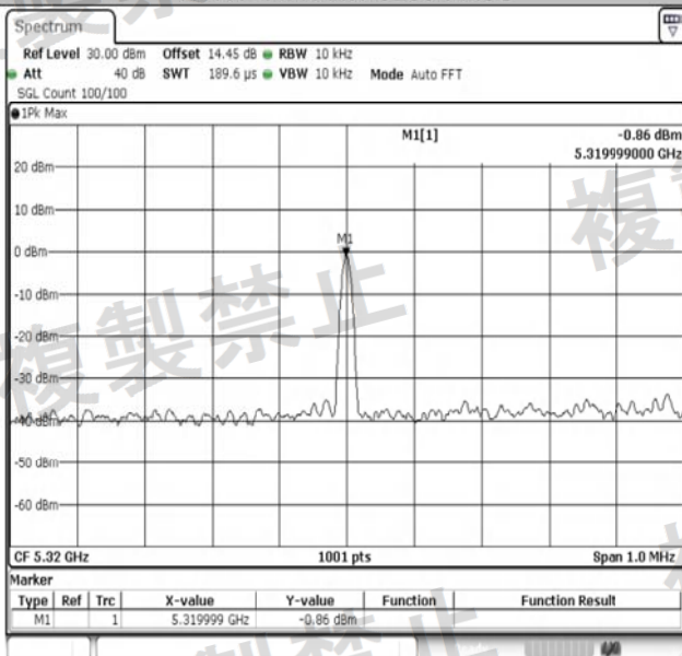
NTNV-11A-Ant1-5320-PASS
