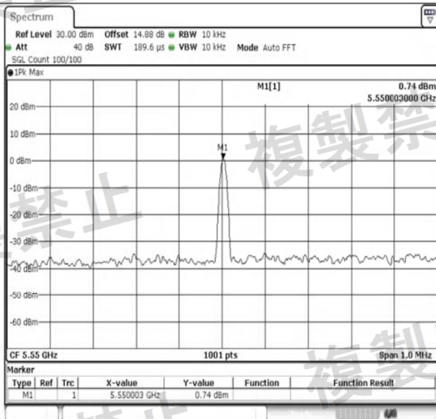
NTNV-11N40SISO-Ant1-5550-PASS
