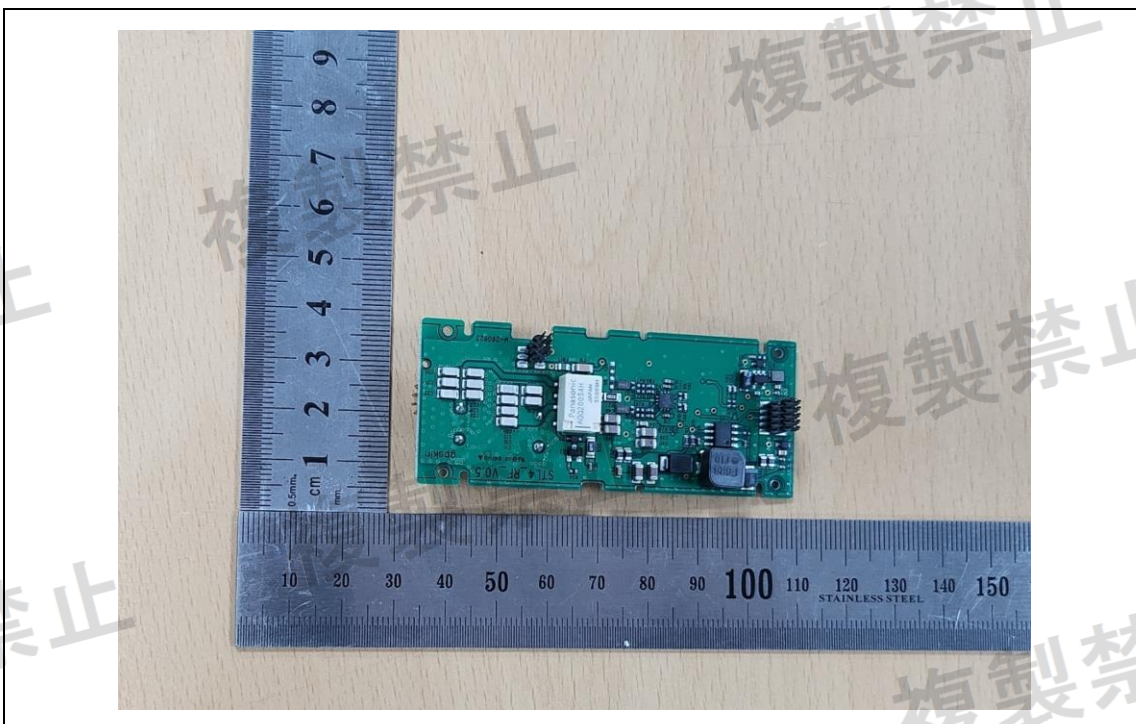
Board 2 Rear
