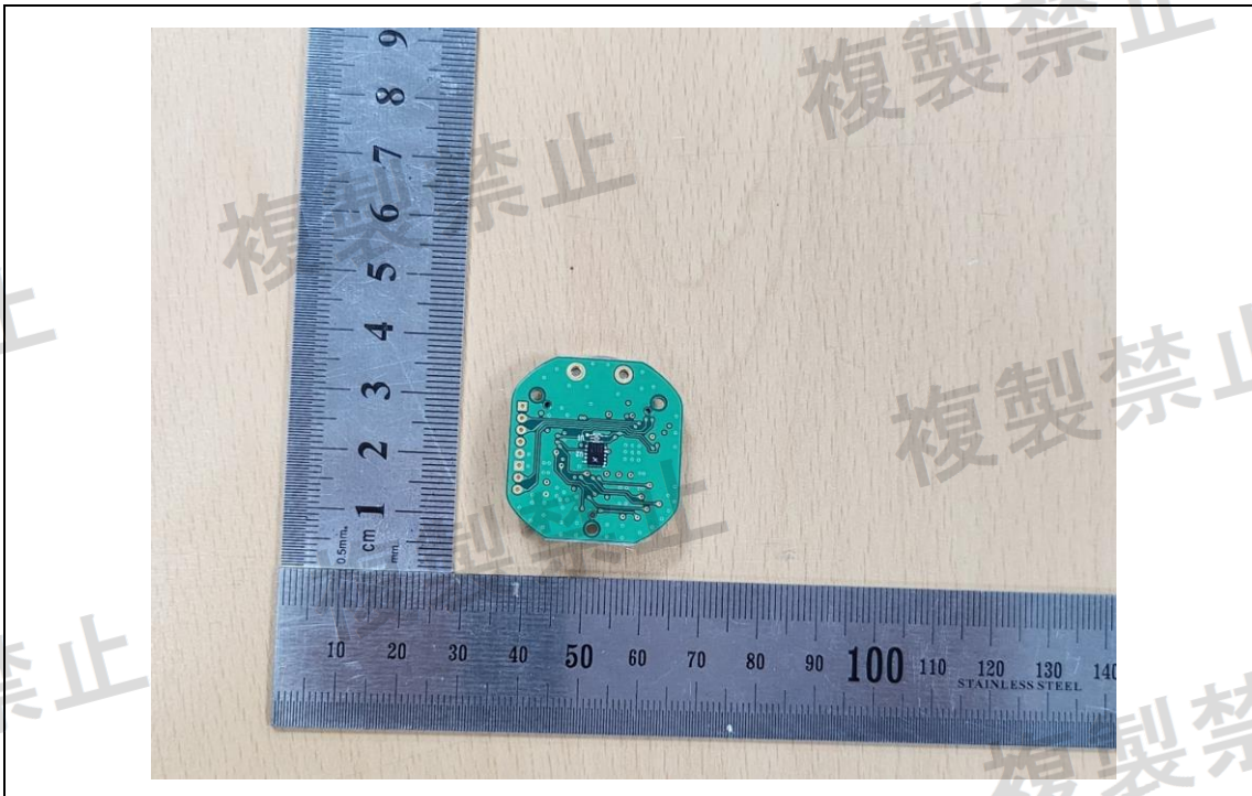
Board 4 Rear
