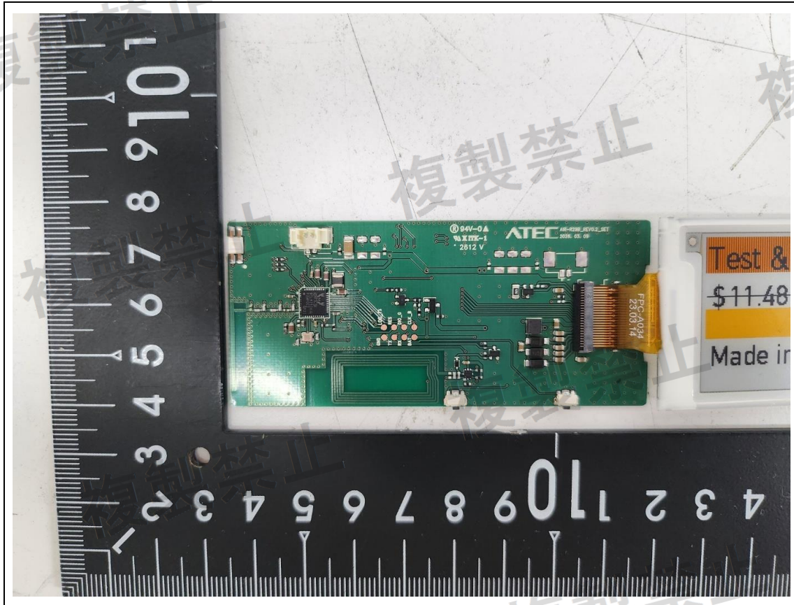
Board 1 Front
